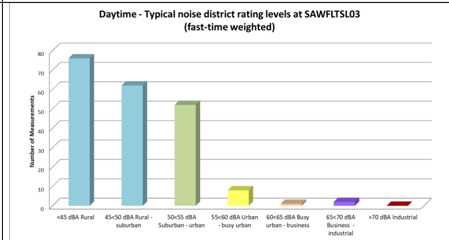
Figure 4-15: Classification of daytime measurements in typical noise districts at SAWFLTSL03
