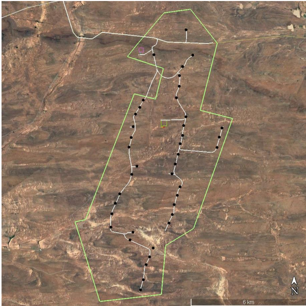
Figure 2. Satellite image showing the layout of the proposed Aberdeen Wind Facility 2, with turbine locations, turbine access roads, substation, battery storage area and laydown area.
