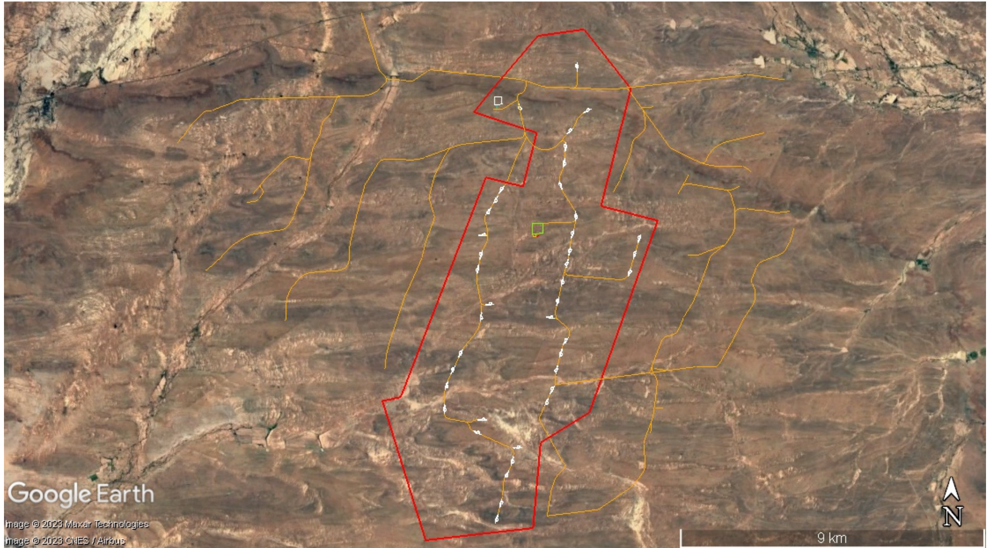
Figure 2 The currently planned infrastructure layout of the proposed Aberdeen Wind Facility 2
