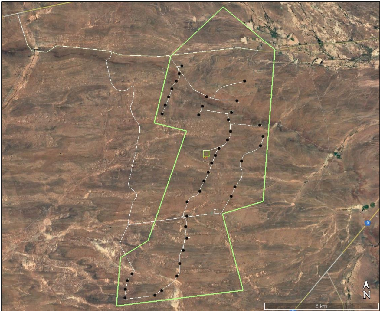
Figure 1. Satellite image showing the location and layout of the proposed Aberdeen Wind Facility 3, with turbine locations, turbine access roads, substation, battery storage area and laydown area.
