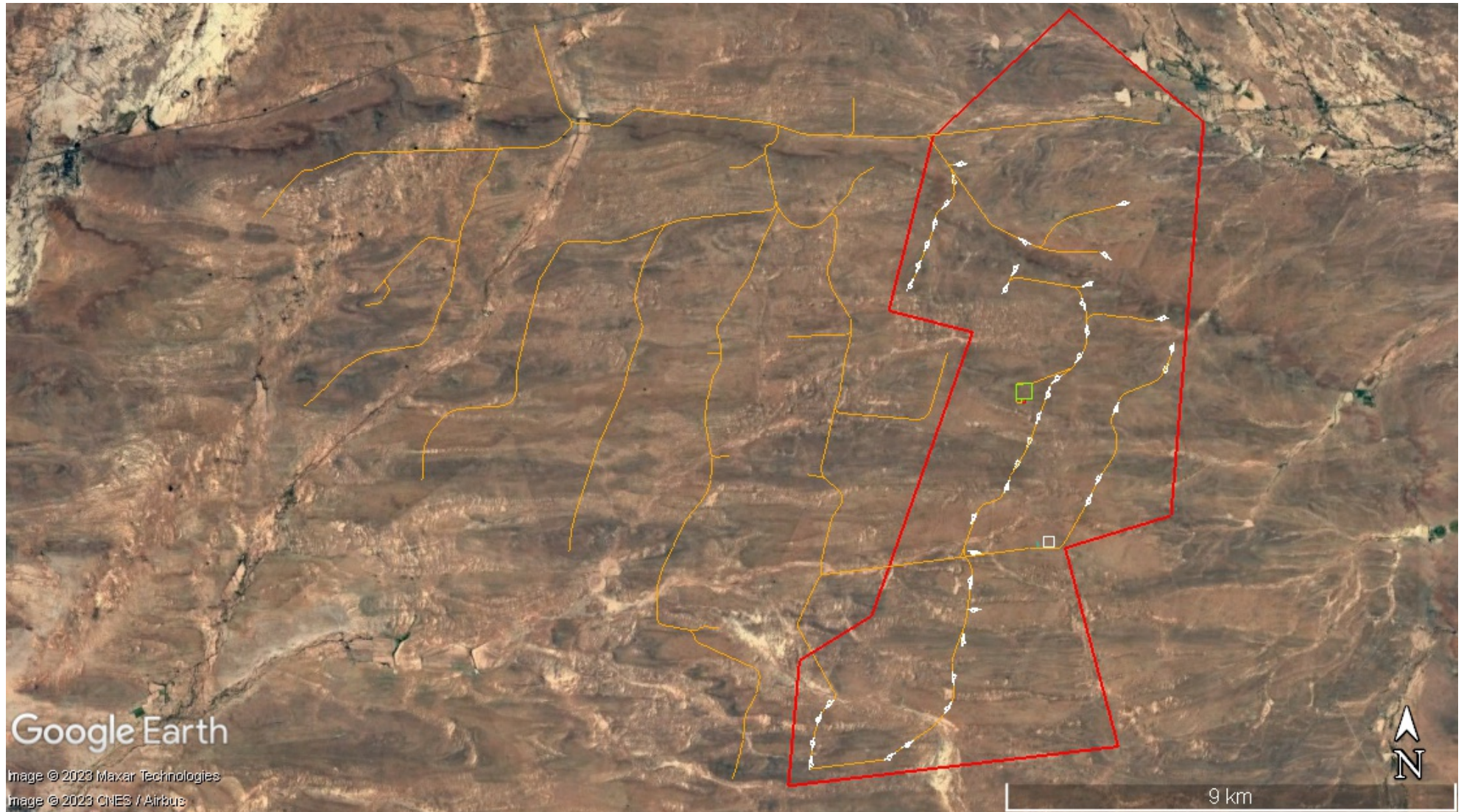
Figure 2 The currently planned infrastructure layout of the proposed Aberdeen Wind Facility 3
