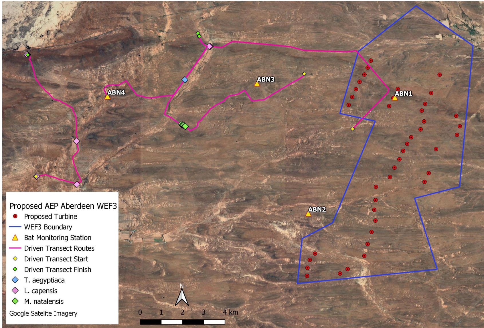
Figure 16 Driven transect routes in the study area, showing the locations and species identity of recorded bat calls
