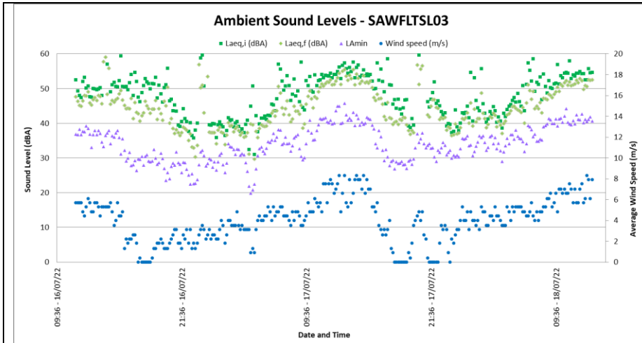
Figure 4-12: Ambient Sound Levels at SAWFLTSL03
