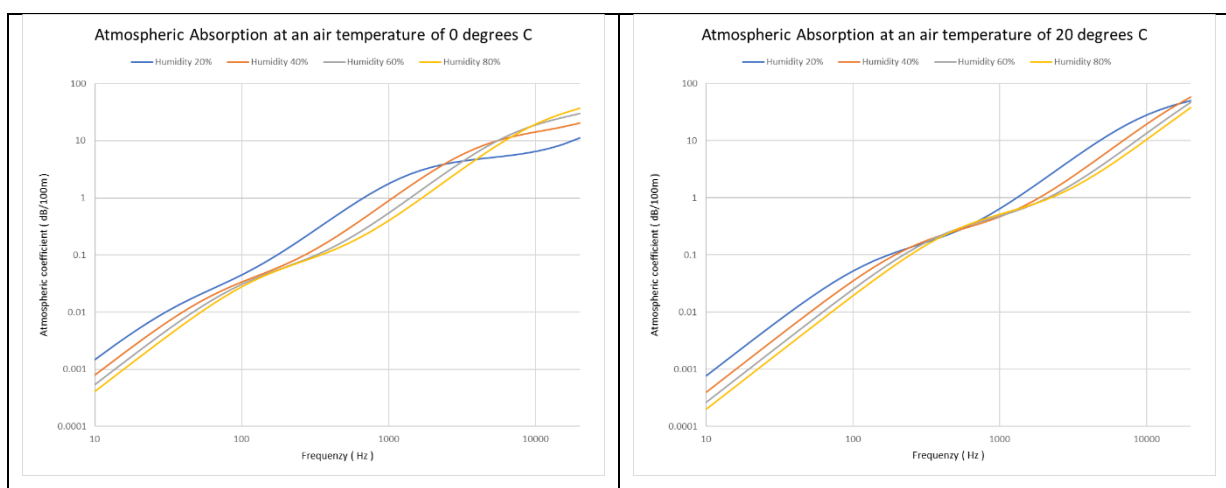
Figure 4-1: Effect of Temperature and Humidity on propagation of Sound
