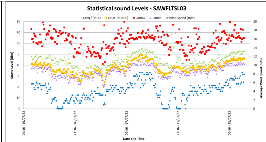
Figure 4-13: Maximum, minimum and Statistical sound levels at SAWFLTSL03
