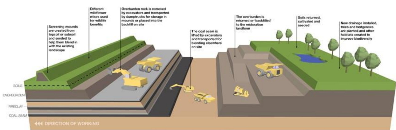
Figure 14: Illustration of a typical opencast rollover mining operation
