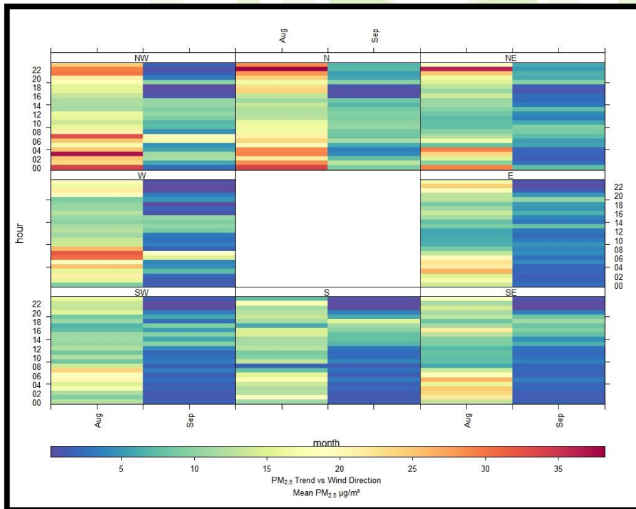
Figure 17: Trend Analysis showing trends in higher emissions at specific hours and wind direction.
