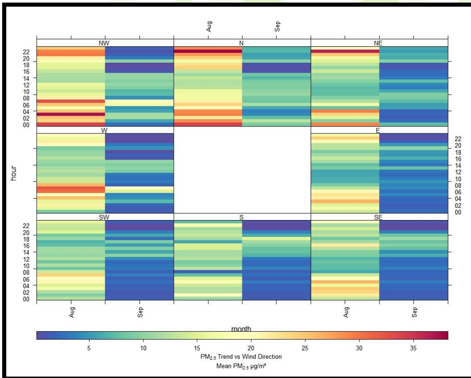
Figure 32: Trend Analysis showing trends in higher emissions at specific hours and wind direction.
