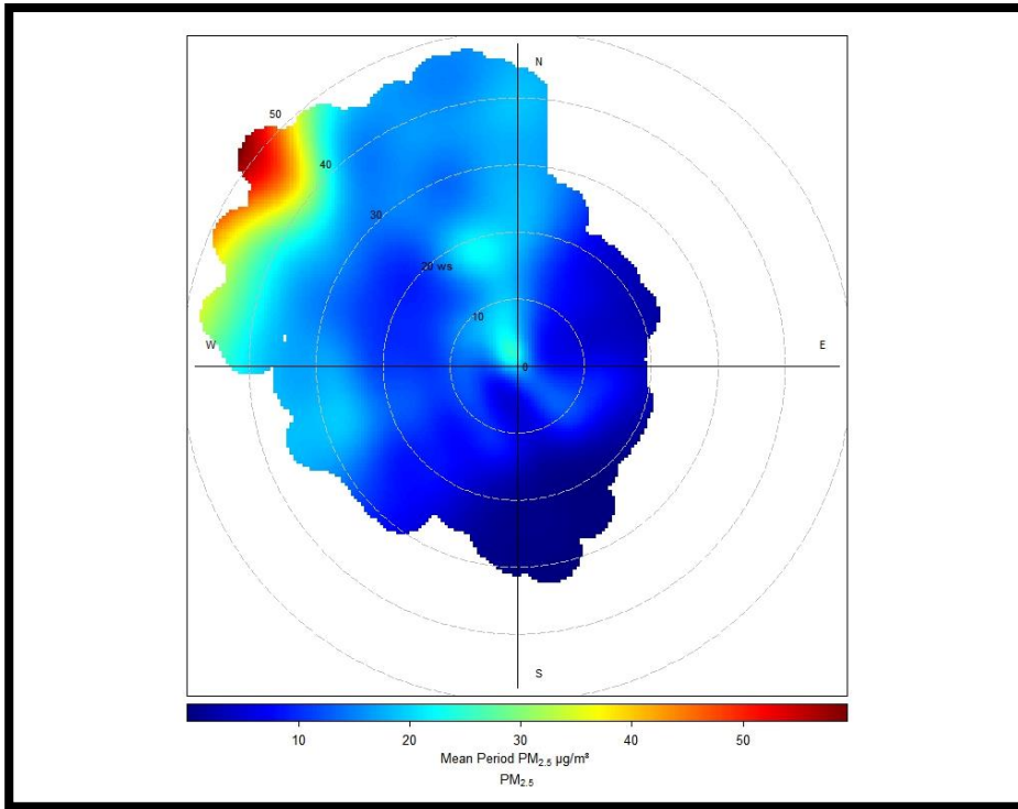
Figure 18: Polar Plot indicating higher emissions at higher windspeeds from the north-west.
