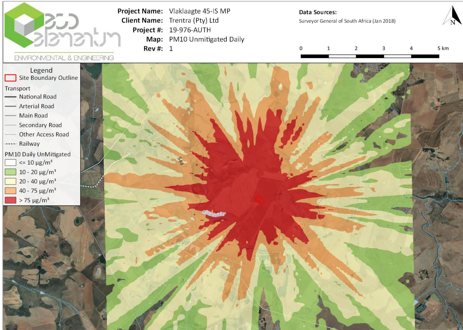
Figure 24: Predicted 2 nd Highest daily concentrations for PM10 for the proposed project operations when unmitigated.
