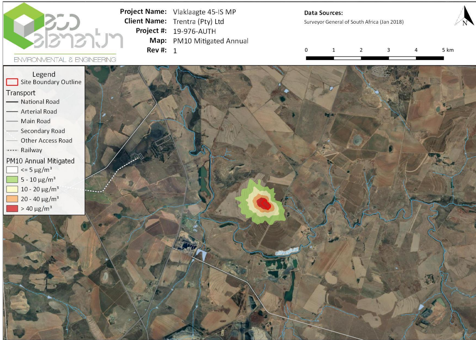
Figure 23: Predicted average annual concentrations for PM10 for the proposed Vlaklaagte project operations when mitigated.
