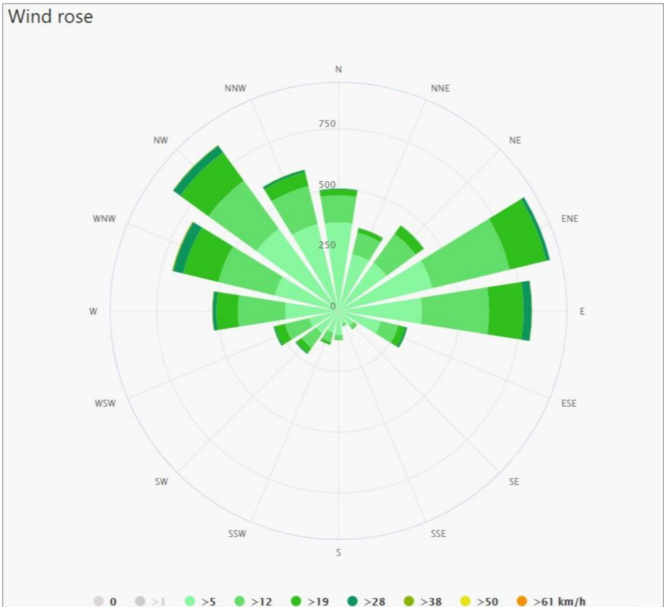
Figure 9: NEMS 30 km simulation model wind rose for the proposed Vlaklaagte project area for the period 1985 to current.
