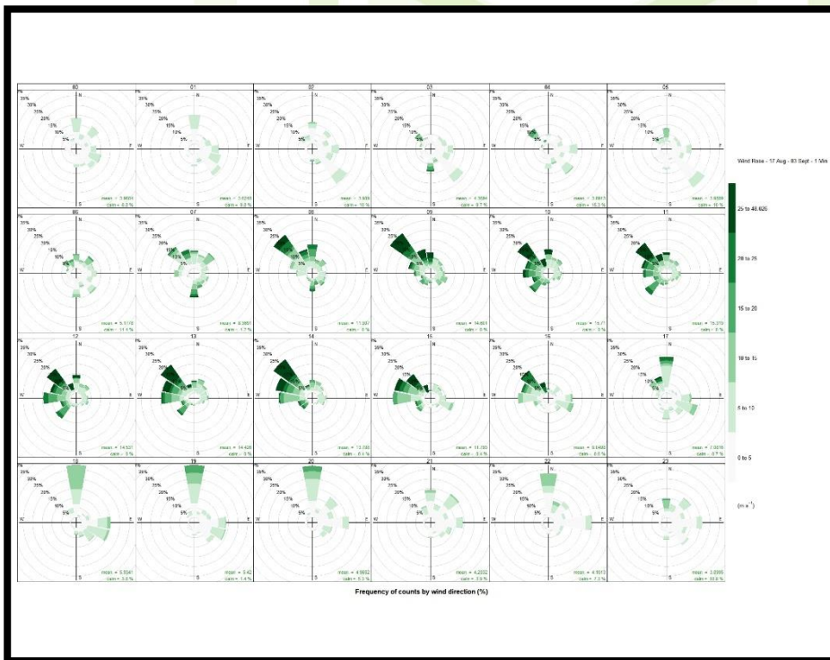
Figure 34: Hourly average wind roses to assist in decision making.
