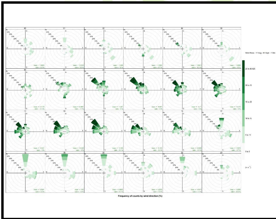
Figure 19: Hourly average wind roses to assist in decision making.
