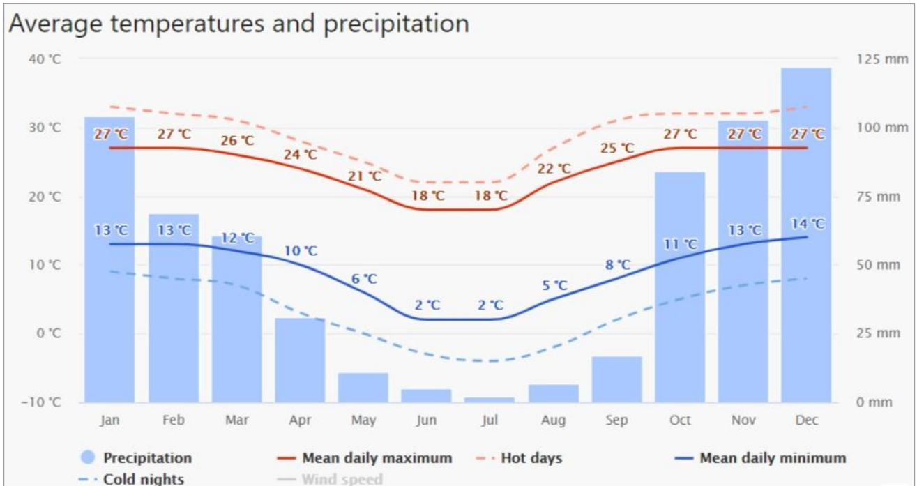
Figure 10: Temp and precipitation simulation results from the NEMS model for the Vlaklaagte project area (1985 - current).
