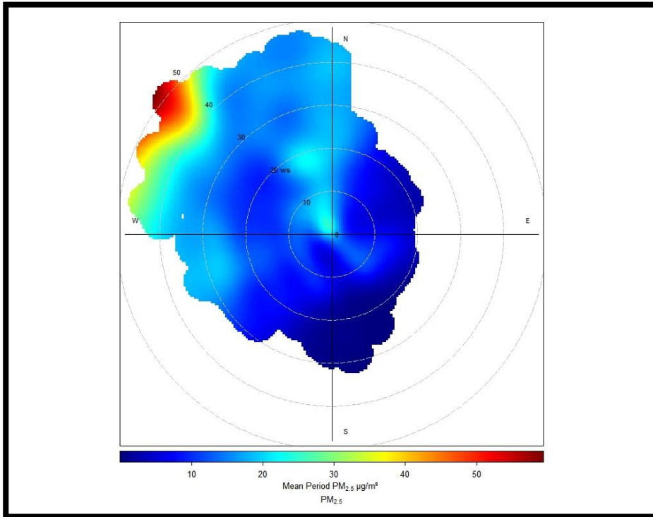
Figure 33: Polar Plot indicating higher emissions at higher windspeeds from the north-west.
