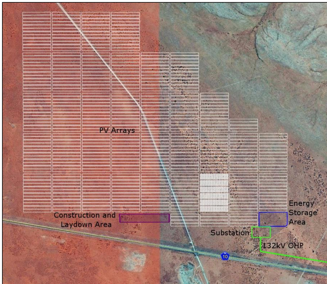
Figure 1: Proposed Allepad PV One layout.
