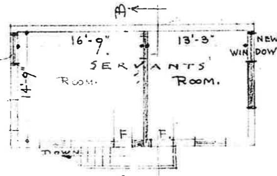
FIRST-FLOOR-PLAN.
