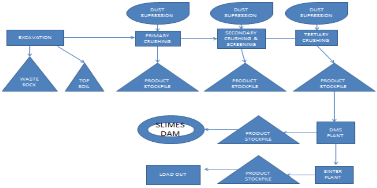
Figure 3: Schematic representation of the planned process flow for manganese and Iron ore.
