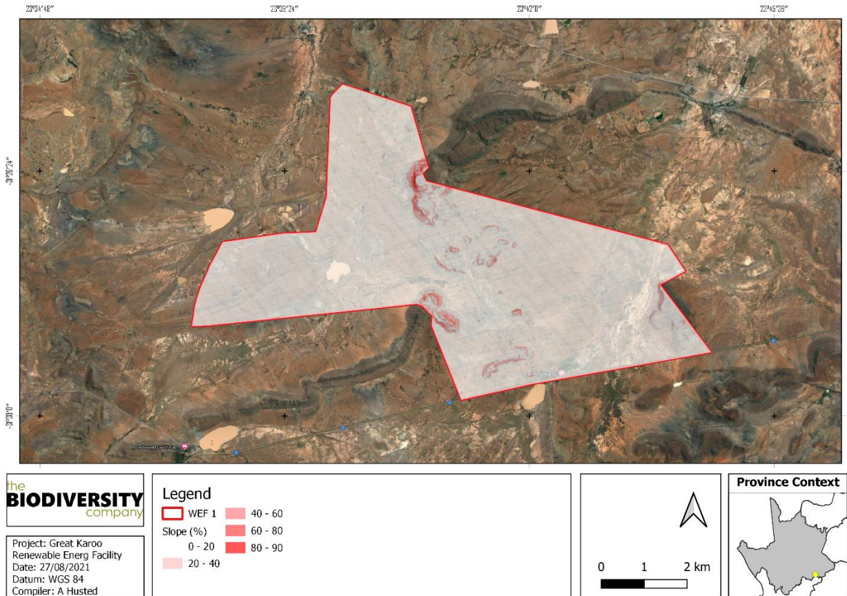
Figure 2-14 The slope percentage calculated for the project area
