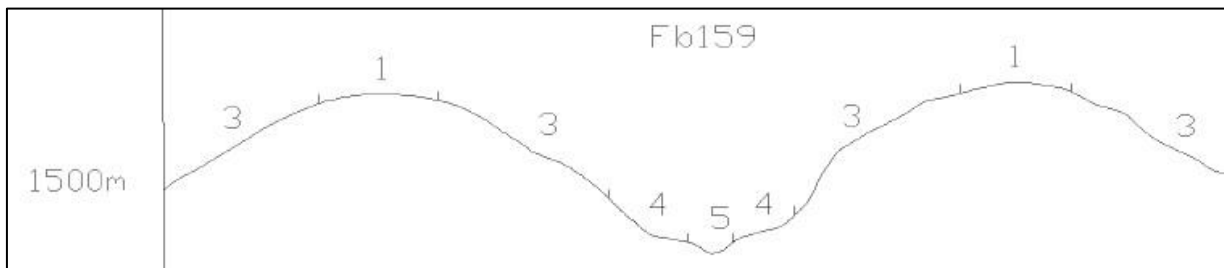
Figure 2-12 Illustration of land type Fb 159 terrain unit (Land Type Survey Staff, 1972 - 2006)
