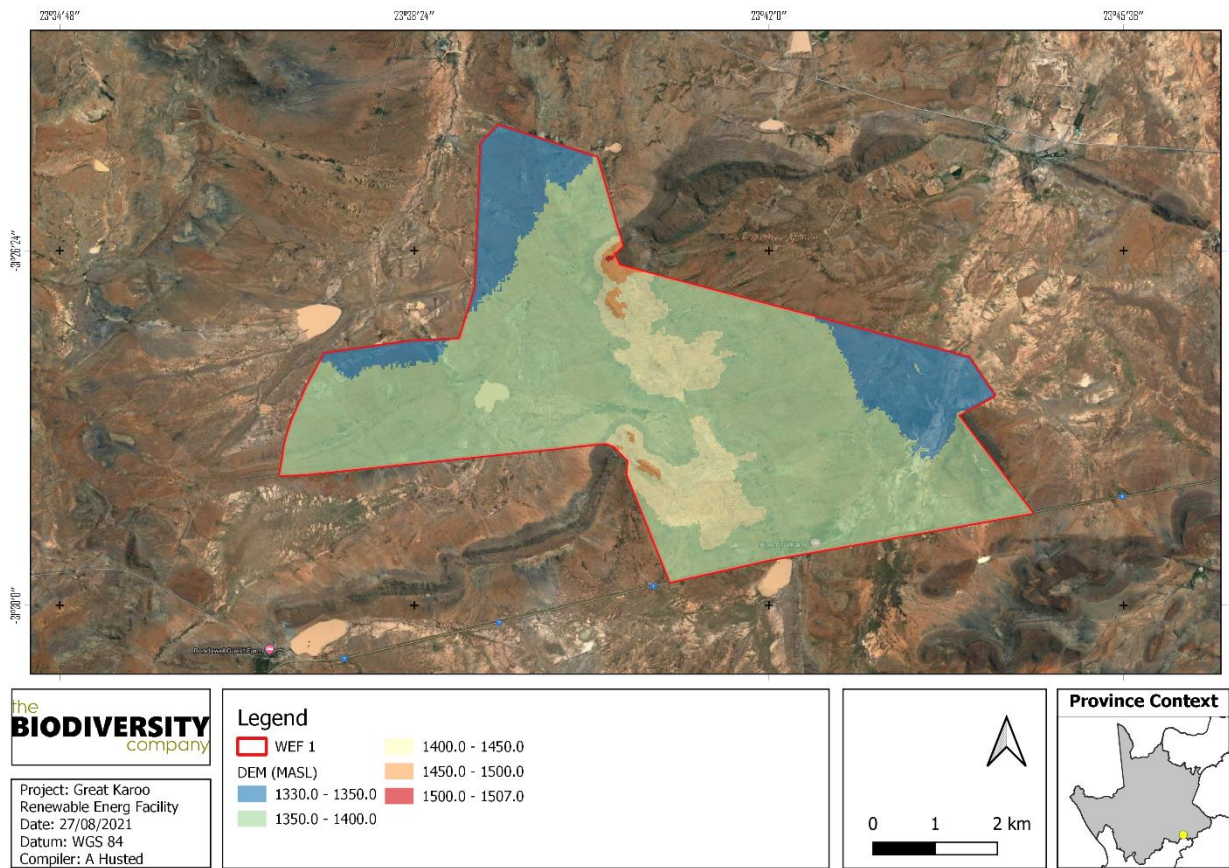
Figure 2-15 The DEM generated for the project area
