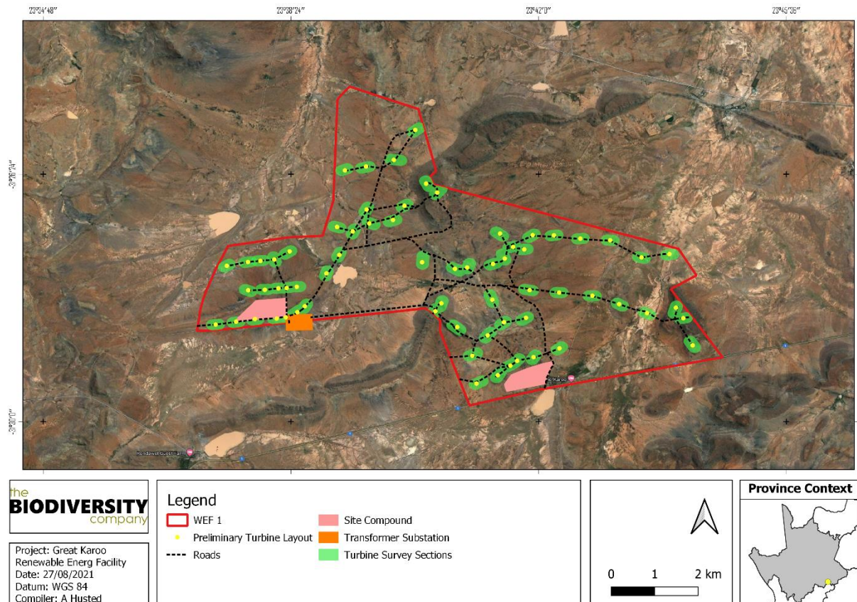
Figure 4-1 Preliminary layout for the proposed facility
