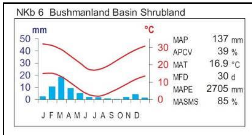
Figure 7. Climate diagram for Bushmanland Basin Shrubland (from Mucina et al. , 2006) showing MAP – Mean Annual Precipitation; APCV = Annual Precipitation Coefficient of Variance; MAT = Mean Annual Temperature; MFD = Mean Frost Days; MAPE = Mean Annual Potential Evaporation; MASMA = Mean Annual Soil Moisture Stress
