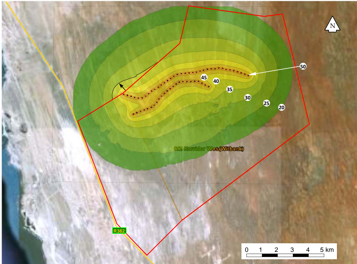
FIGURE 5.1 Richtersveld proposed wind farm with site boundaries demarcated by red lines; wind turbine locations shown in red; and calculated L_{Aeq} contours due to noise from the wind turbines.
