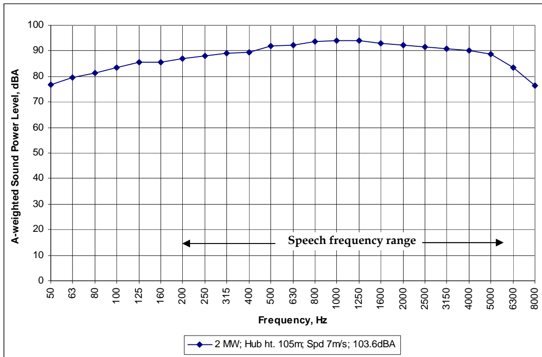
Figure 4.1 A-weighted sound power level spectra of 2 MW wind energy turbine with hub height of 105 m used in this study operating in a wind speed of 7 m/s.
