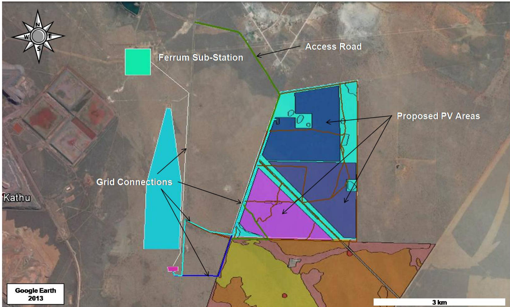
Figure 2. Provisional development layout on the affected properties showing PV Areas (solar panels), access road and grid connection routes.
