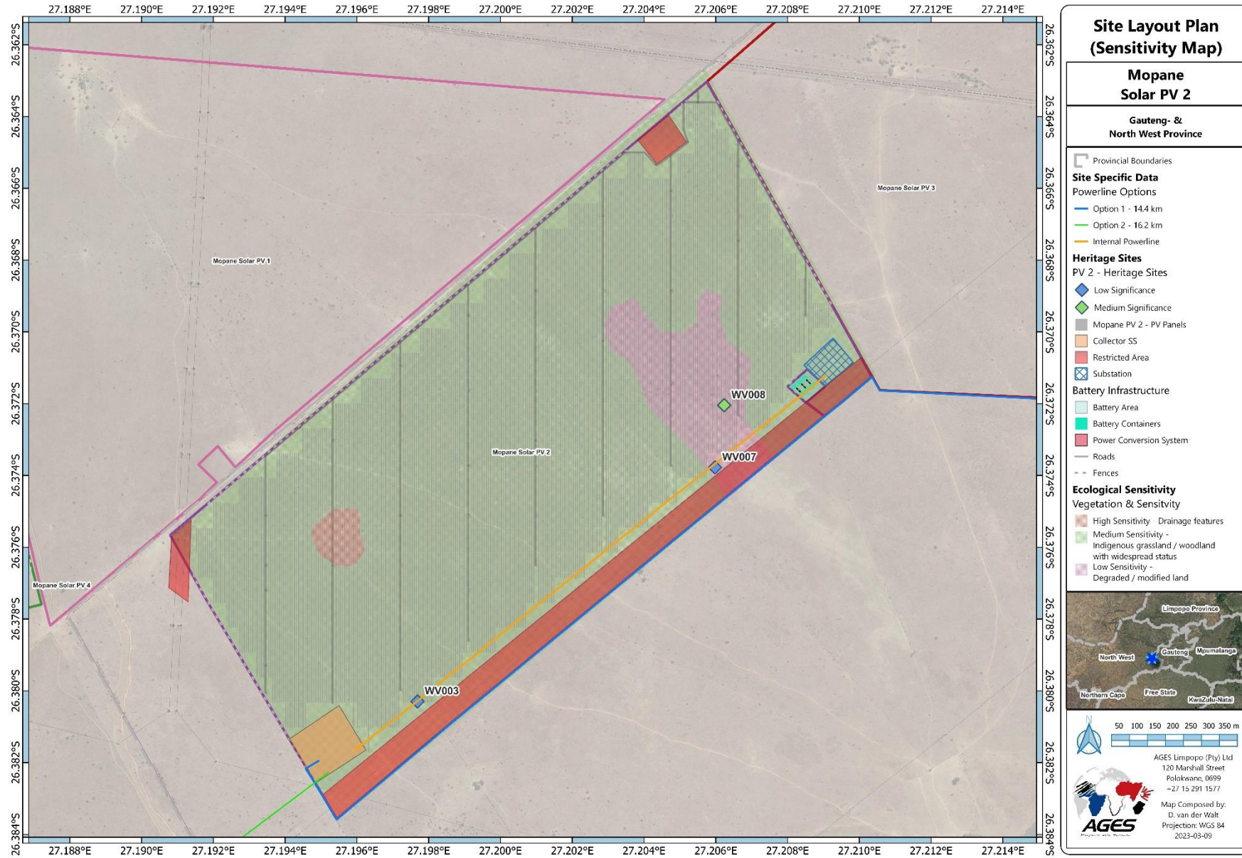
Figure 4. Aerial view and proposed draft layout of the project
