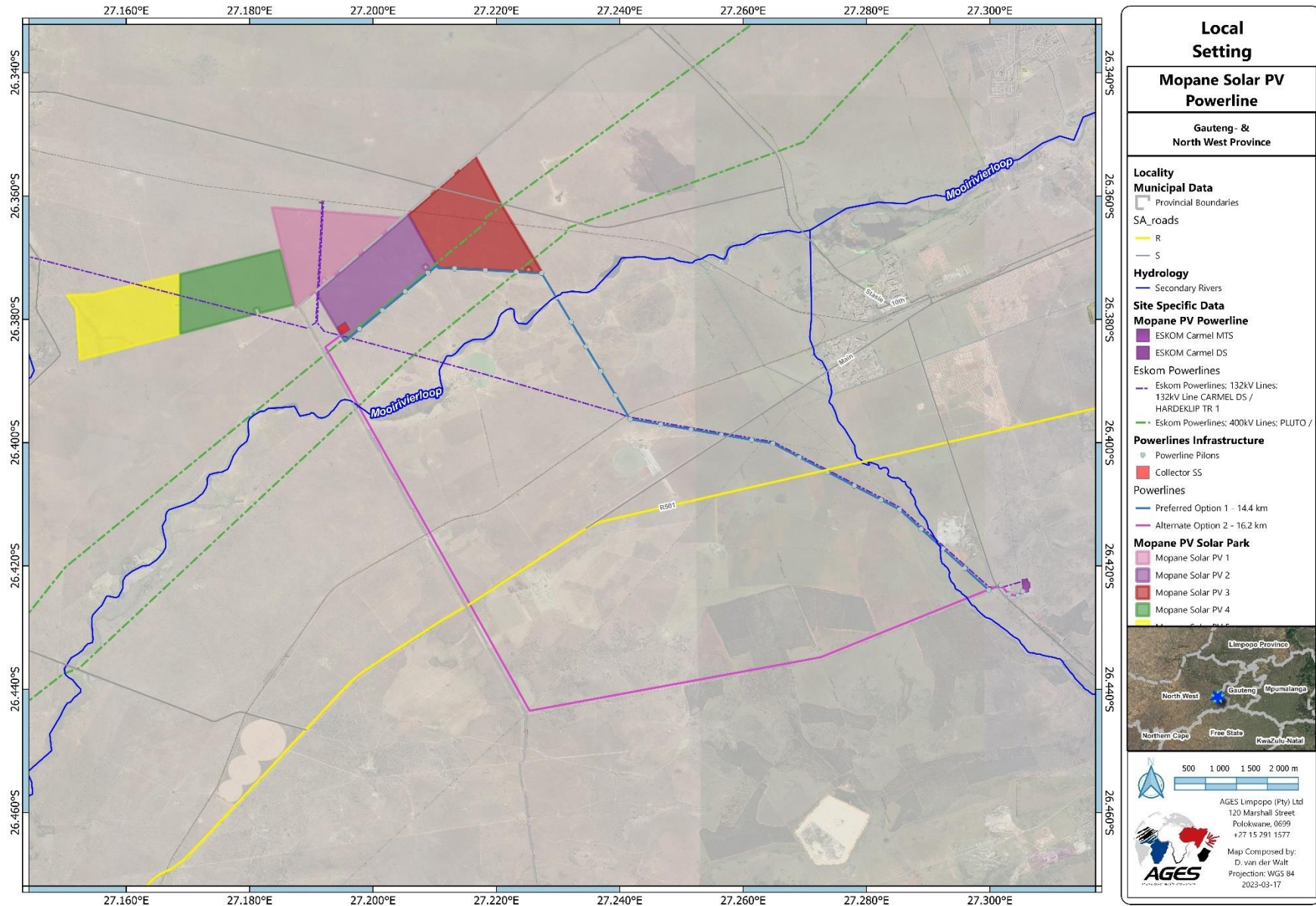
Figure 1. Regional location map of the Mopane 1 - 5 PV Solar Parks cluster
