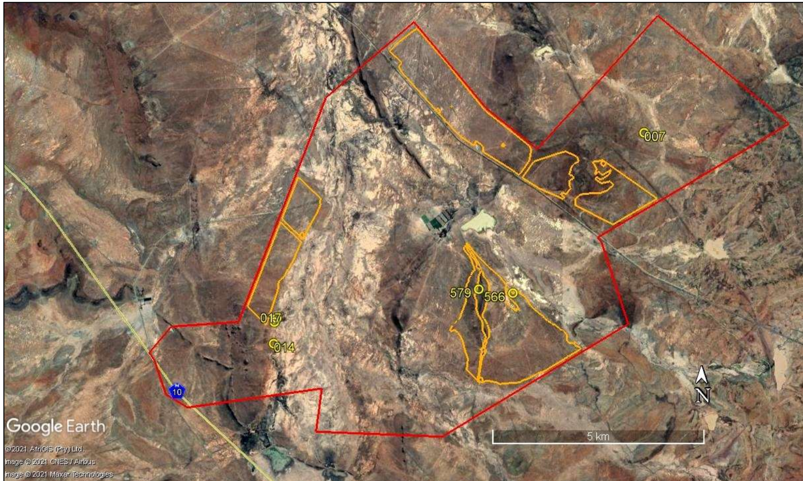
Figure 44: Google Earth© satellite image of the Soventix 300 MW solar plant project areas near Hanover (yellow polygons) showing numbered new fossil localities: 007 – questionable invertebrate burrows in koffieklip . 014, 017, 020 – locally common blocks of reworked Permian petrified wood eroding out of consolidated older alluvium along the Brakrivier. 566 – poorly-preserved bone fragments (possibly dinocephalian) in surface float (No mitigation recommended). 579 – fragmentary remains (including partial jaws and teeth) of a tapinocephalid dinocephalian – N.B. this site lies just outside the project area (No mitigation necessary). See Appendix 1 for GPS locality details.
