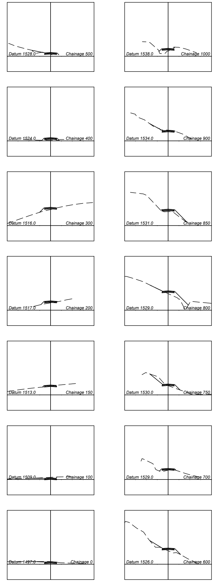
ROAD 4 Horizontal Scale 1:1000 Vertical Scale 1:500
