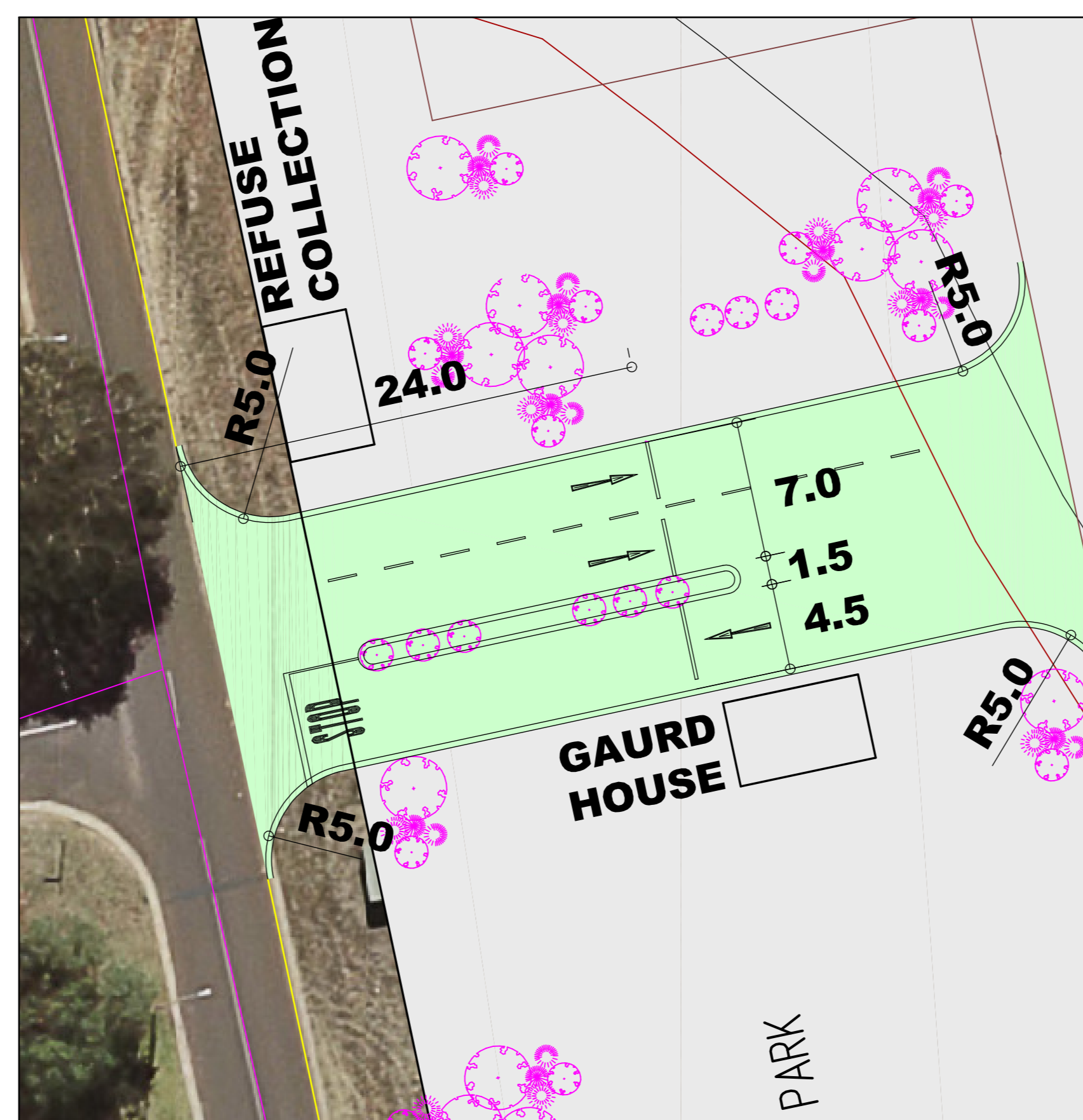
INSERT: ACCESS DETAIL SCALE 1:250
