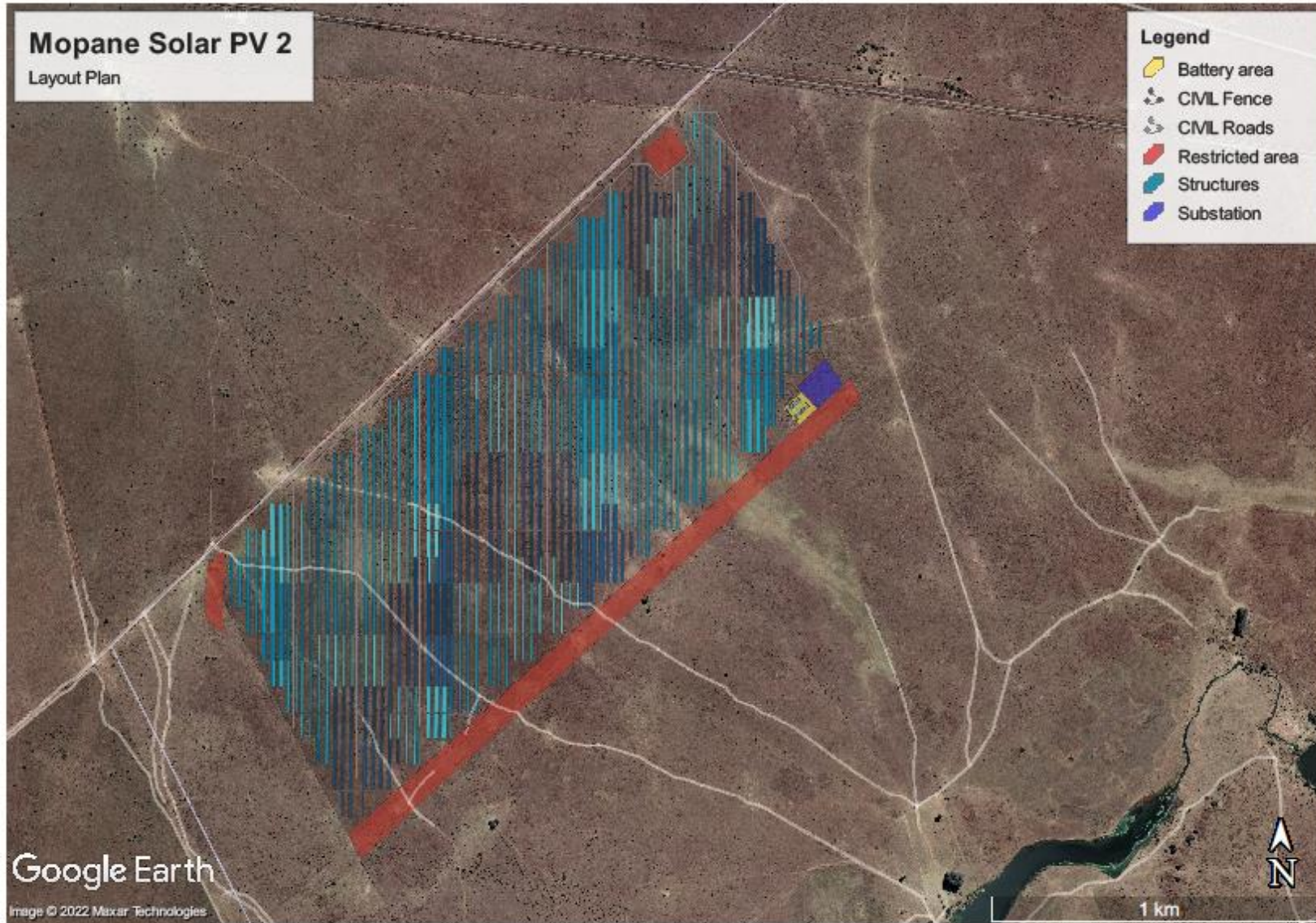
Figure 1. Proposed Draft Layout Plan of the Mopane Solar PV 2
