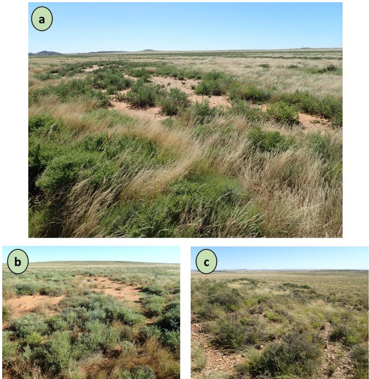
Figure 13: Alluvial fans
