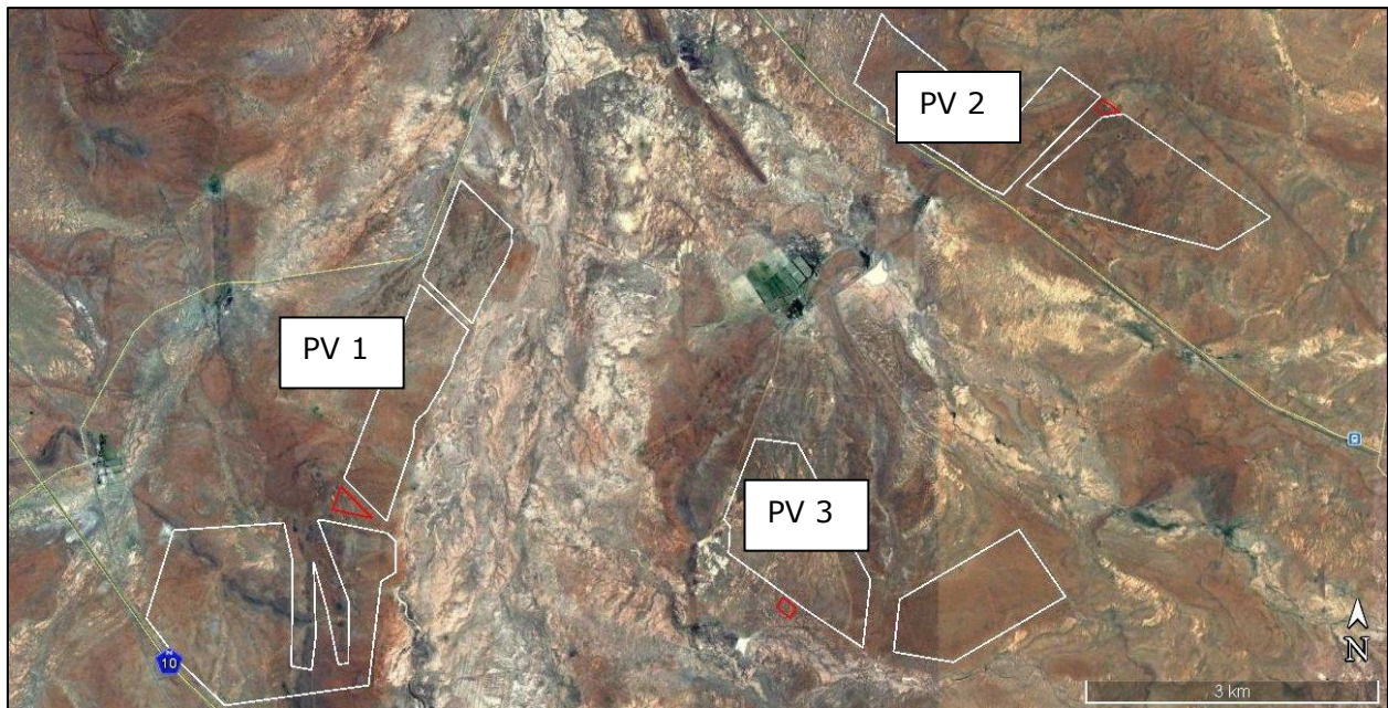
Figure 1. Satellite image of the Soventix solar development site, illustrating the proposed development alternatives, with the substation sites in red and the three PV sites (labelled 1,2 and 3) in white.
