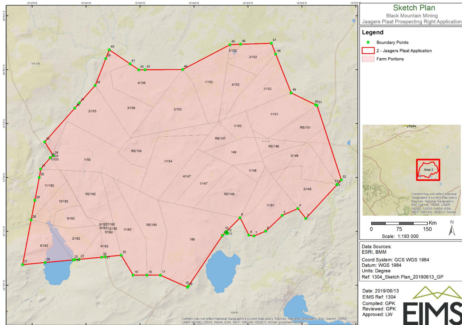
Figure 1: Locality Map
