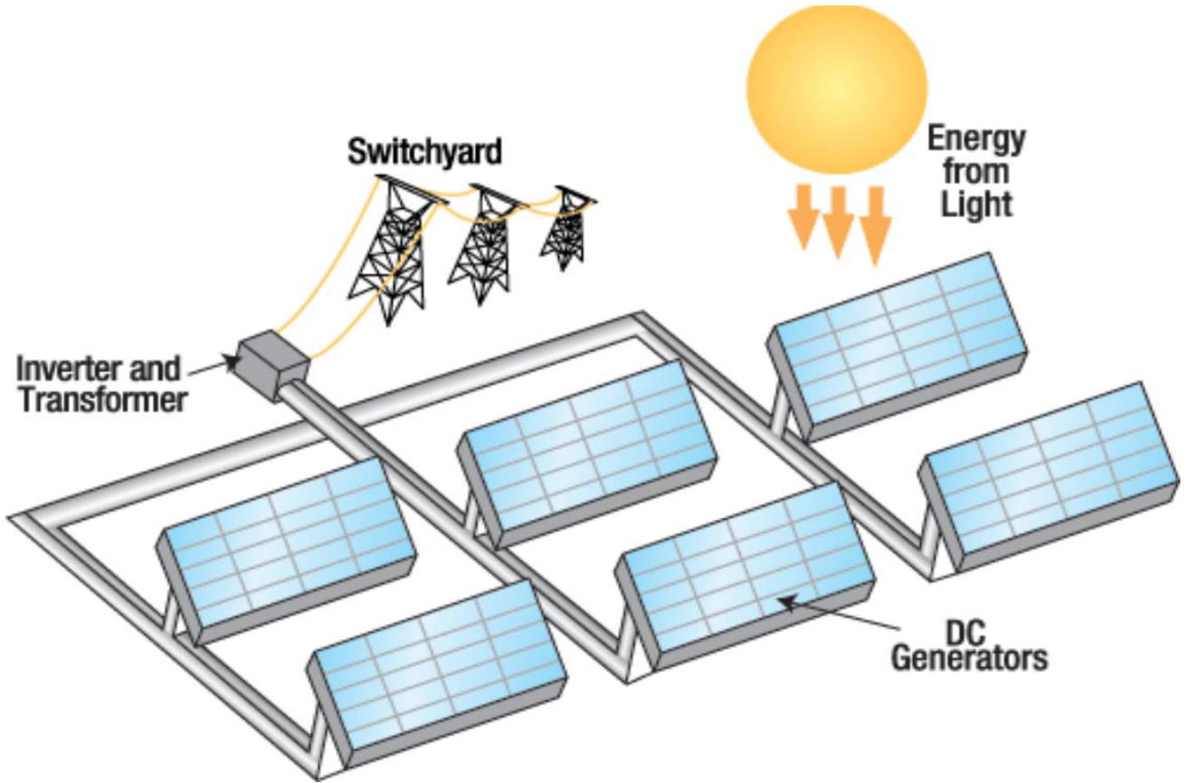
TYPICAL LAYOUT AND ILLUSTRATION OF THE PLANNED SOLAR (PV) ENERGY GENERATION PLANT
