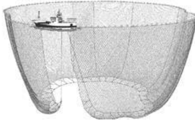
Figure 3.11: Schematic diagram showing typical configuration and deployment of a small pelagic purse-seine for targeting anchovy and sardine as used in South African waters.
