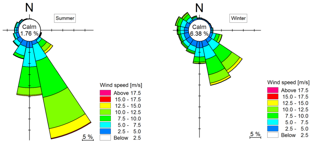
Figure 6: Wind Speed vs. Wind Direction for NCEP hind cast data at location 15° E, 31° S (From PRDW 2013).
