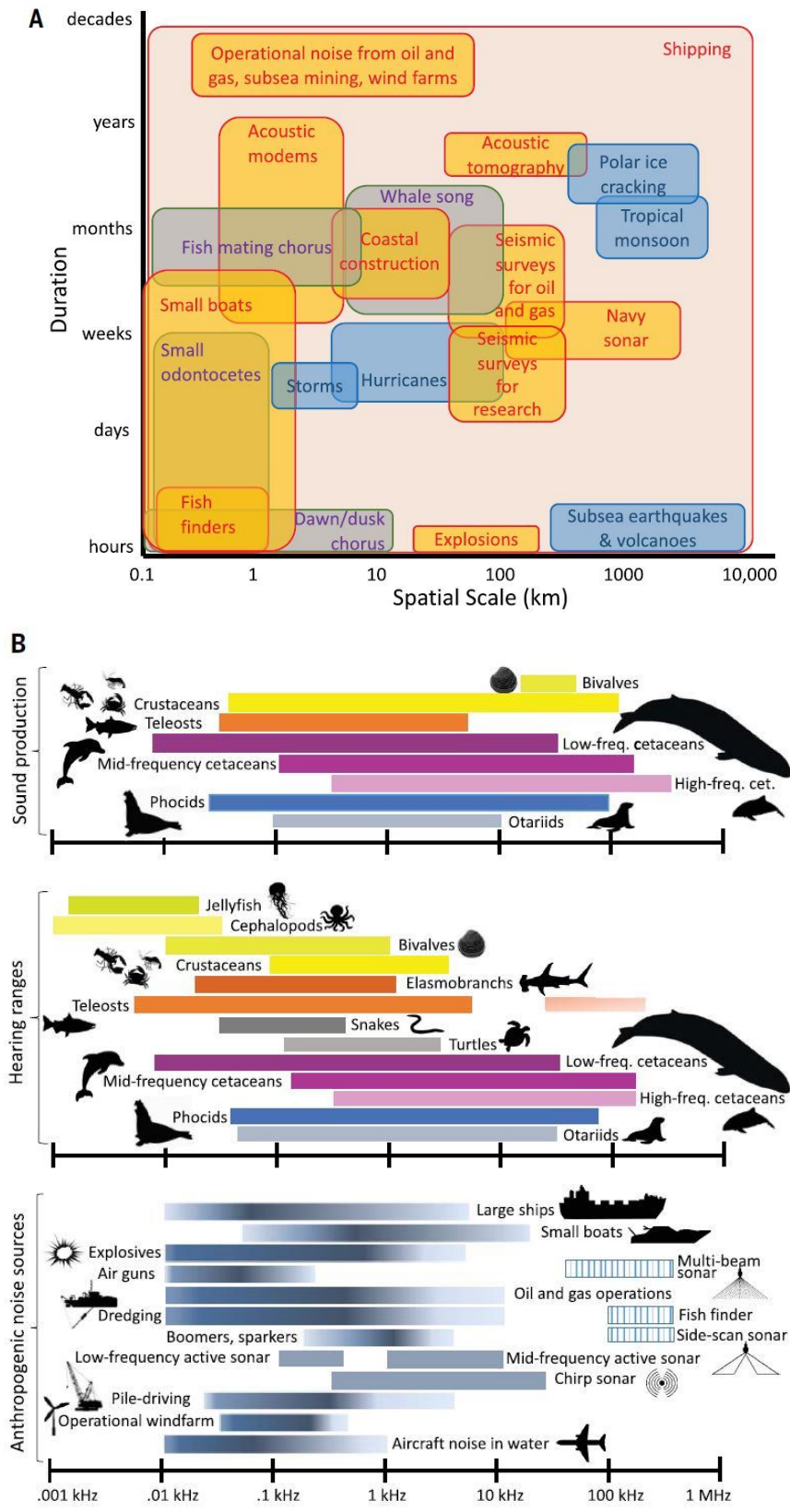
Figure 45: Sources and animal receivers of sound in the ocean. A) Spatial extent and duration of selected sound producing events, and B) Approximate sound production and hearing ranges of marine taxa and frequency ranges of selected anthropogenic sound sources. (Source: Duarte et al. 2021).
