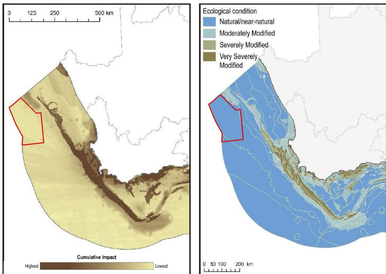
Figure 50: The Reconnaissance Permit Area (red polygon) in relation to cumulative impact on marine biodiversity, based the intensity of all cumulative pressures and the sensitivity of the underlying ecosystem types to each of those pressures (left) and the ecological condition of the marine realm based on the severity of modification as a result of the cumulative impacts (adapted from Sink et al. 2019 and Harris et al. 2022).
