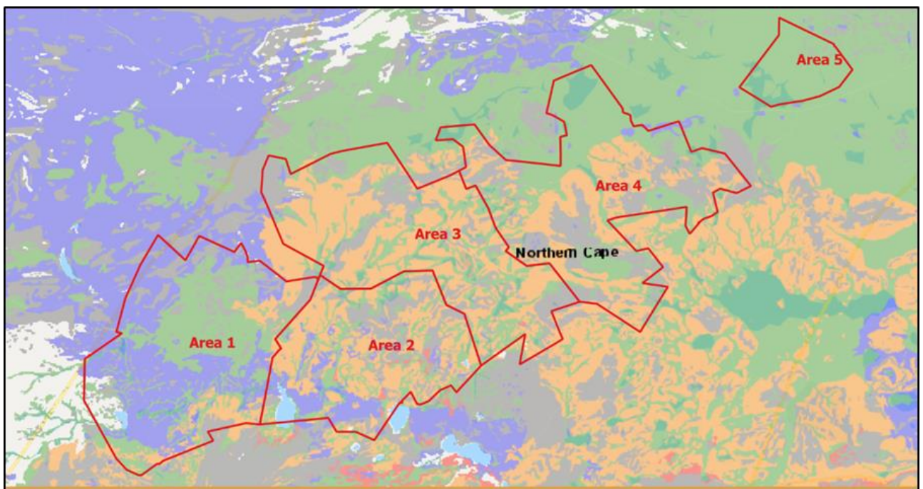
Figure 3: Extract of the 1: 250 000 SAHRIS Palaeosensitivity Map (Jaegers Plaet Application =Area 2)
