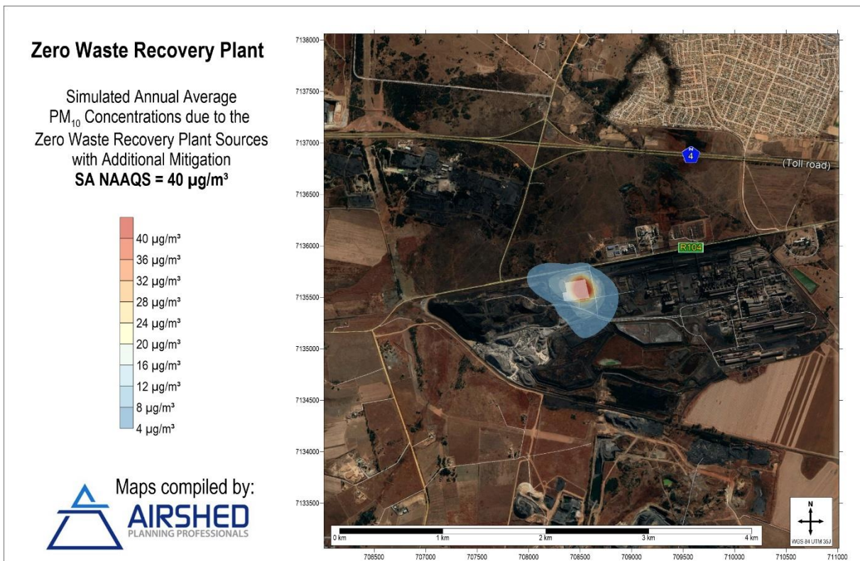
Figure 18: Simulated ground-level Annual Average PM 10 Concentrations – Incremental Impact of Zero-Waste Plant Sources with additional mitigation measures applied.
