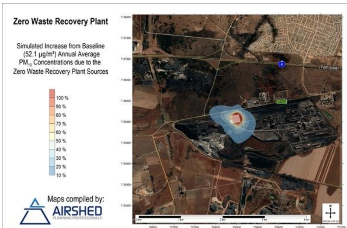
Figure 28: Simulated Increase from Baseline Annual Average PM 10 Concentrations–Cumulative Impact
