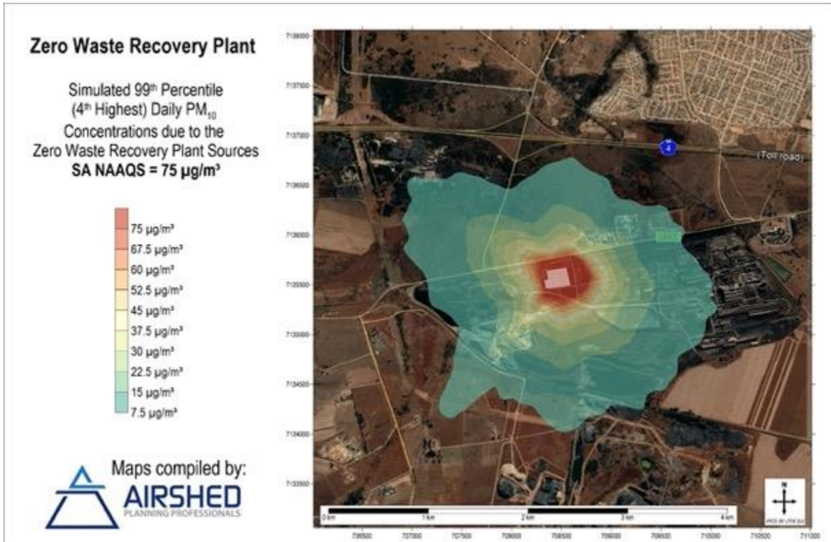
Figure 15: Simulated ground-level 99 th Percentile Daily PM 10 Concentrations – Incremental Impact of Zero-Waste Plant Sources Only
