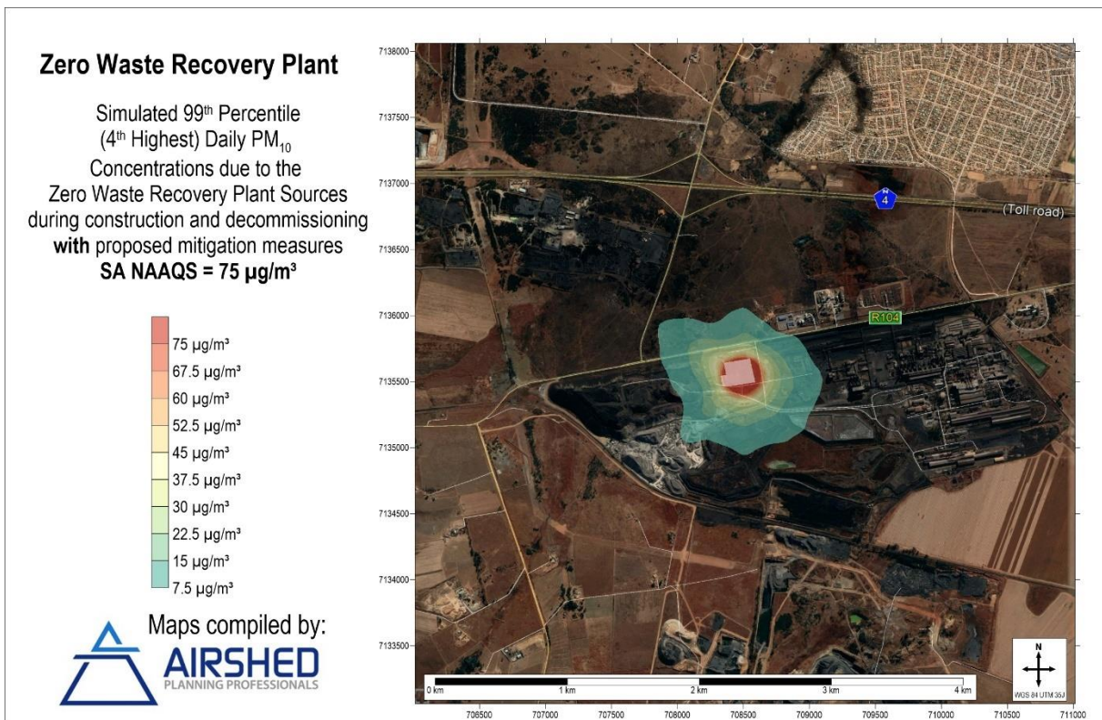
Figure 39: Simulated ground-level 99 th Percentile Daily PM 10 Concentrations – Incremental Impact during the construction and decommissioning phases with recommended mitigation measures (Table 27).
