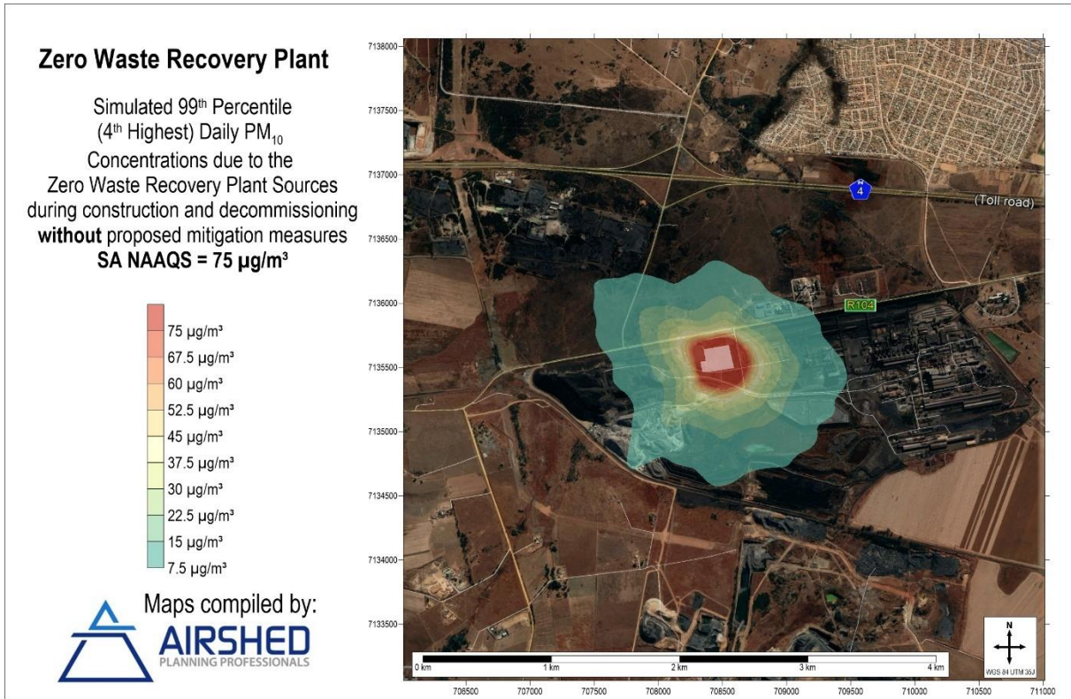
Figure 38: Simulated ground-level 99 th Percentile Daily PM 10 Concentrations – Incremental Impact during the construction and decommissioning phases with no mitigation.
