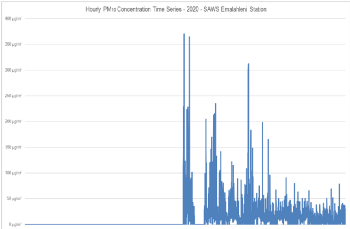
Figure 13: Time series – Hourly PM 10 concentrations – 2020 – SAWS Emalaheni Station
