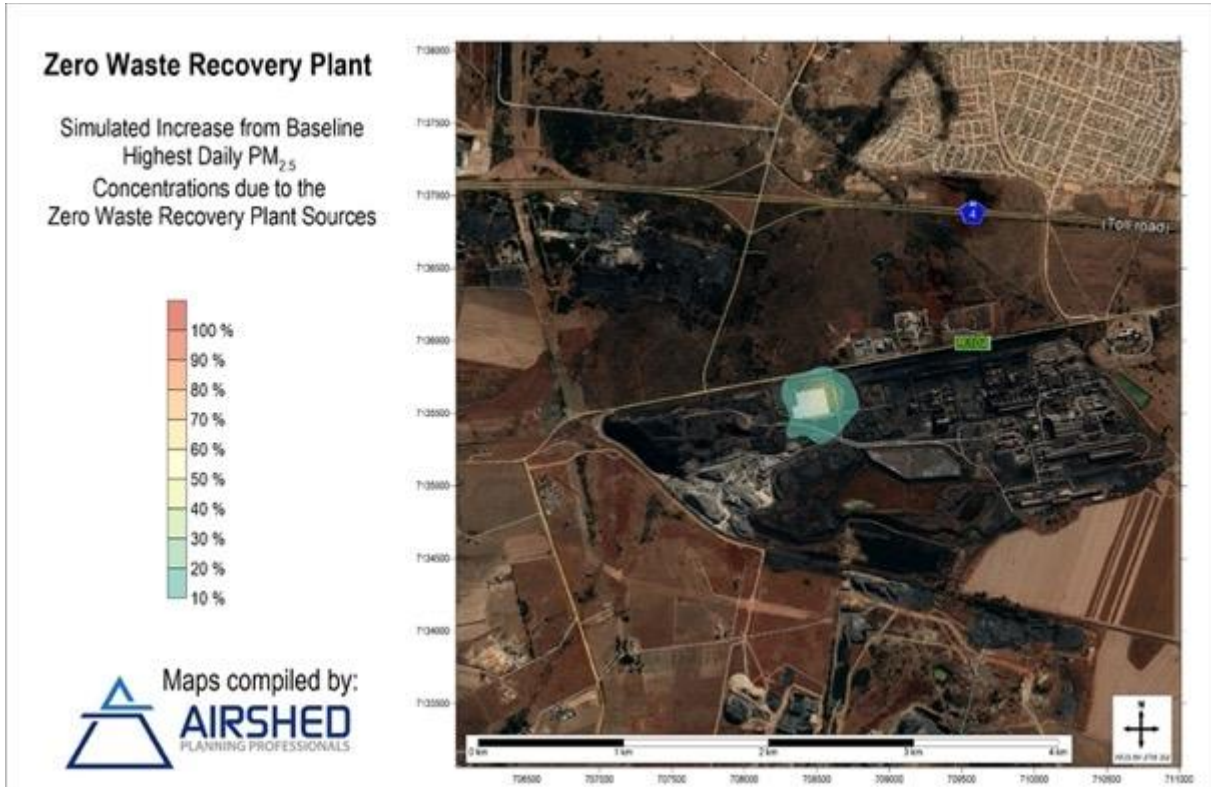
Figure 31: Simulated Increase from Baseline Highest Daily PM_{2.5} Concentrations – Cumulative Impact
