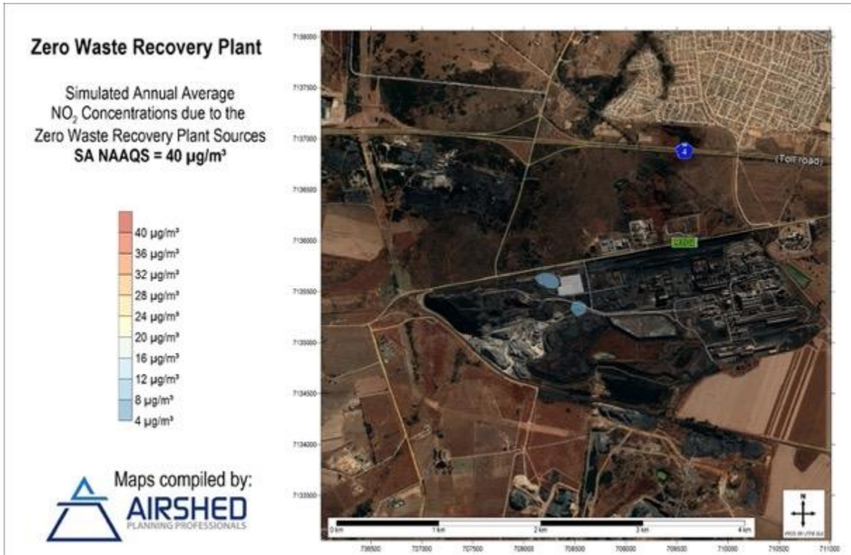
Figure 25: Simulated ground-level Annual Average NO 2 Concentrations – Incremental Impact of Zero-Waste Plant Sources Only
