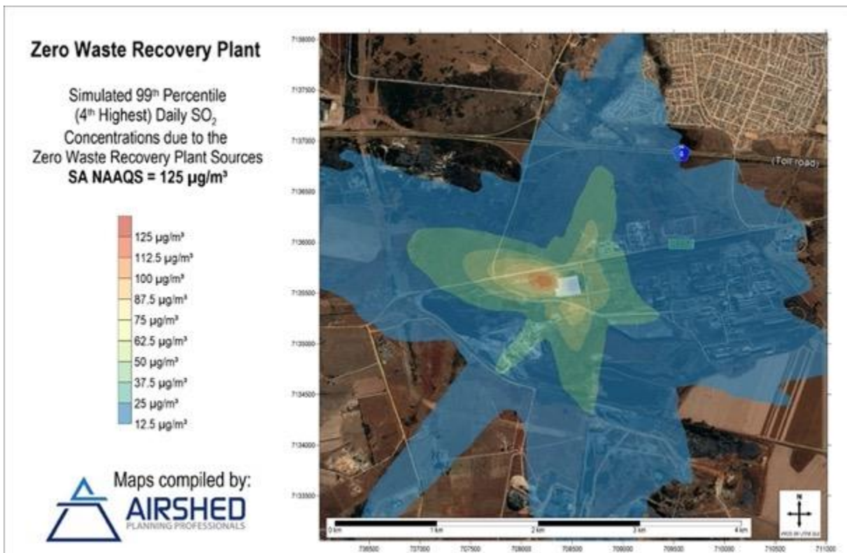
Figure 22: Simulated ground-level 99 th Percentile Daily SO 2 Concentrations – Incremental Impact of Zero-Waste Plant Sources Only
