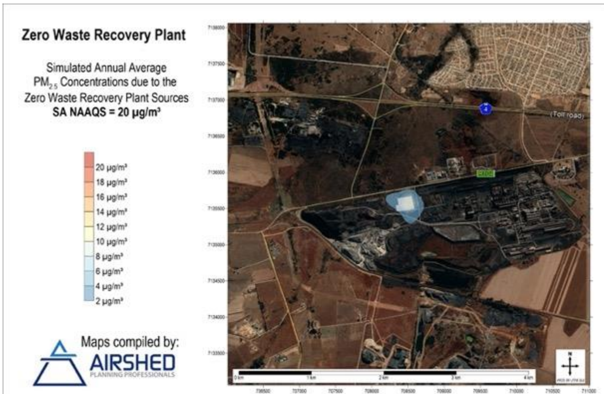
Figure 20: Simulated ground-level Annual Average PM 2.5 Concentrations– Incremental Impact of Zero-Waste Plant Sources Only
