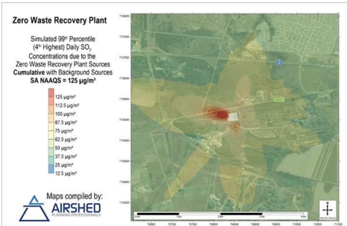
Figure 34: Simulated ground-level 99 th Percentile Daily SO 2 Concentrations - Cumulative Impact of Zero-Waste Plant Sources Together with Background Concentrations
