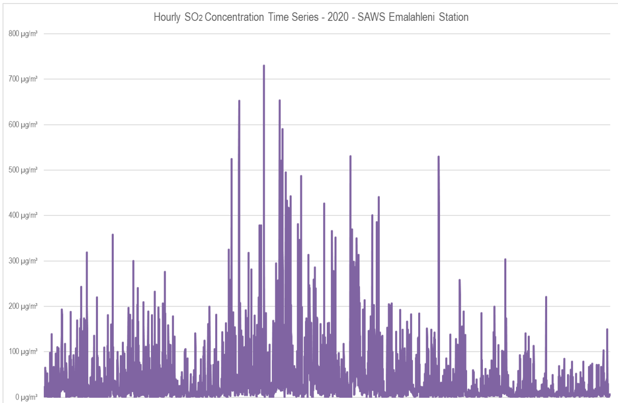
Figure 12: Time series – Hourly SO 2 concentrations – 2020 – SAWS Emalahleni Station
