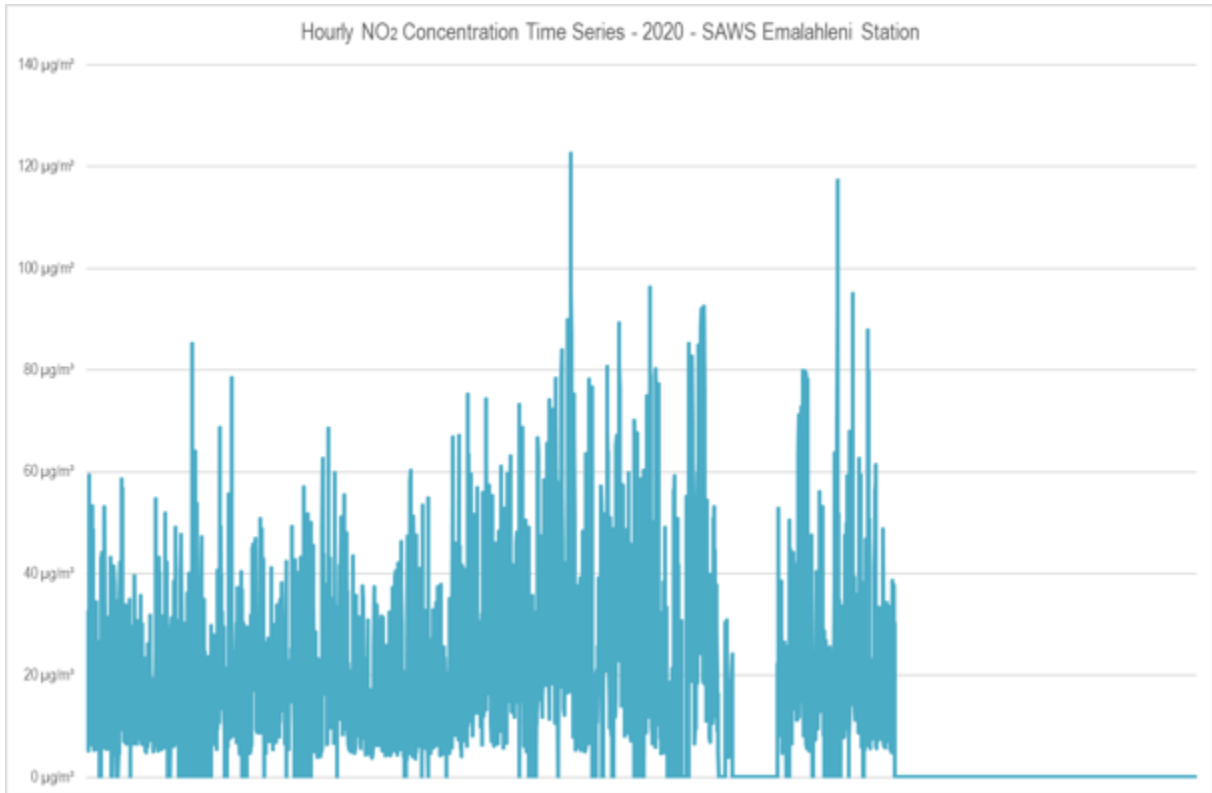
Figure 11: Time series – Hourly NO 2 concentrations – 2020 – SAWS Emalahleni Station
