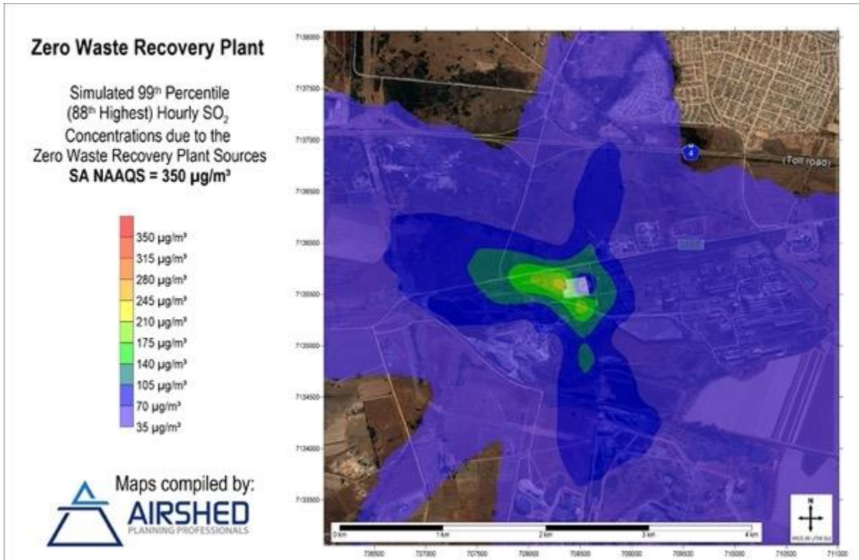
Figure 21: Simulated ground-level 99 th Percentile Hourly SO 2 Concentrations – Incremental Impact of Zero-Waste Plant Sources Only
