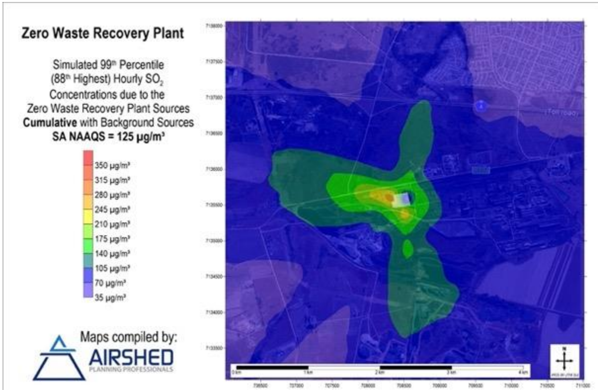
Figure 33: Simulated ground-level 99 th Percentile Hourly SO 2 Concentrations - Cumulative Impact of Zero-Waste Plant Sources Together with Background Concentrations
