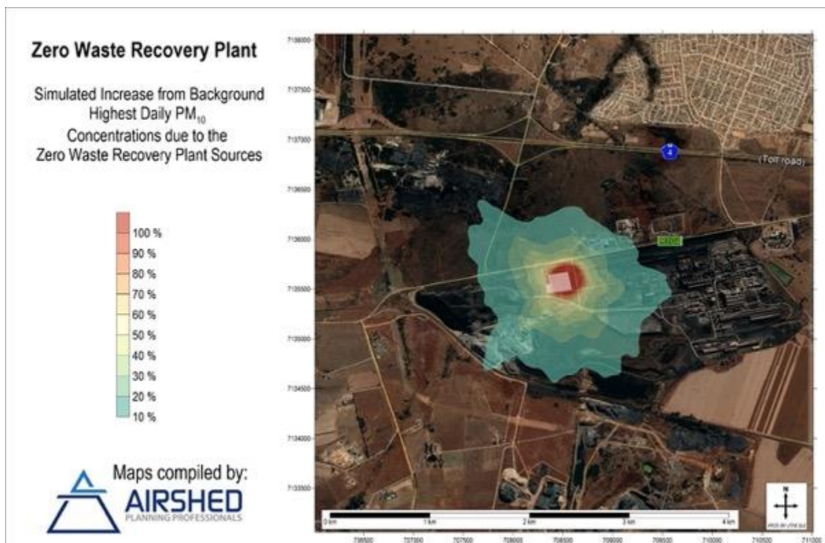
Figure 27: Simulated Increase from Baseline Highest Daily PM 10 Concentrations – Cumulative Impact
