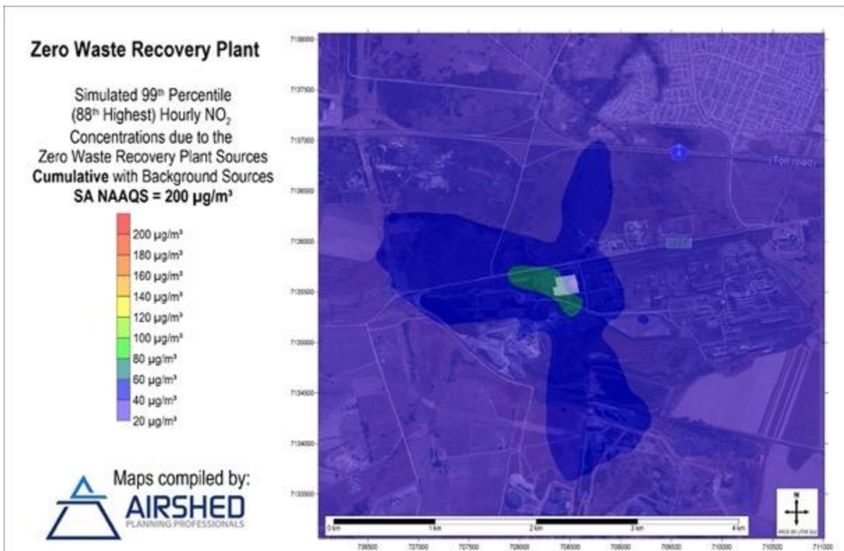
Figure 36: Simulated ground-level 99 th Percentile Hourly \text{NO}_2 Concentrations - Cumulative Impact of Zero-Waste Plant Sources Together with Background Concentrations
