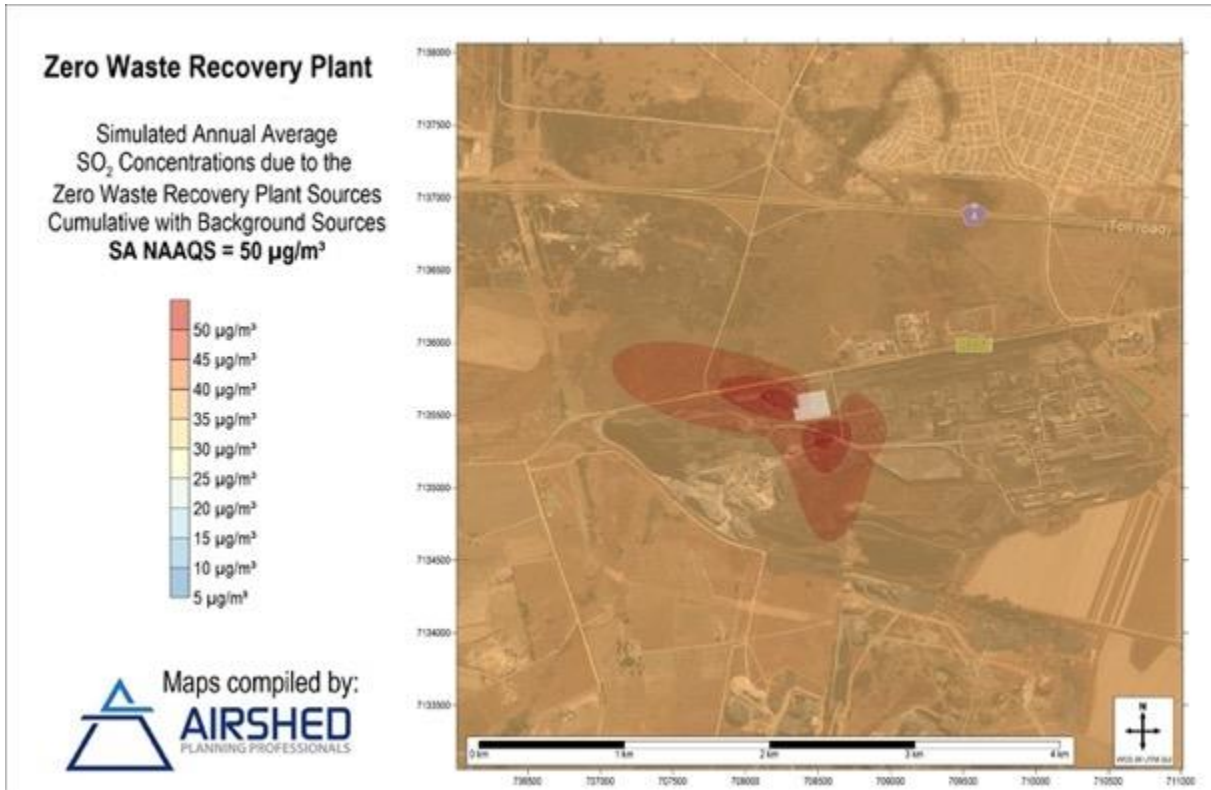
Figure 35: Simulated ground-level Annual Average \text{SO}_2 Concentrations – Cumulative Impact of Zero-Waste Plant Sources Together with Background Concentrations
