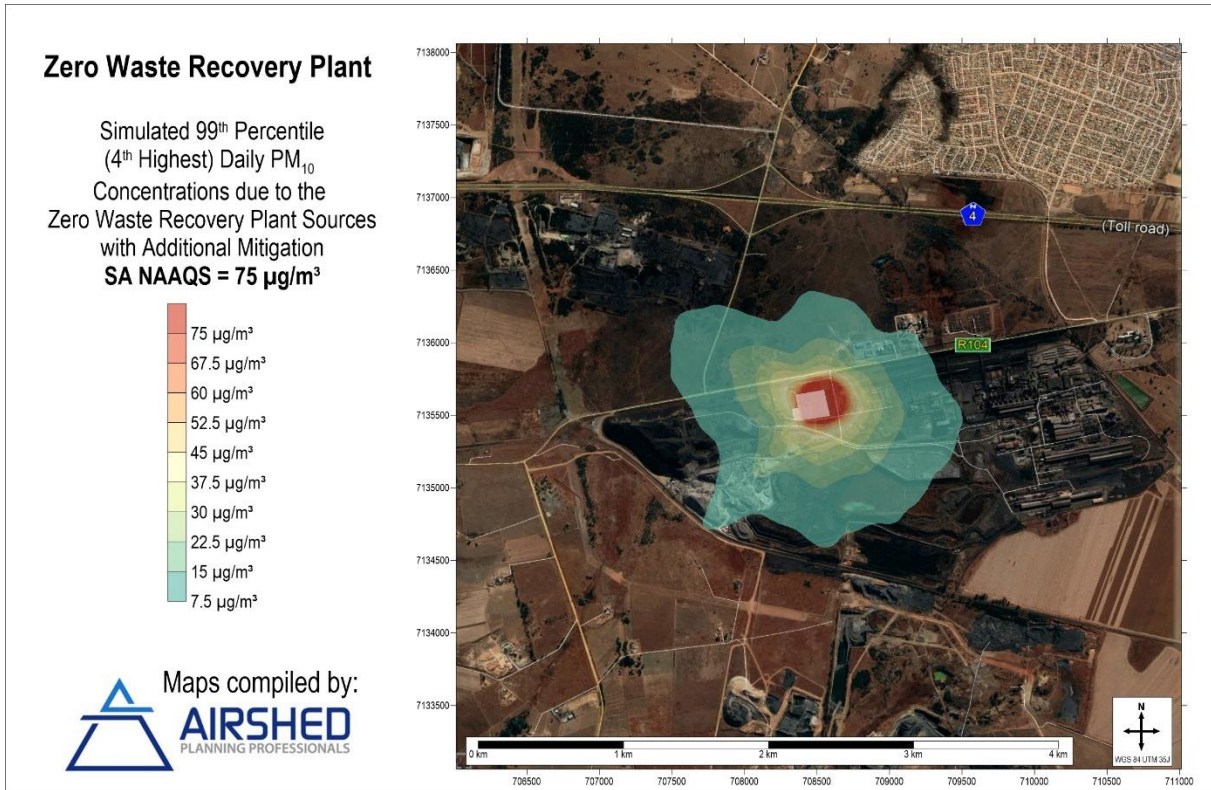
Figure 17: Simulated ground-level 99 th Percentile Daily PM 10 Concentrations – Incremental Impact of Zero-Waste Plant Sources with additional mitigation measures applied.
