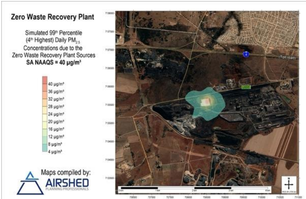
Figure 19: Simulated Ground-level 99 th Percentile Daily PM 2.5 Concentrations – Incremental Impact of Zero-Waste Plant Sources Only
