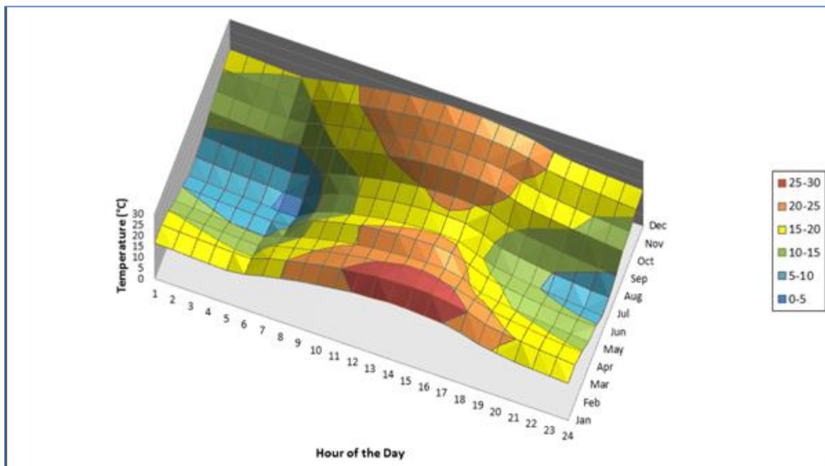
Figure 10: Monthly average temperature profile for SAWS Emalahleni
