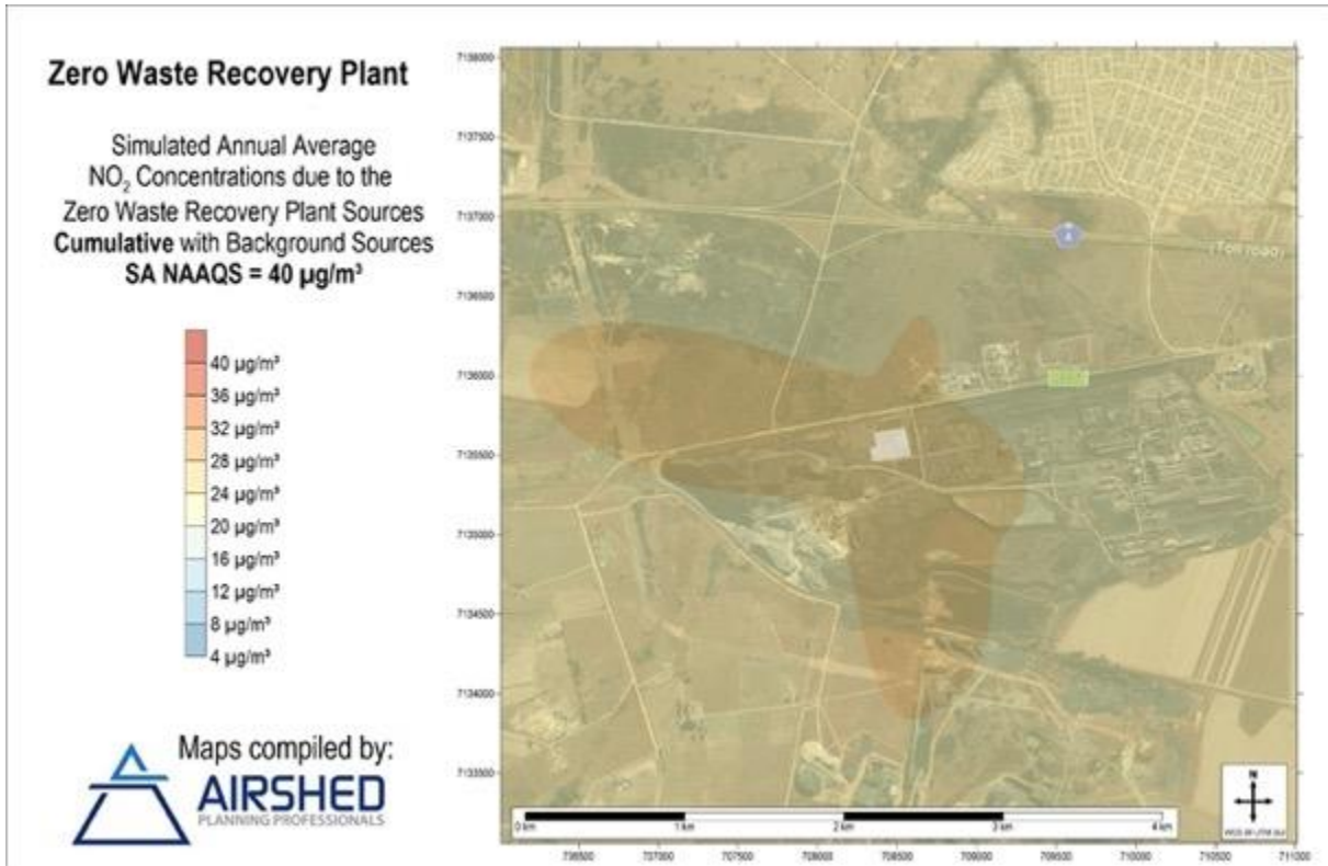
Figure 37: Simulated ground-level Annual Average NO 2 Concentrations - Cumulative Impact of Zero-Waste Plant Sources Together with Background Concentrations
