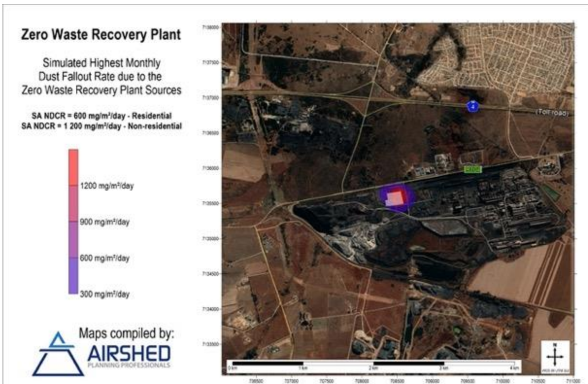
Figure 26: Simulated ground-level Highest Monthly Dust Fallout Rate – Incremental Impact of Zero-Waste Plant Sources Only
