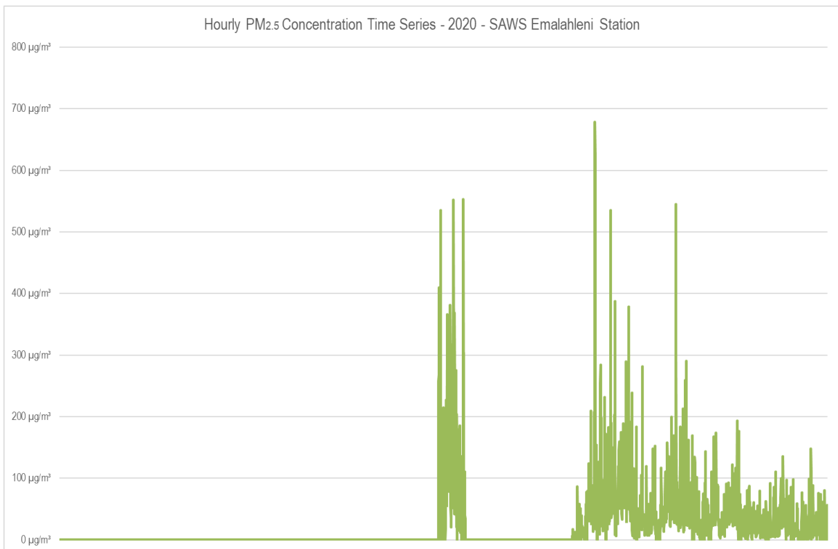
Figure 14: Time series – Hourly PM 2.5 concentrations – 2020 – SAWS Emalaheni Station
