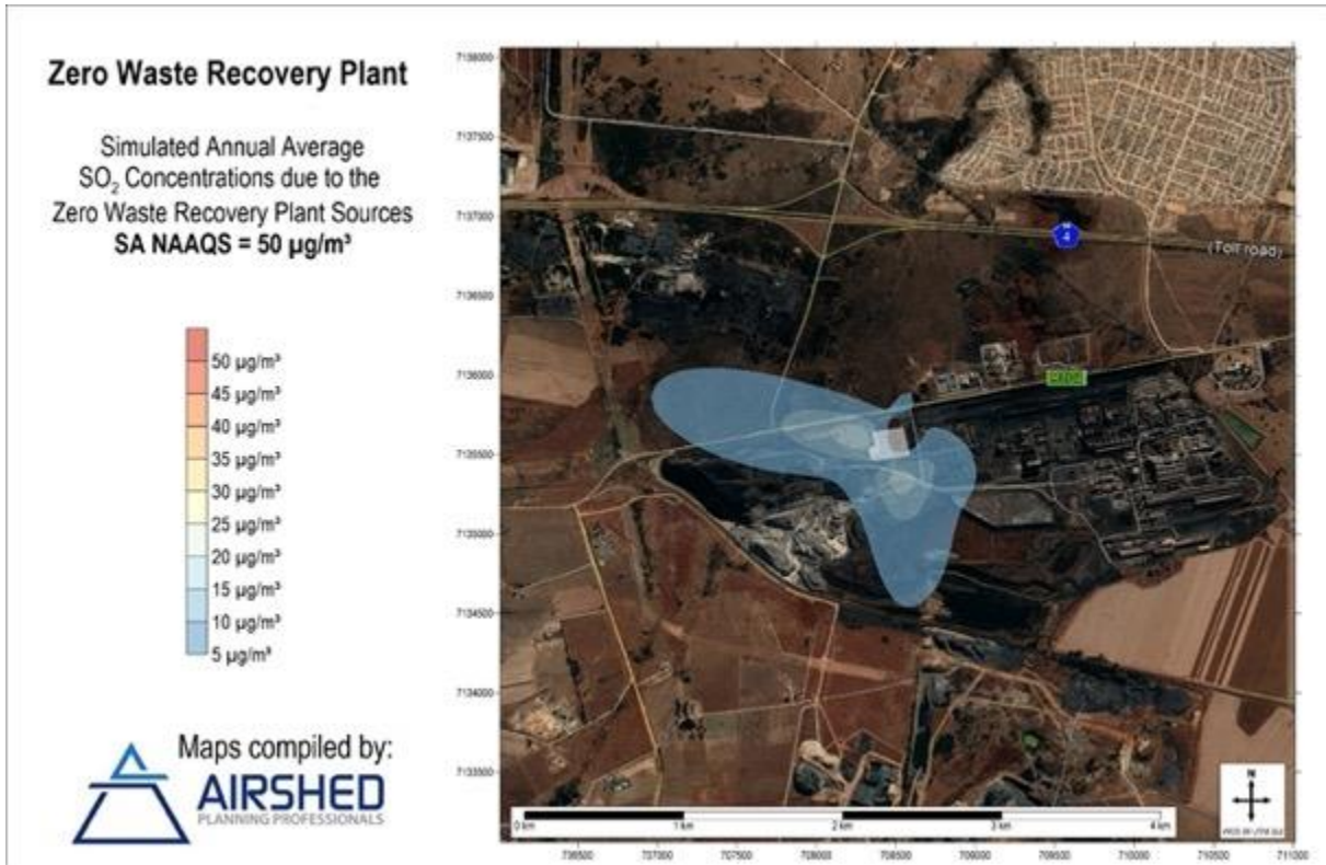
Figure 23: Simulated ground-level Annual Average \text{SO}_2 Concentrations – Incremental Impact of Zero-Waste Plant Sources Only
