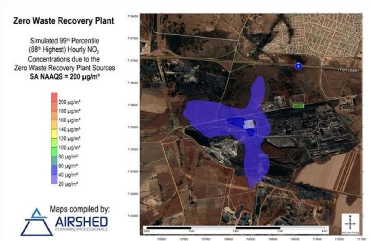
Figure 24: Simulated ground-level 99 th Percentile Hourly \text{NO}_2 Concentrations – Incremental Impact of Zero-Waste Plant Sources Only
