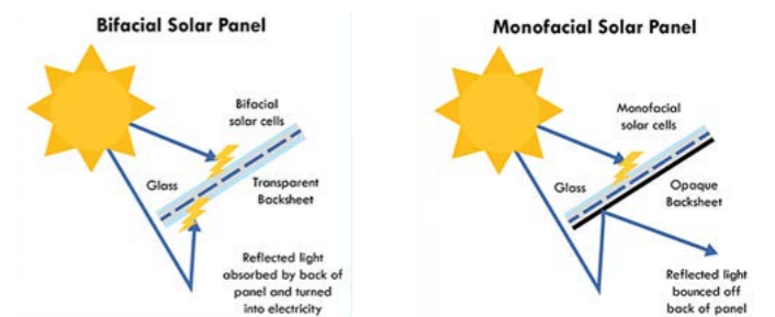
Figure 4: Diagram showing how bifacial and monofacial Solar PV panels work (Source: https://www.solarkobo.com/post/bifacial-solar-panels )
