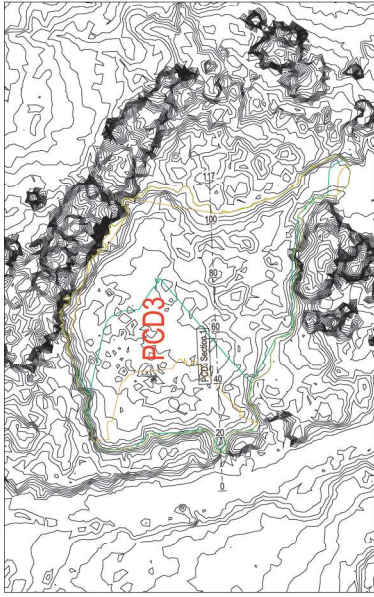
PCD3 LAYOUT SCALE 1:1000
