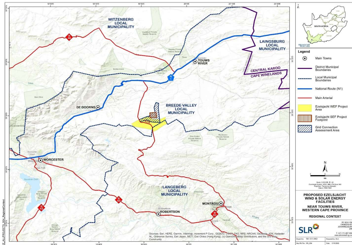
Figure 1: Locality Map
