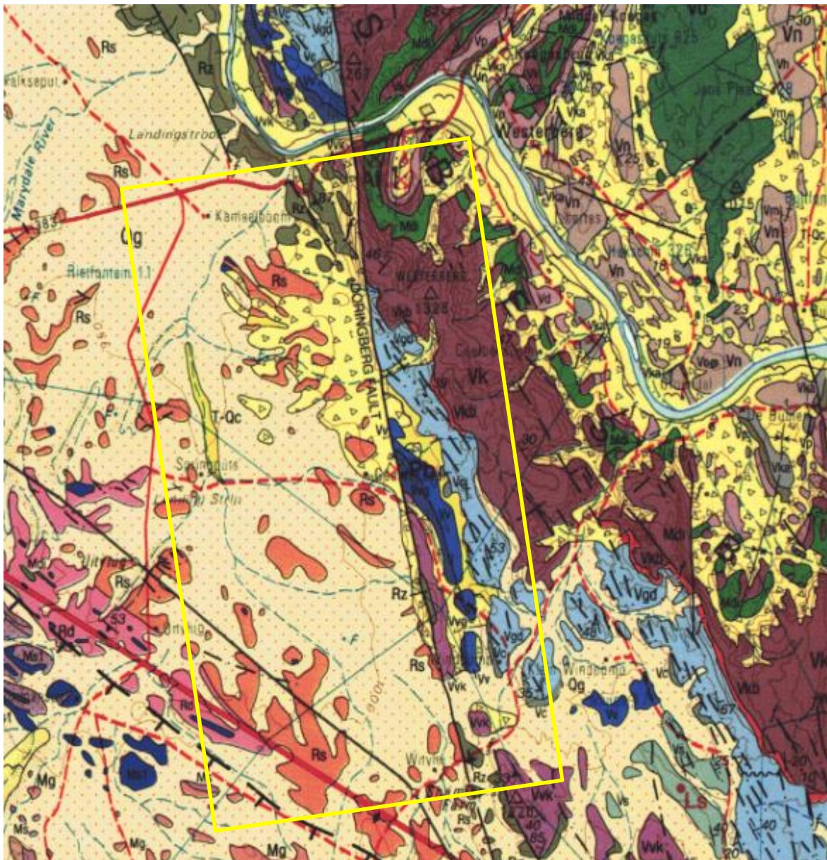
Figure 2: Geological map of the area around the Farms Rietfontein 11 and Nauga 17 with the prospecting area indicated within the yellow rectangle. Abbreviations of the rock types are explained in Table 2. Map enlarged from the Geological Survey 1: 250 000 map 2922 Prieska.
