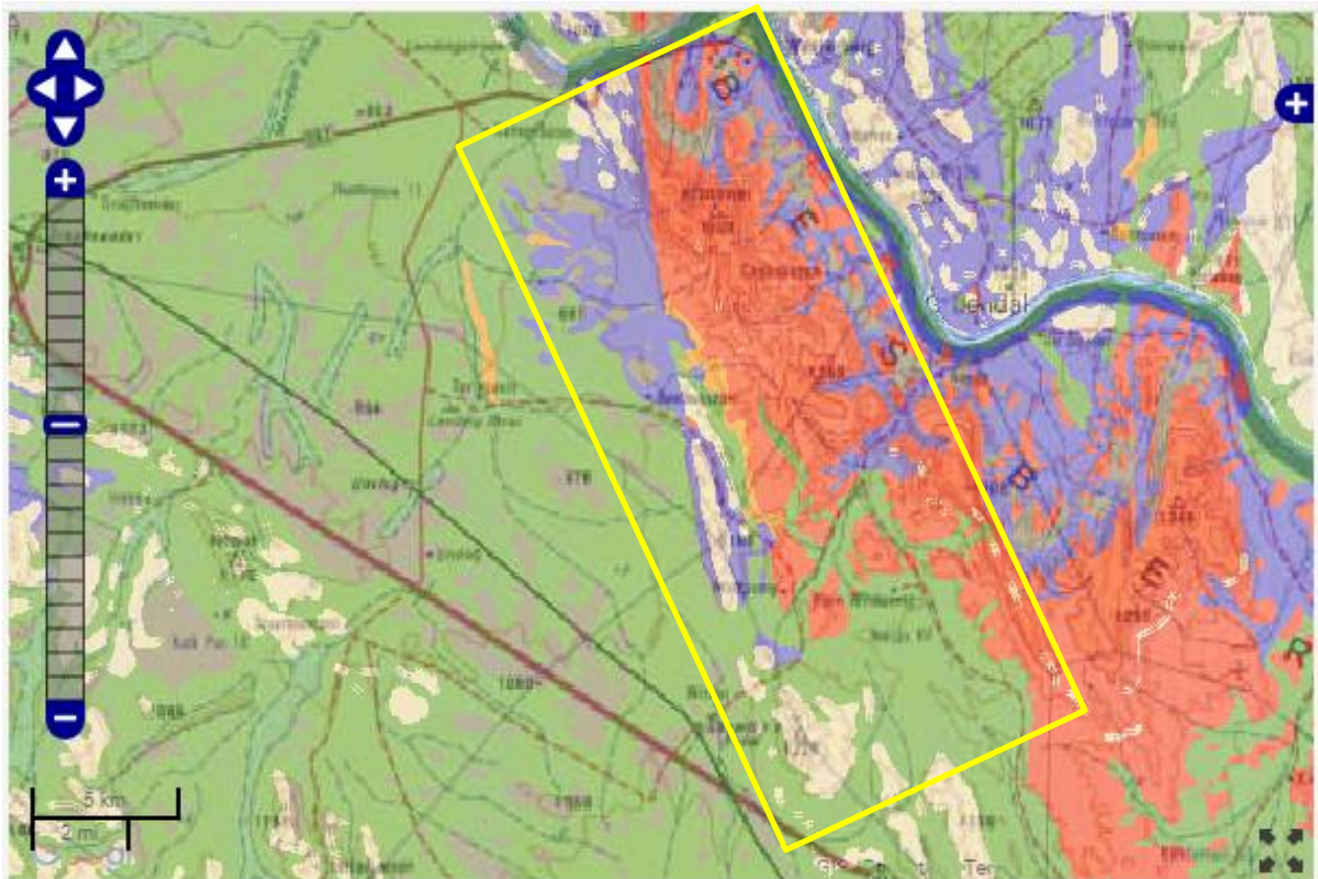
Figure 3: SAHRIS palaeosensitivity map for the site for the proposed PRA on Farms Rietfontein 11 and Nauga 17 (project 2) shown within the yellow rectangle. Background colours indicate the following degrees of sensitivity: red = very highly sensitive; orange/yellow = high; green = moderate; blue = low; grey = insignificant/zero.
