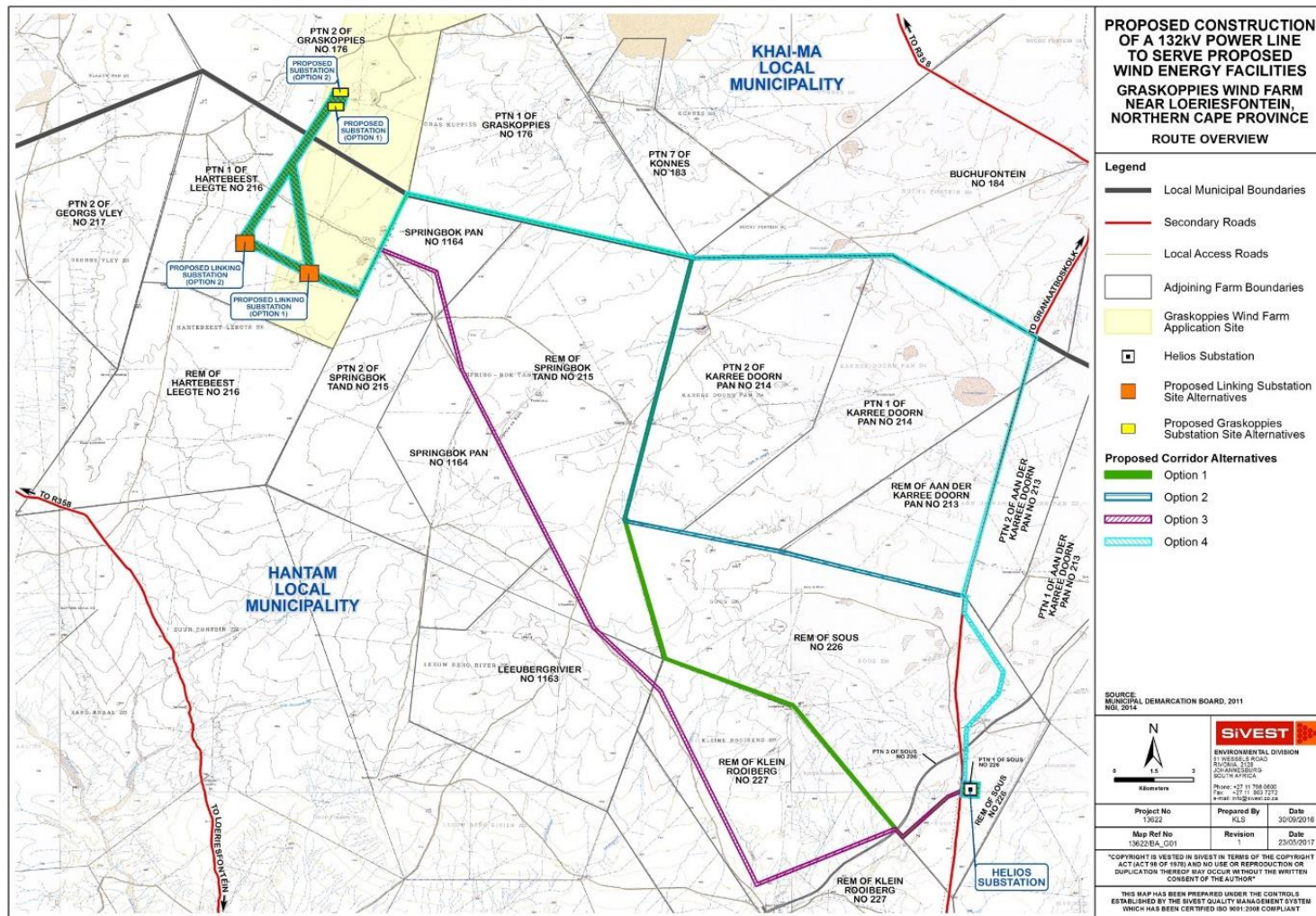
Figure 2: The proposed layout of the Graskoppies grid connection, showing the various corridor alternatives
