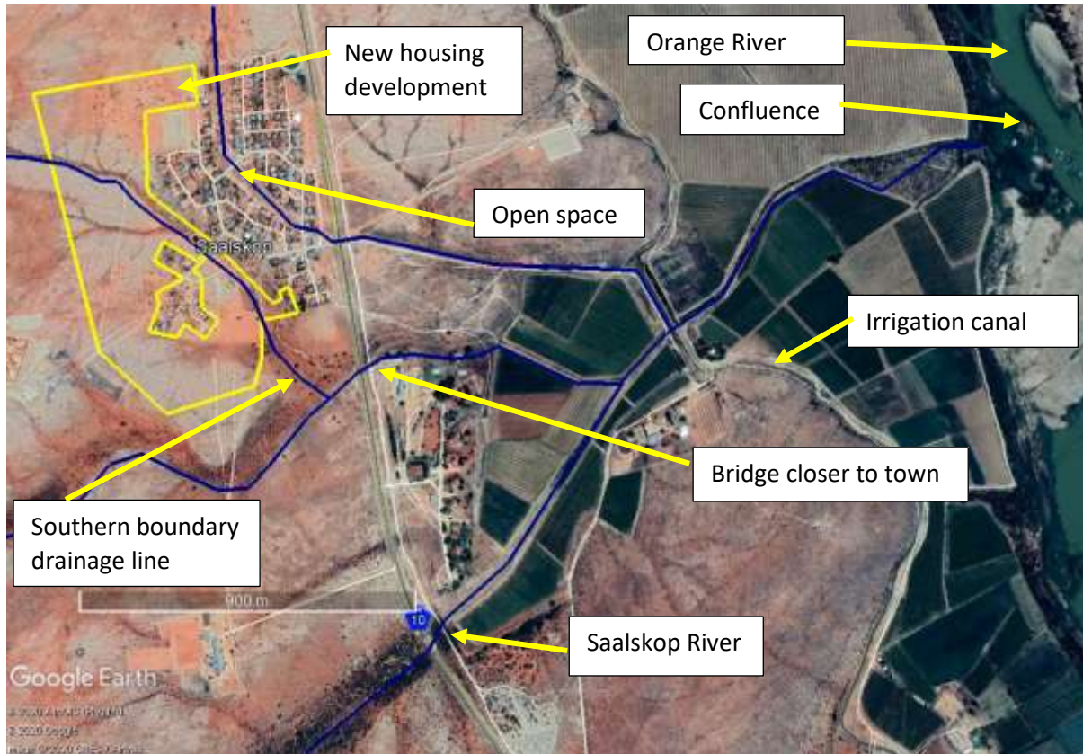
Figure 11 Topline drainage lines
