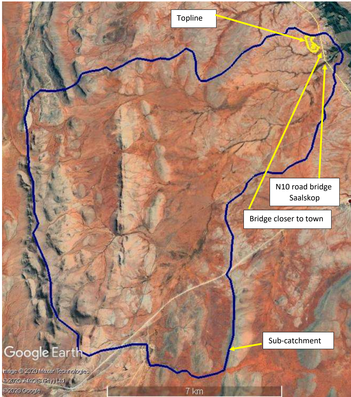
Figure 7 Topline Housing drainage line
