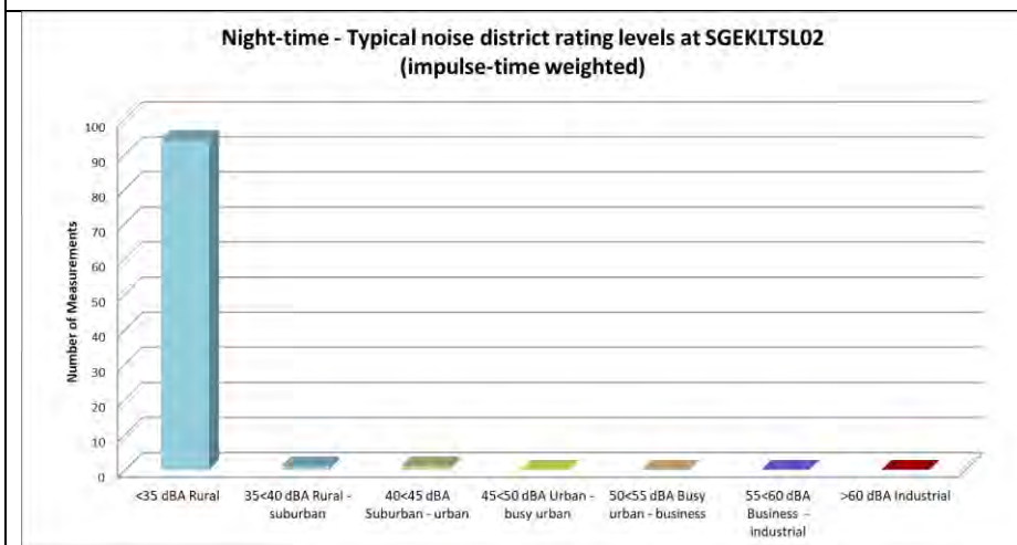
Figure 13: Classification of night-time measurements in typical noise districts at SGEKLTSL02
