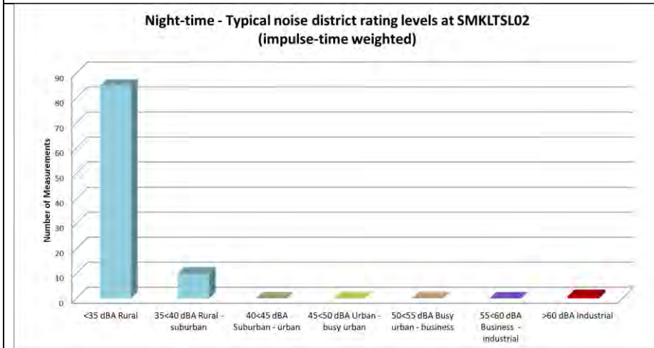
Figure 25: Classification of night-time measurements in typical noise districts at SMKLTSL02
