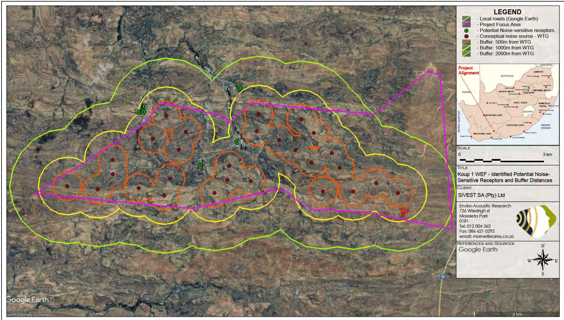
Figure 4: Aerial Image indicating closest NSD as identified during the site visit as well as buffer areas around the WTG
