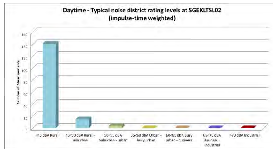
Figure 14: Classification of daytime measurements in typical noise districts at SGEKLTSL02
