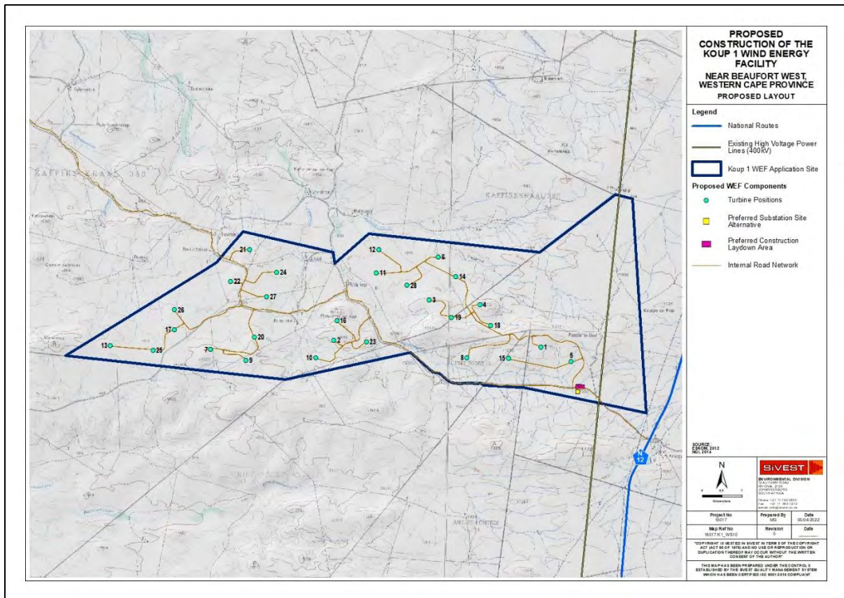
Figure 4: Infrastructure proposed as part of the Koupi 1 WEF
