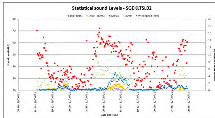
Figure 12: Maximum, minimum and statistical values at SGEKLTSL02
