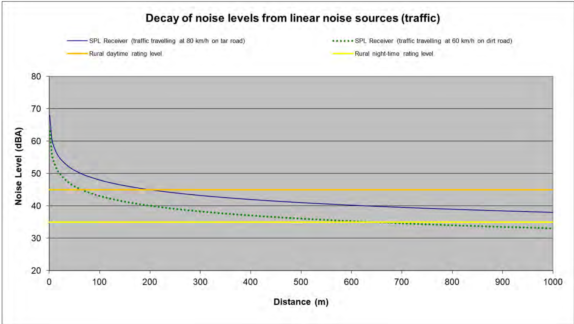
Figure 45: Projected conceptual construction noise levels – Decay over distance from linear activities
