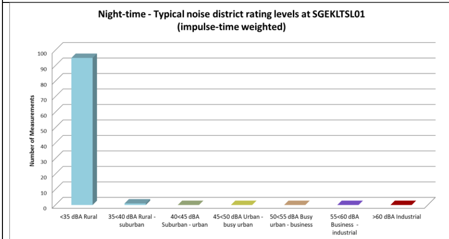
Figure 9: Classification of night-time measurements in typical noise districts at SGEKLTSL01
