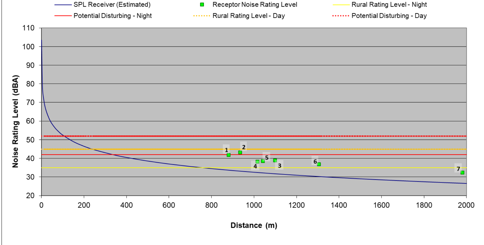
Figure 44: Projected conceptual construction noise levels - Decay of noise from construction activities
