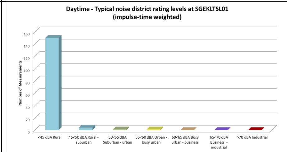
Figure 10: Classification of daytime measurements in typical noise districts at SGEKLTSL01
