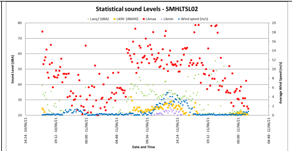
Figure 32: Maximum, minimum and Statistical sound levels at SMHLTSL02
