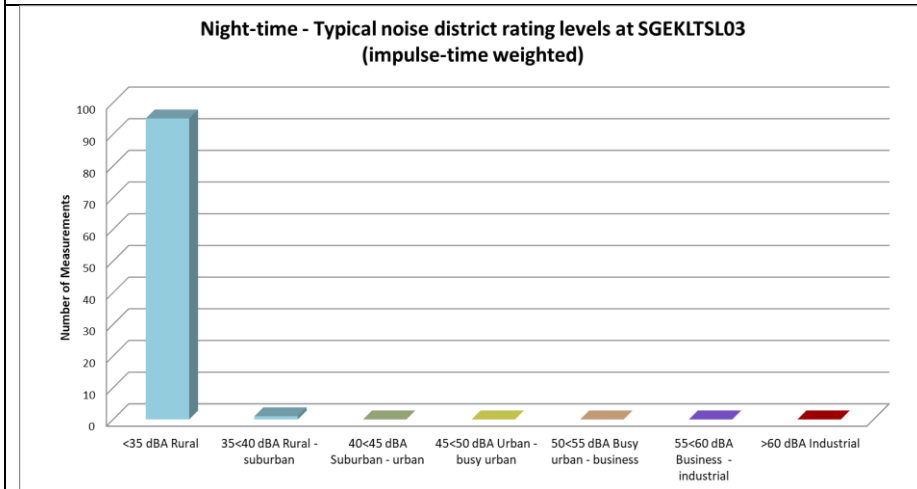
Figure 17: Classification of night-time measurements in typical noise districts at SGEKLTSL03
