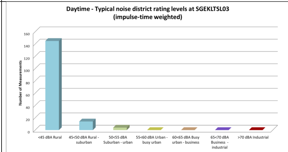
Figure 18: Classification of daytime measurements in typical noise districts at SGEKLTSL03
