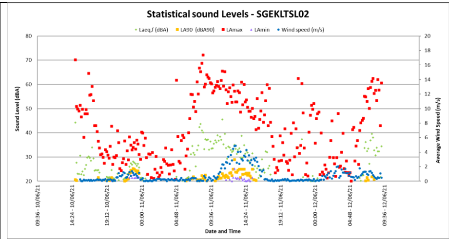
Figure 12: Maximum, minimum and statistical values at SGEKLTSL02
