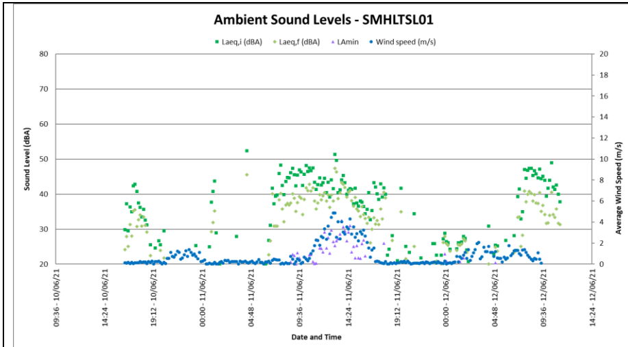
Figure 27: Residual noise Levels at SMHLTSL01
