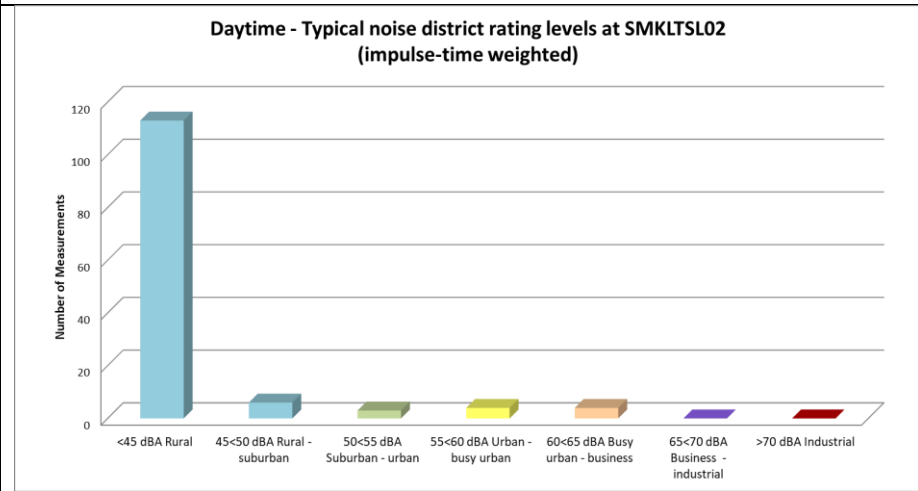
Figure 26: Classification of daytime measurements in typical noise districts at SMKLTSL02
