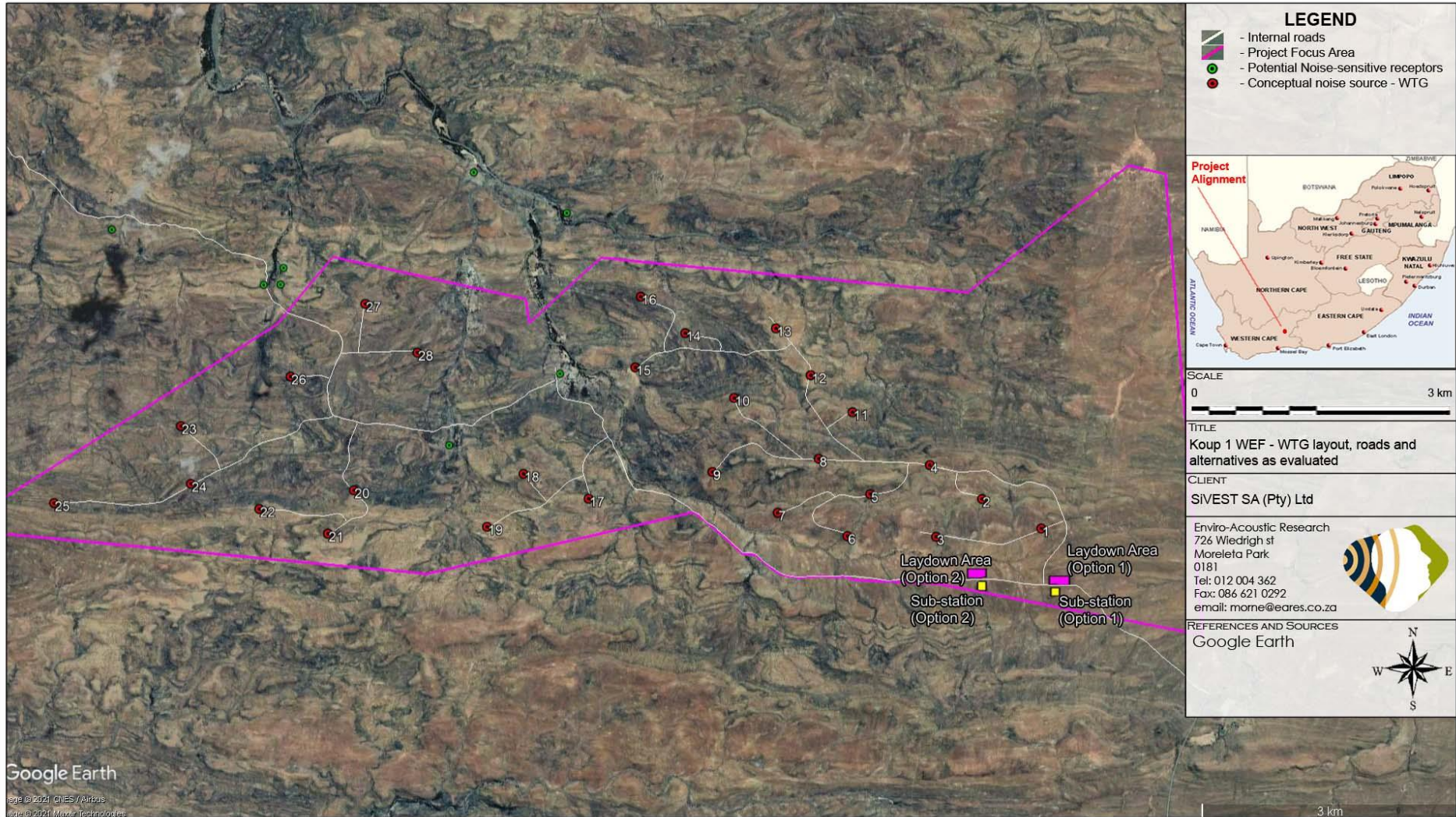
Figure 43: Proposed WTG Layout of the Koup 1 WEF
