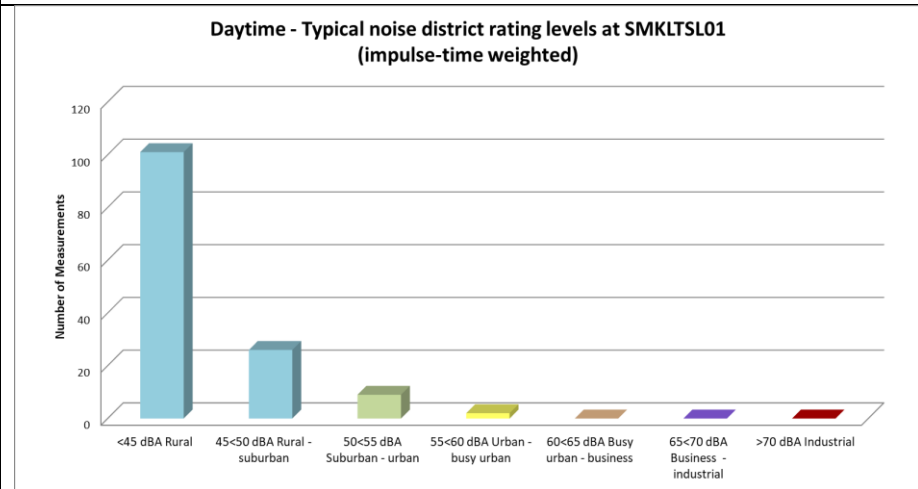
Figure 22: Classification of daytime measurements in typical noise districts at SMKLTSL01
