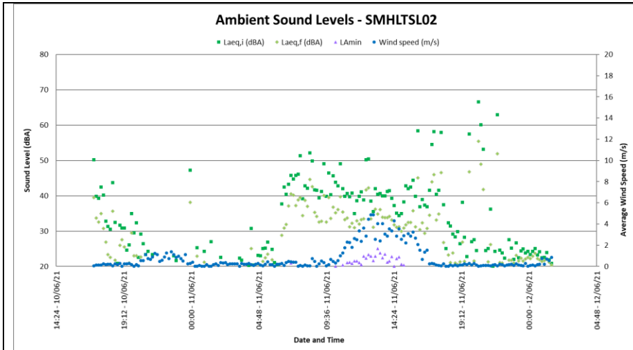
Figure 31: Residual noise Levels at SMHLTSL02
