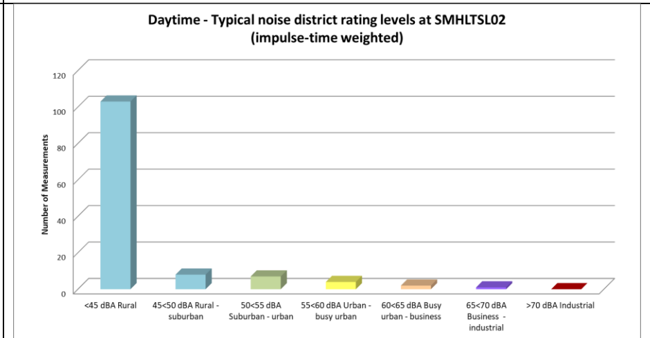
Figure 34: Classification of daytime measurements in typical noise districts at SMHLTSL02
