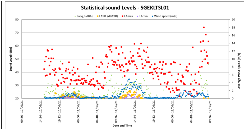
Figure 8: Maximum, minimum and Statistical sound levels at SGEKLTSL01
