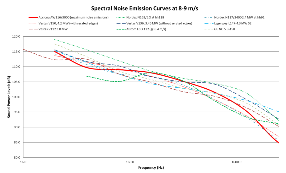
Figure 37: Octave sound power emissions of various wind turbines
