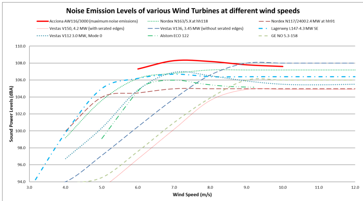
Figure 36: Noise Emissions Curve of a number of different wind turbines (figure for illustration purposes only)
