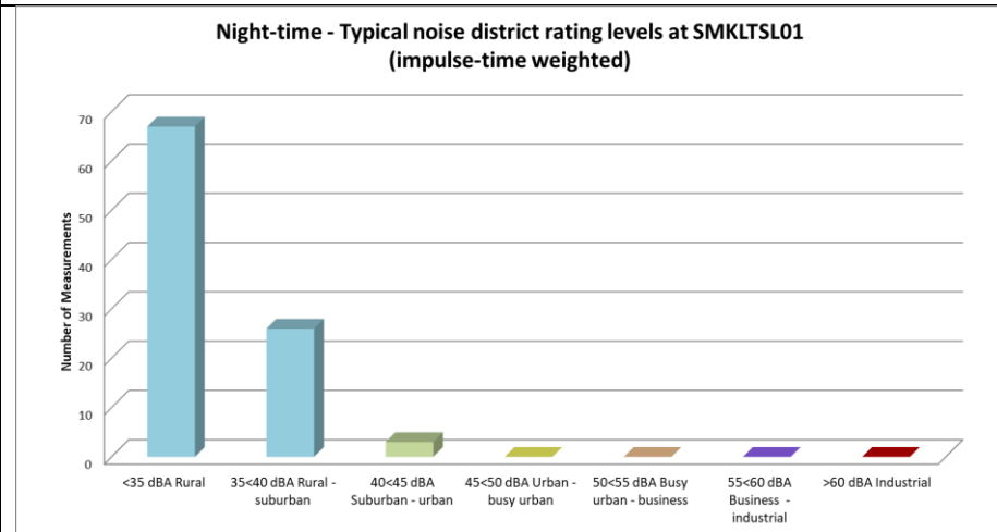
Figure 21: Classification of night-time measurements in typical noise districts at SMKLTSL01
