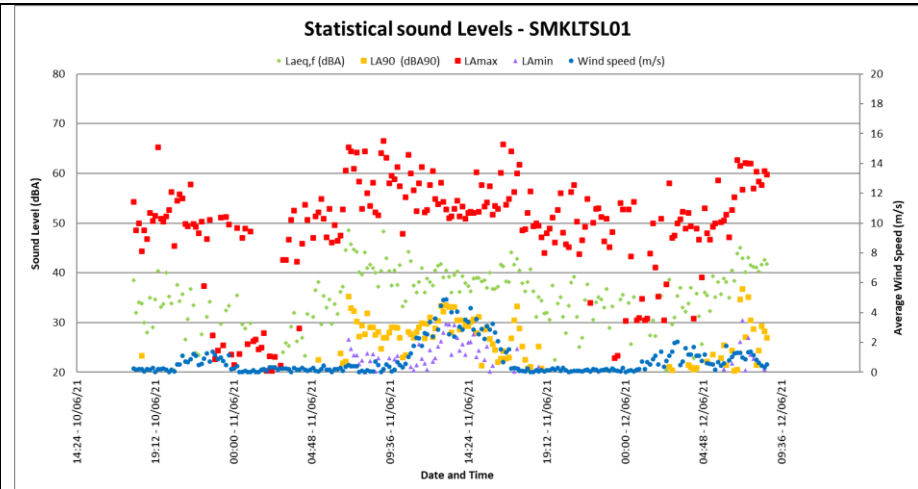
Figure 20: Maximum, minimum and Statistical sound levels at SMKLTSL01
