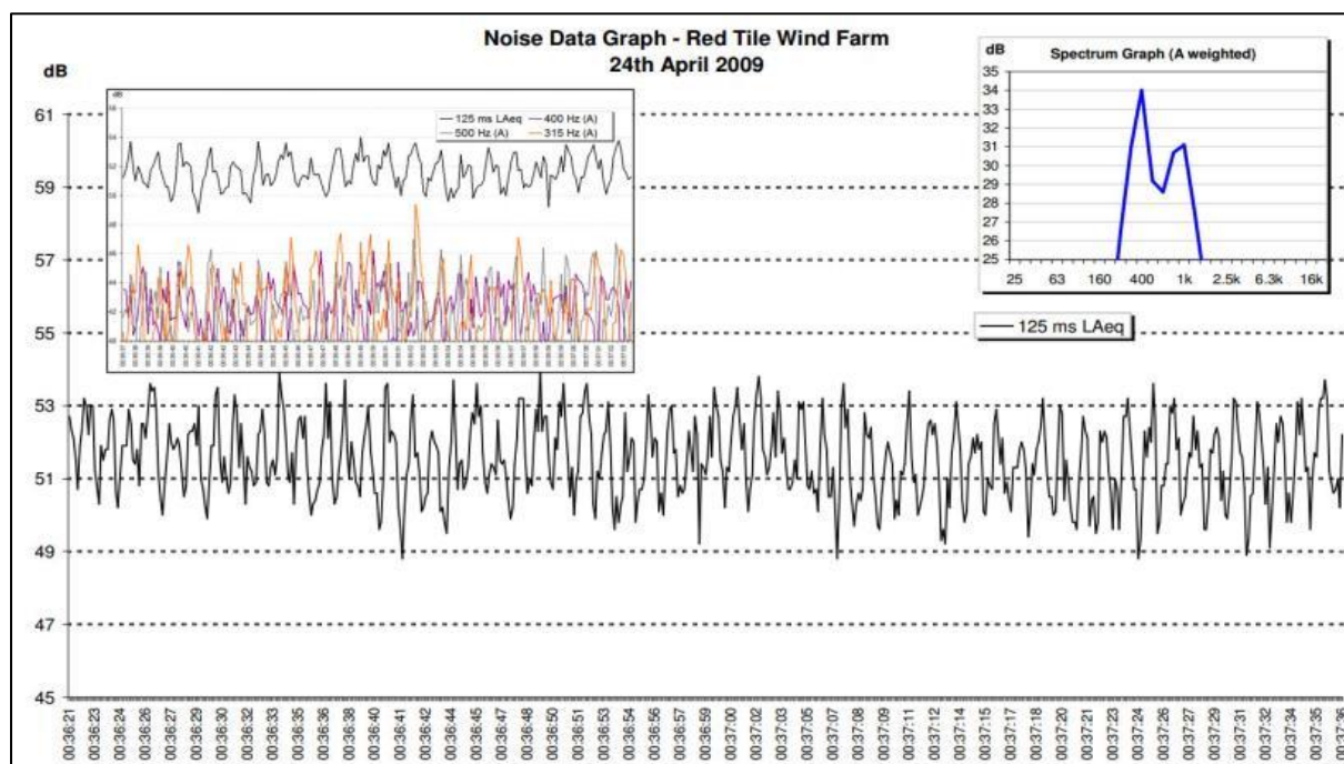
Figure 39: Example time-sound series graph illustrating AM as measured by Stigwood 18 (et al) (2013)
