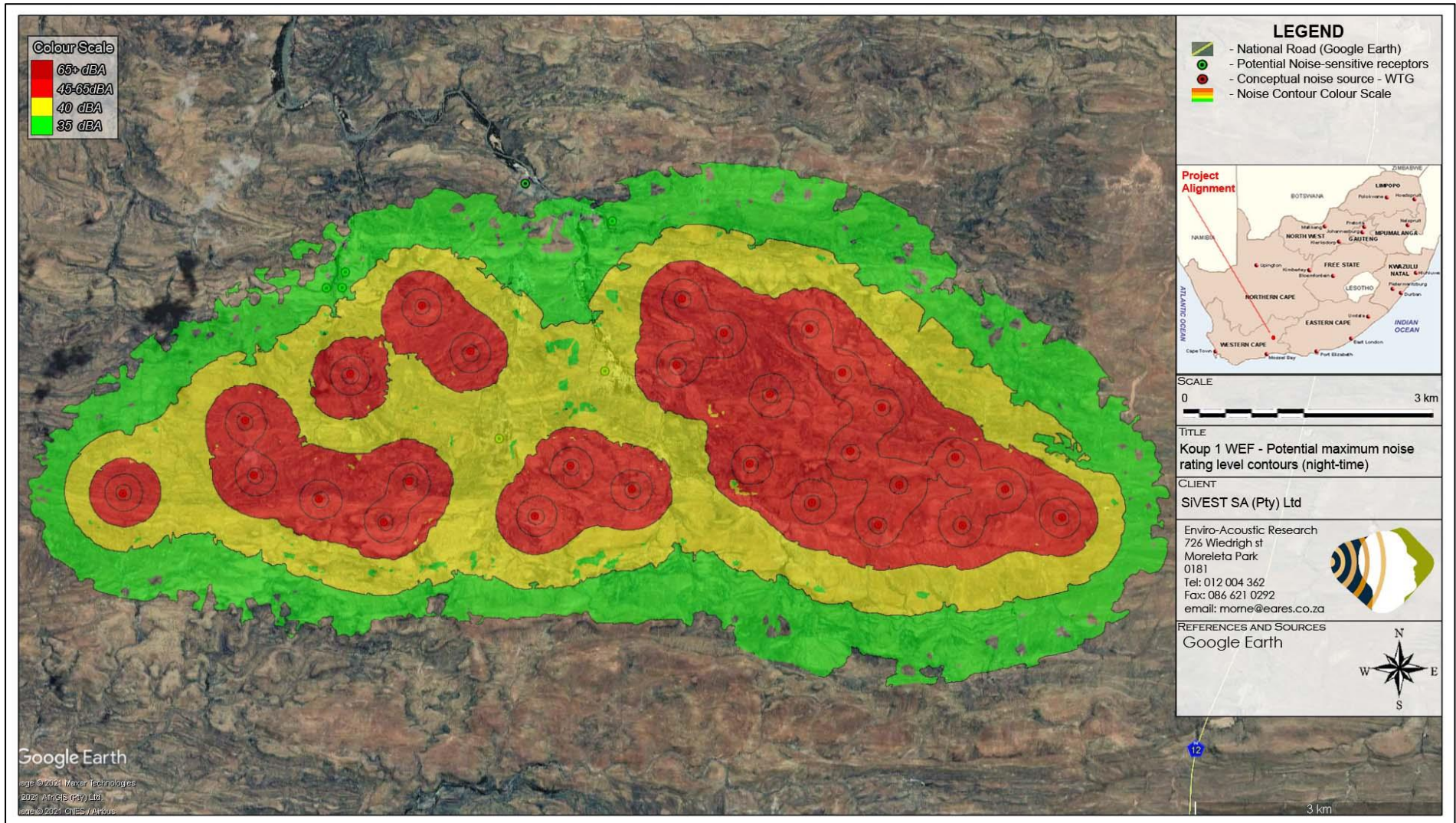
Figure 46: Projected maximum night-time operational noise rating levels due to the operation of Koup 1 WEF
