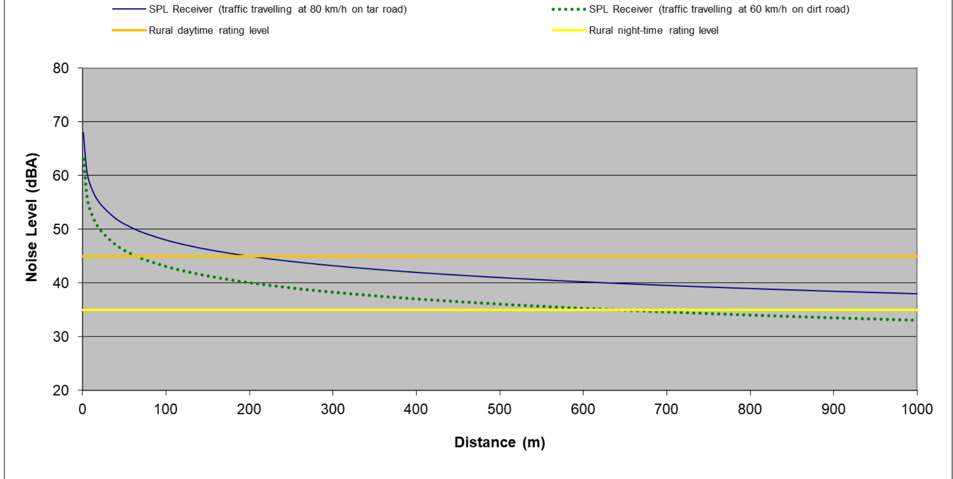
Figure 45: Projected conceptual construction noise levels – Decay over distance from linear activities
