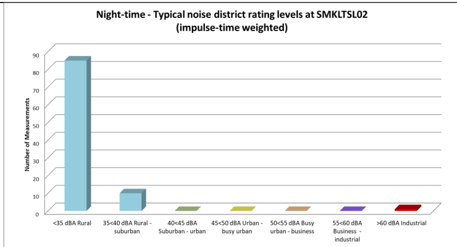
Figure 25: Classification of night-time measurements in typical noise districts at SMKLTSL02
