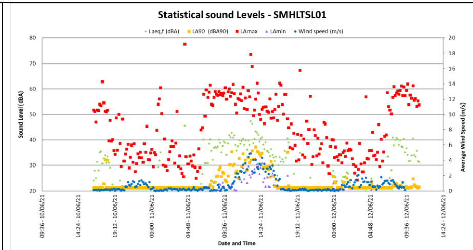
Figure 28: Maximum, minimum and Statistical sound levels at SMHLTSL01
