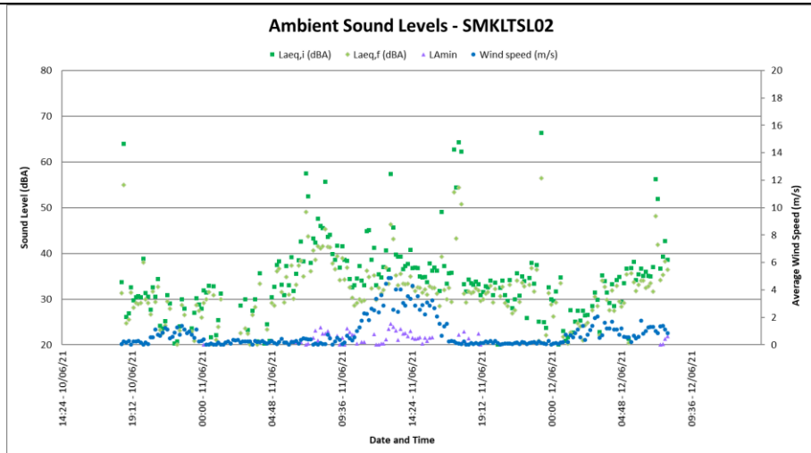
Figure 23: Residual noise Levels at SMKLTSL02
