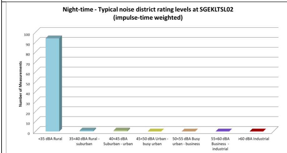
Figure 13: Classification of night-time measurements in typical noise districts at SGEKLTSL02
