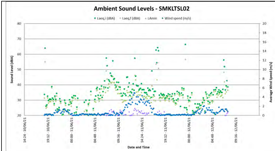
Figure 23: Residual noise Levels at SMKLTSLO2
