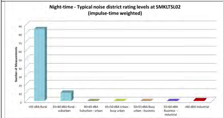
Figure 25: Classification of night-time measurements in typical noise districts at SMKLTSLO2
