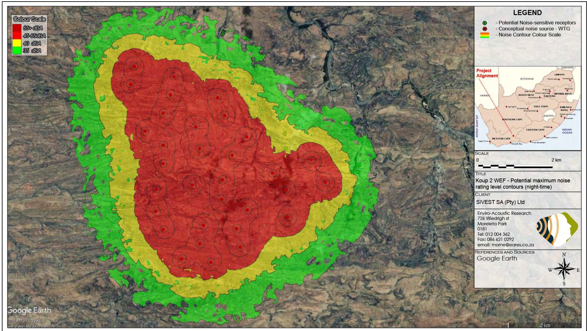
Figure 46: Projected maximum night-time operational noise rating levels due to the operation of Koup 2 WEF
