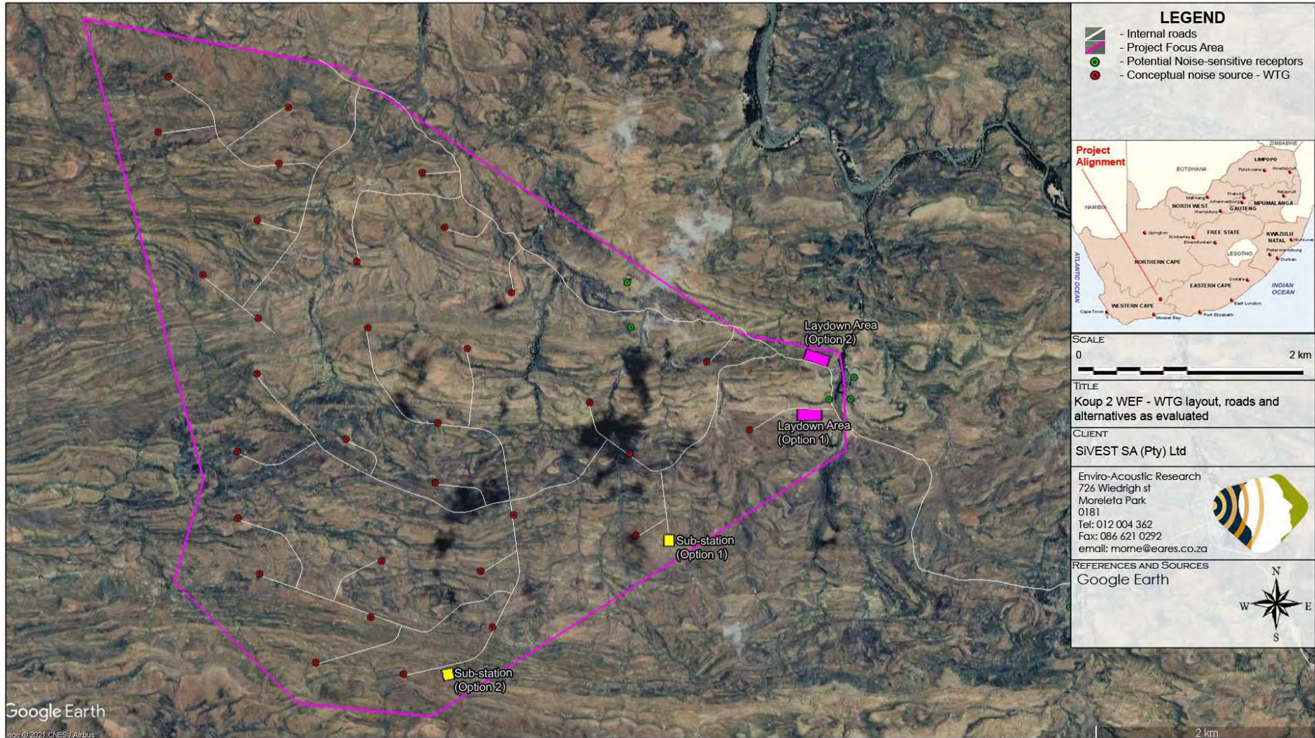
Figure 43: Proposed WTG Layout of the Koup 2 WEF
