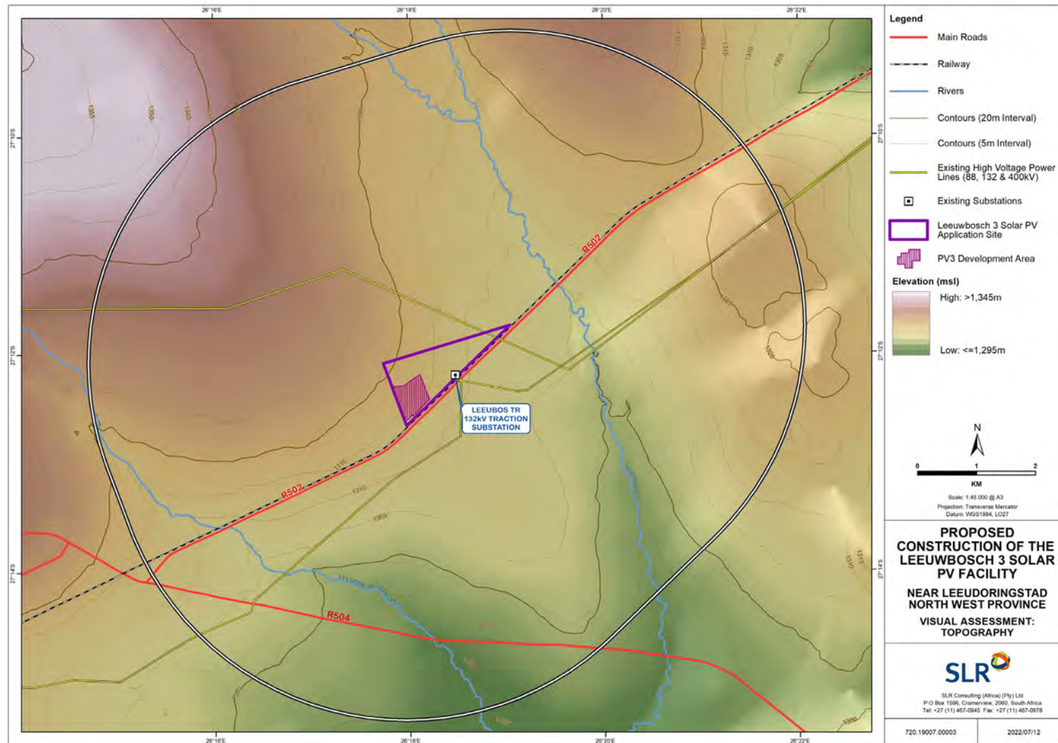
Figure 5: Topography in the Study Area
