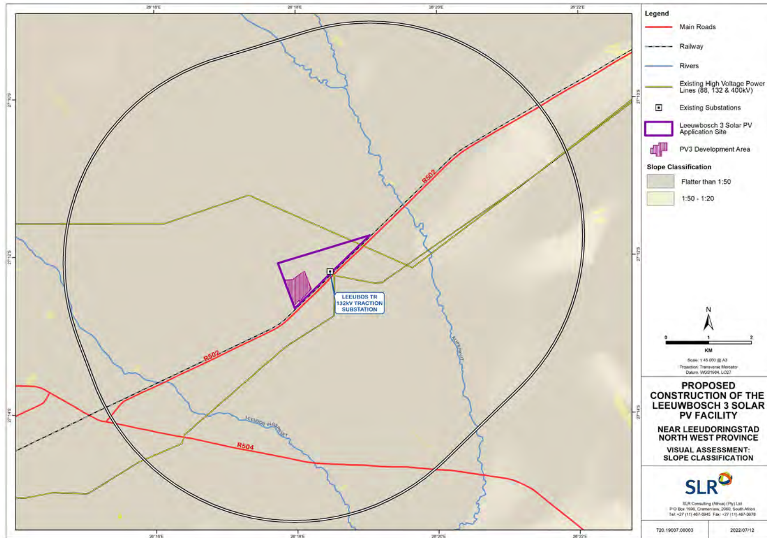
Figure 6: Slope Classification in the Study Area
