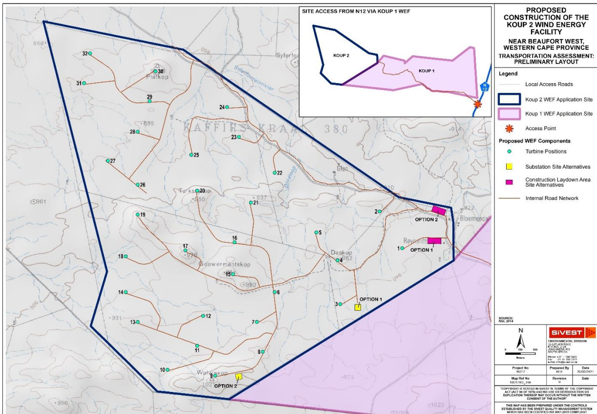
Figure 8.2 Koups 2 WEF – Preliminary Internal Layout
