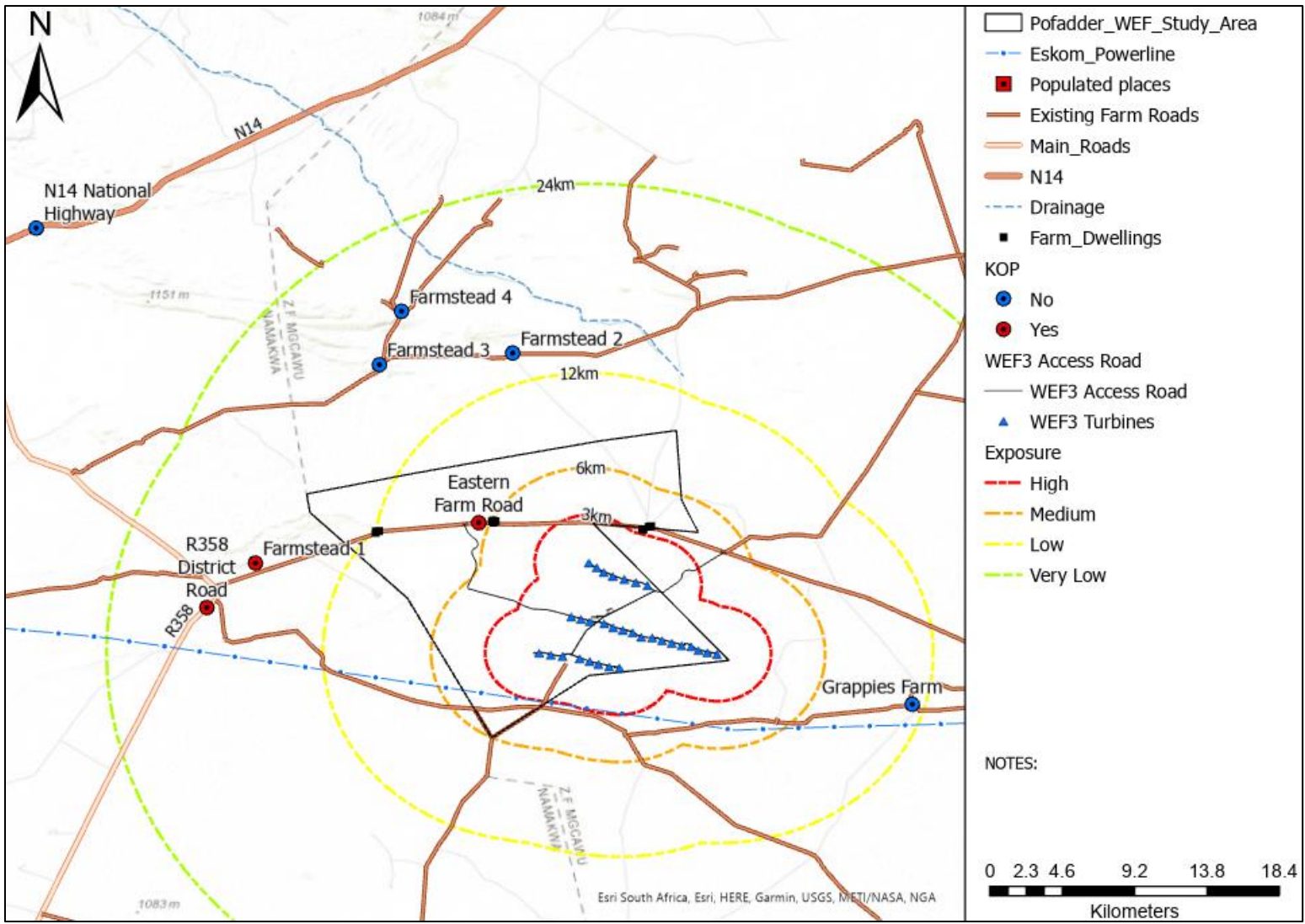
Figure 17: WEF3 preliminary Receptor and KOP locality map.
