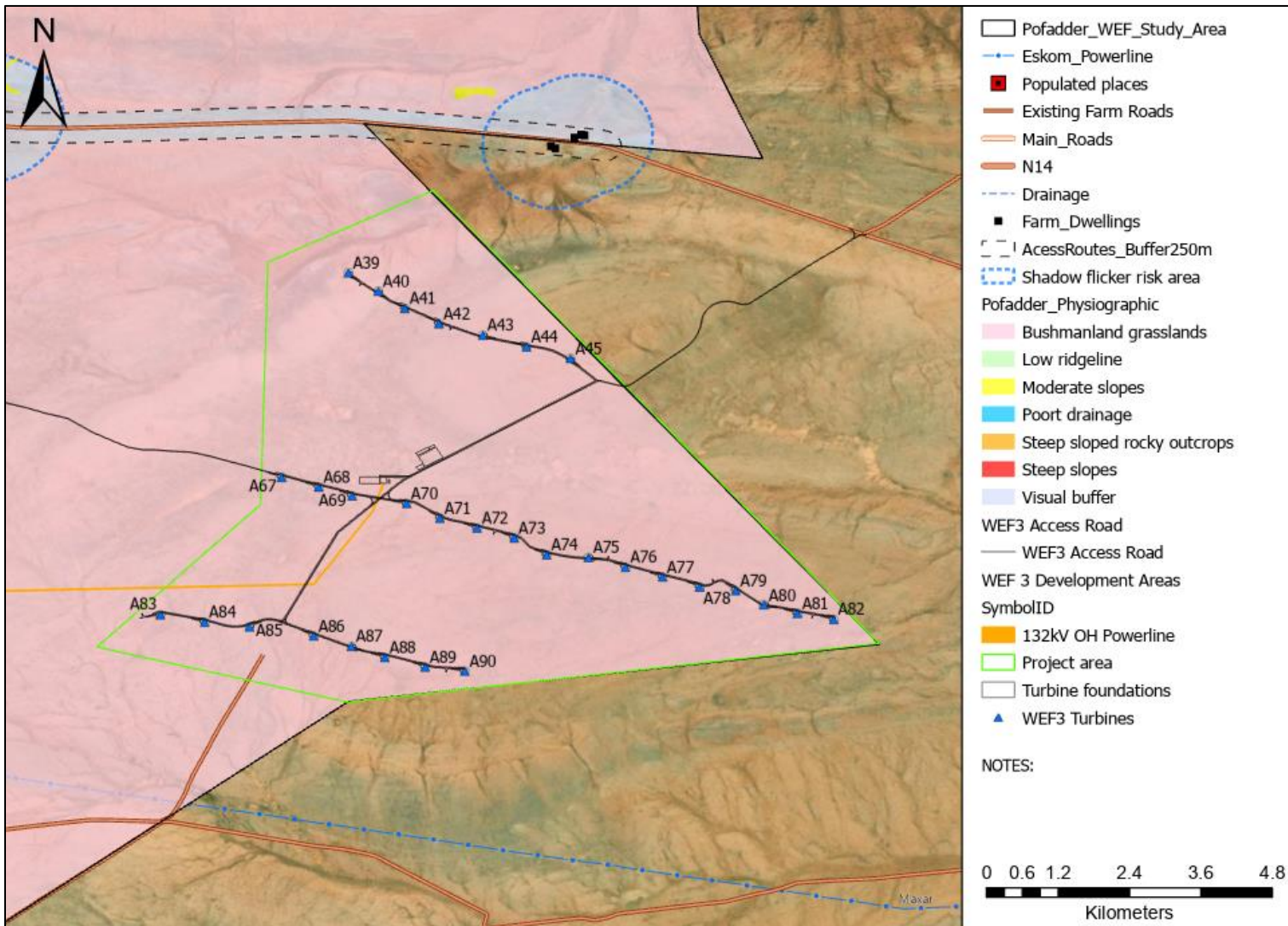
Figure 18: WEF3 site Satellite Image Map depicting uniform terrain and vegetation.
