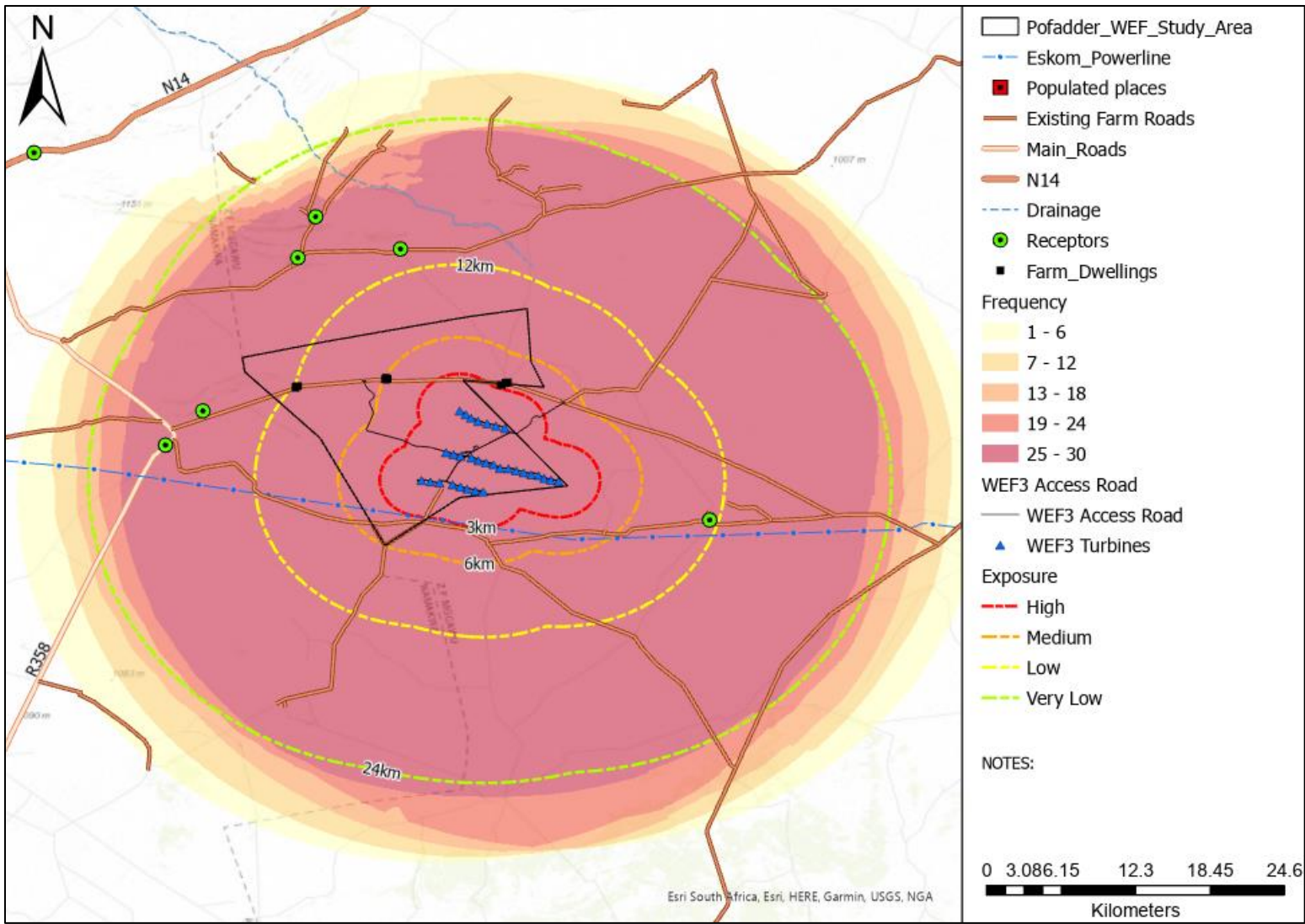
Figure 15. Expected WEF3 project viewshed and exposure generated from 300m height above ground from turbine points.
