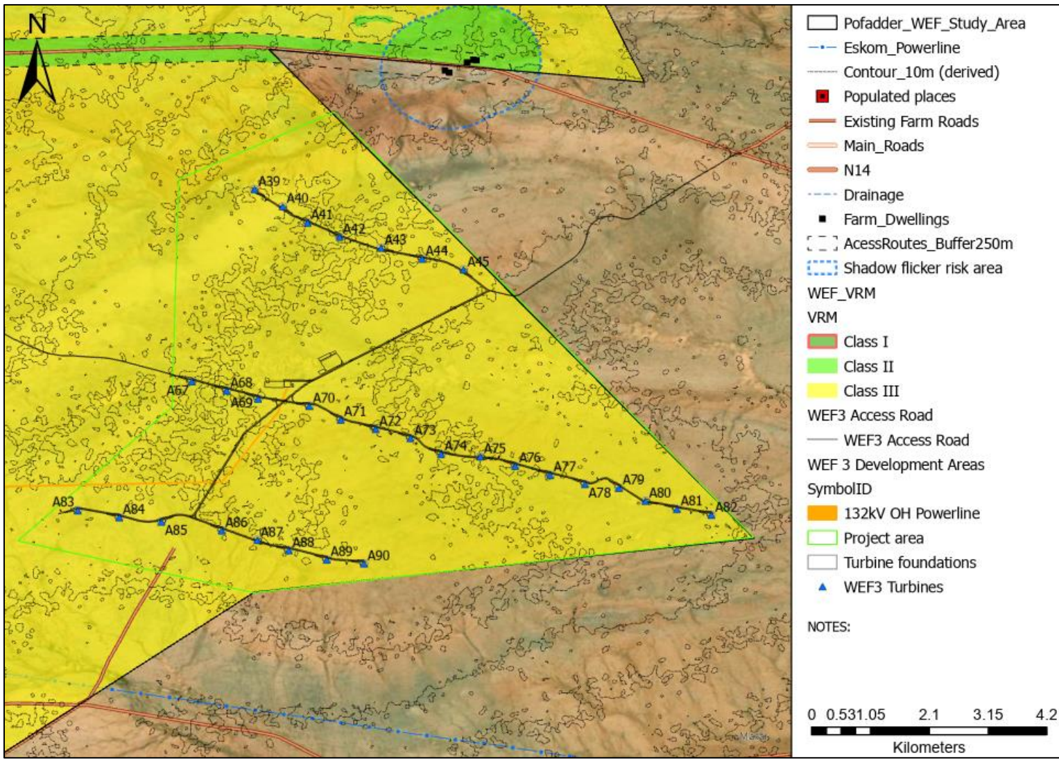
Figure 19: WEF3 VRM Class overlay onto satellite imagery.
