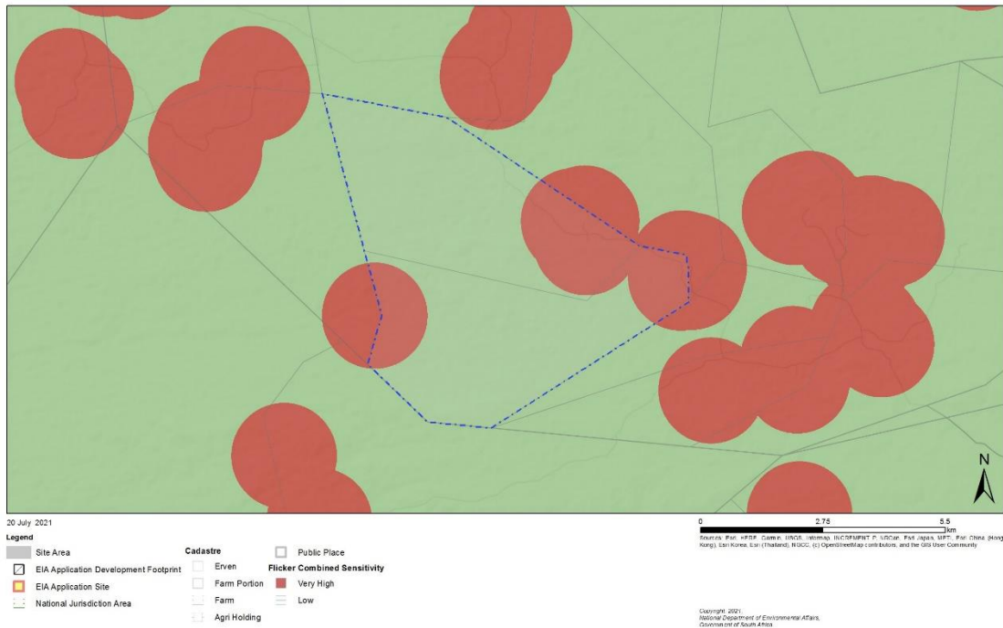
Figure 30: Flicker Sensitivity (July 2021)
