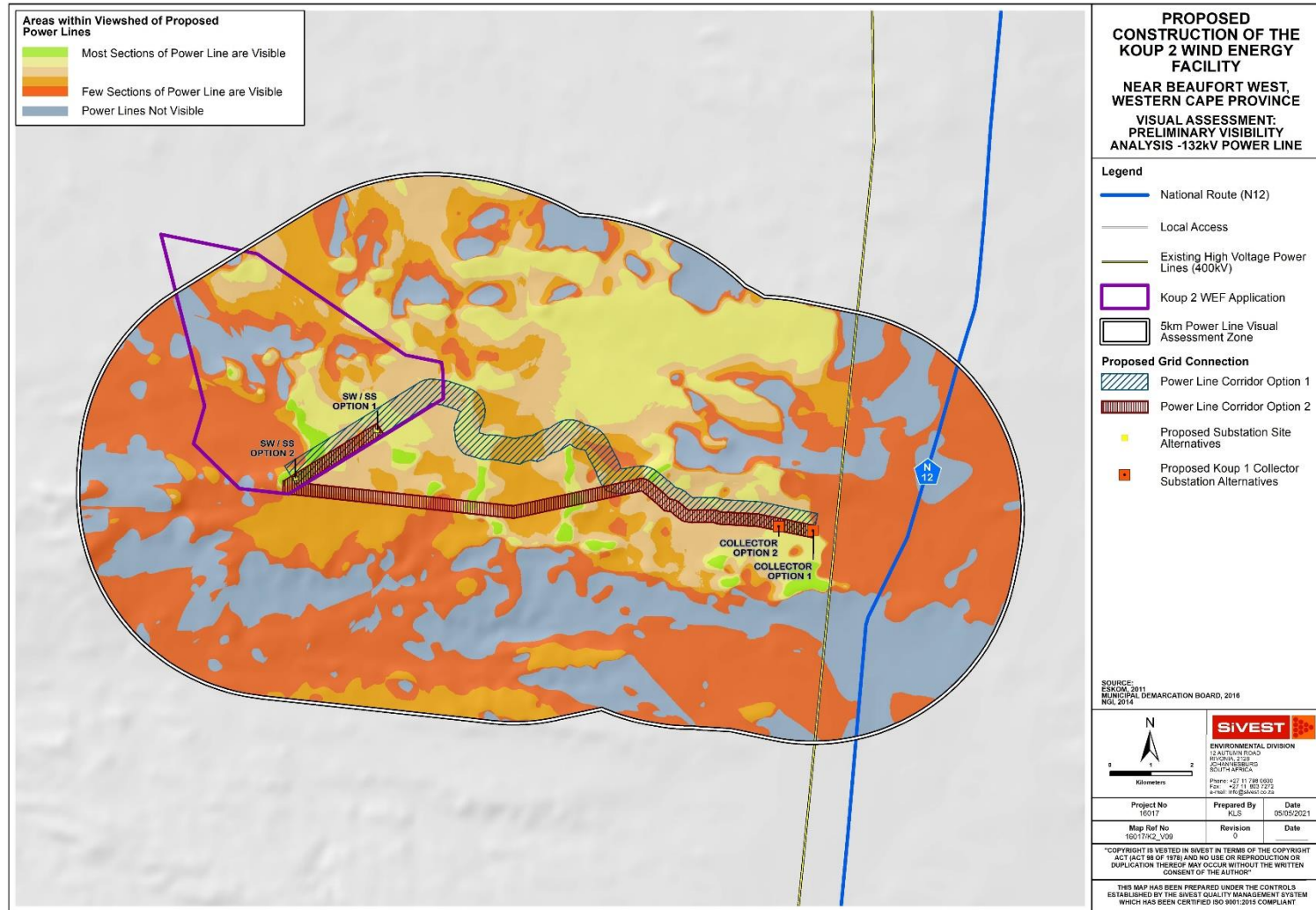
Figure 16: Potential Visibility of Power Lines
