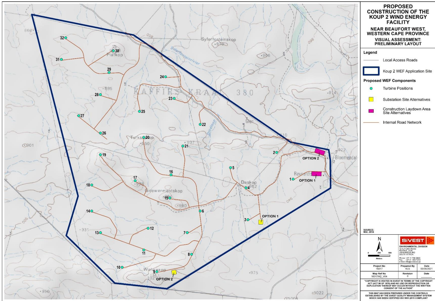
Figure 6: Preliminary Koup 2 WEF layout
