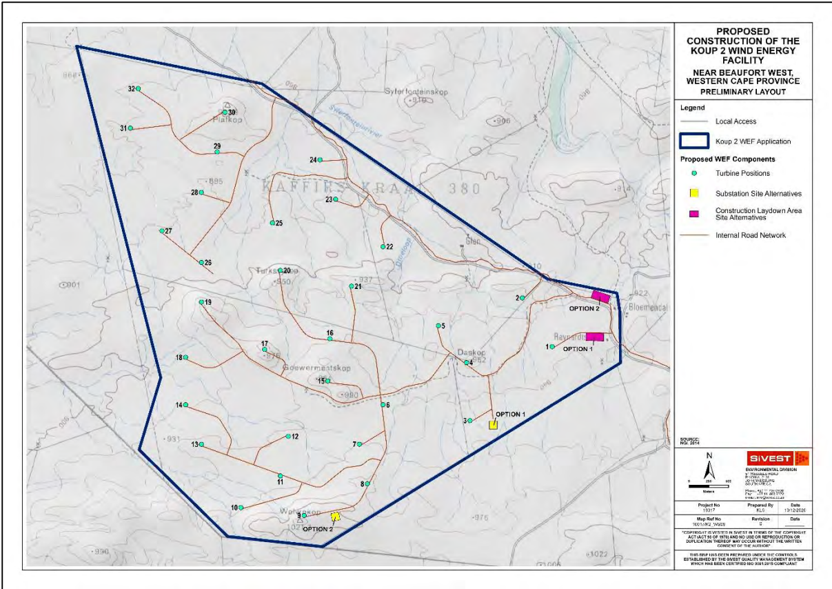
Figure 4: Preliminary Layout
