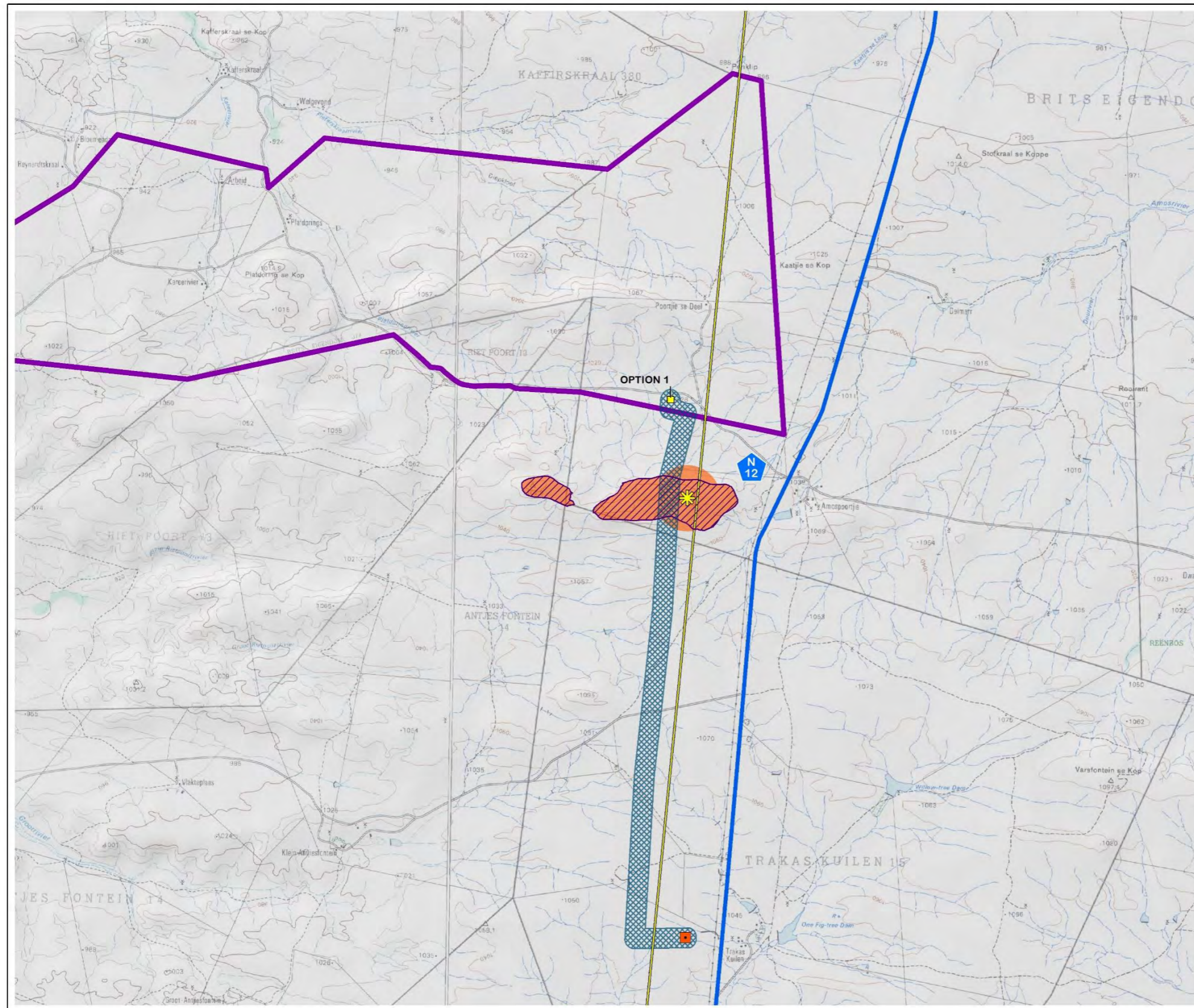
MAP 20: Preferred Grid Connection Alternatives for Koup 1 WEF
