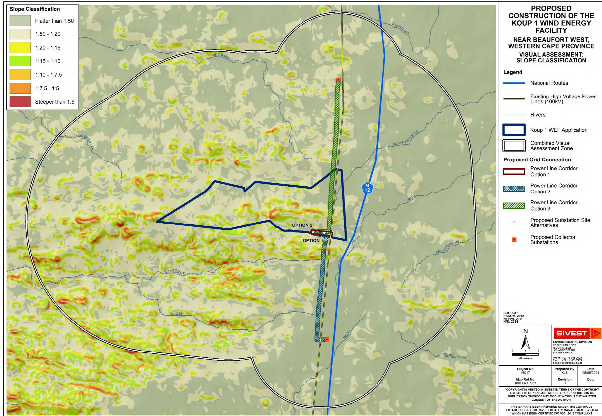
MAP 7: Slope Classification
