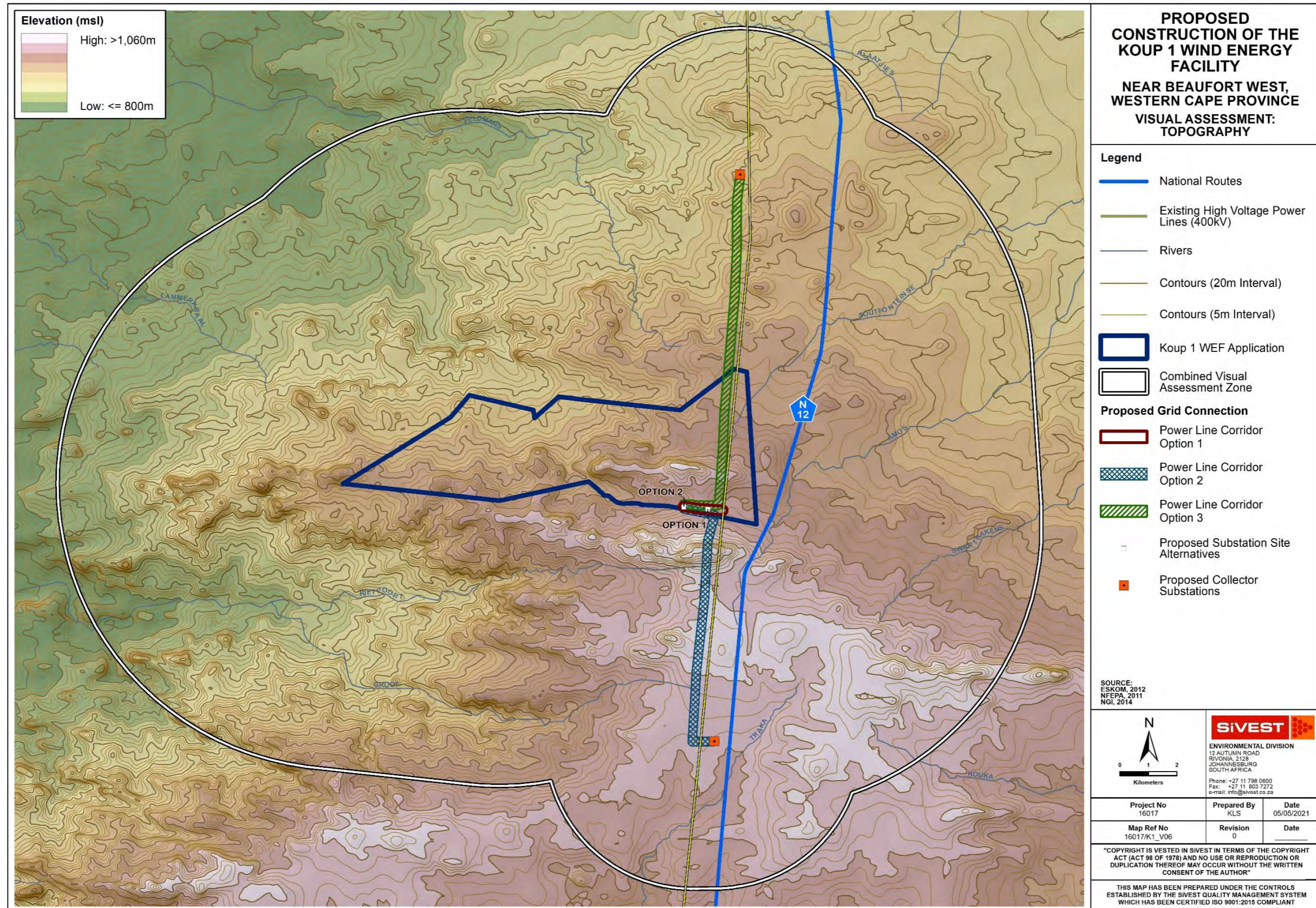
MAP 6: Topography
