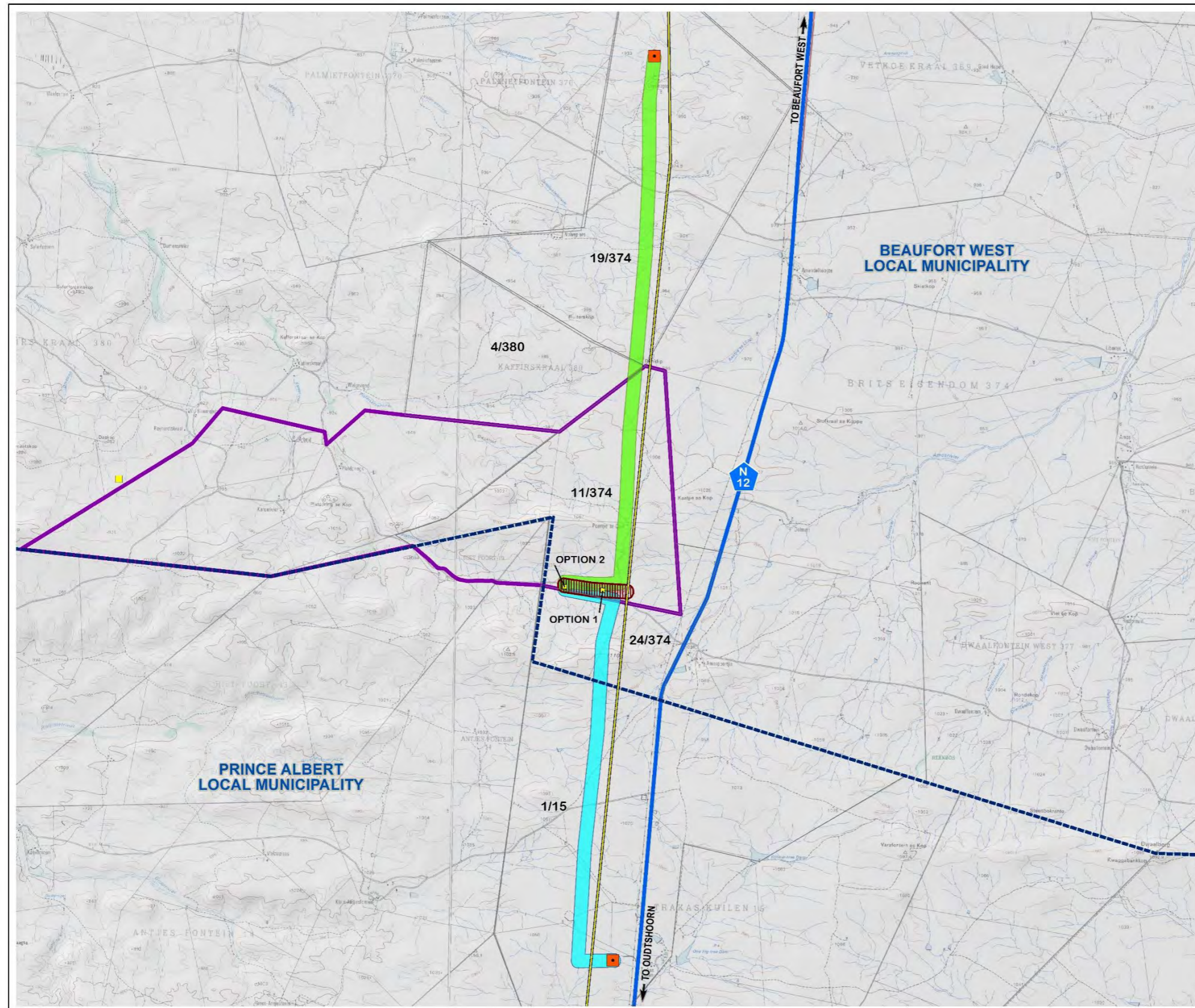
MAP 5: Grid Connection Alternatives
