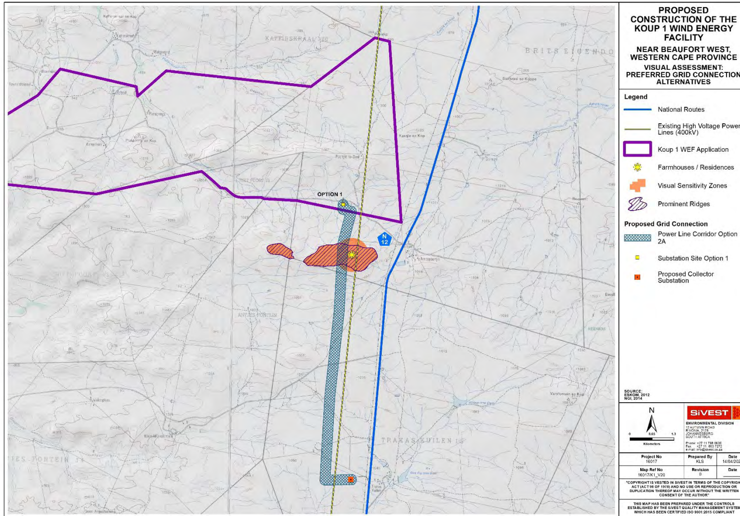
Figure 44: Preferred Grid Connection Alternatives for Koups 1 WEF
