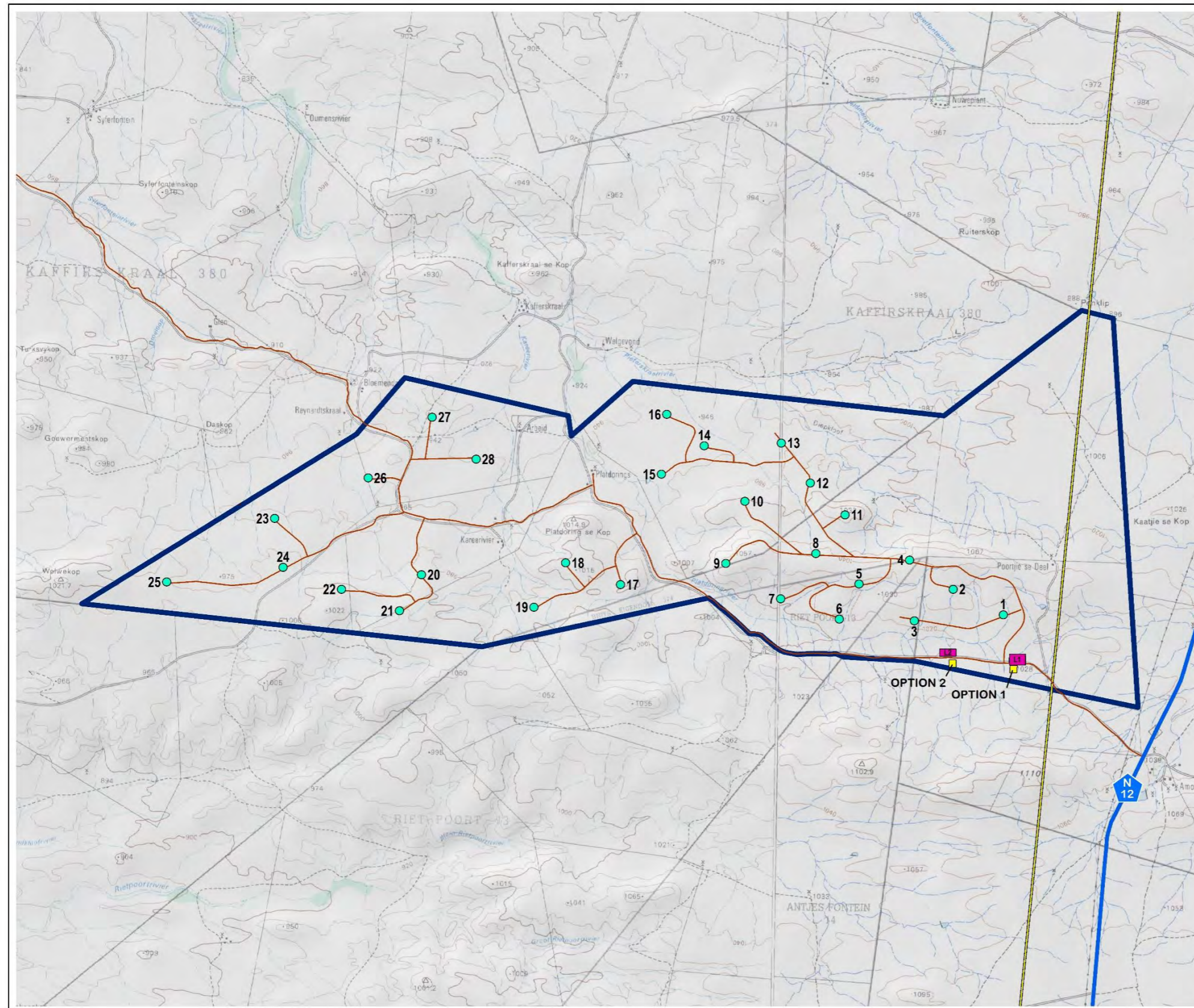
MAP 4: Preliminary WEF Layout
