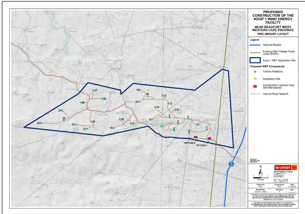
Figure 4: Preliminary Layout
