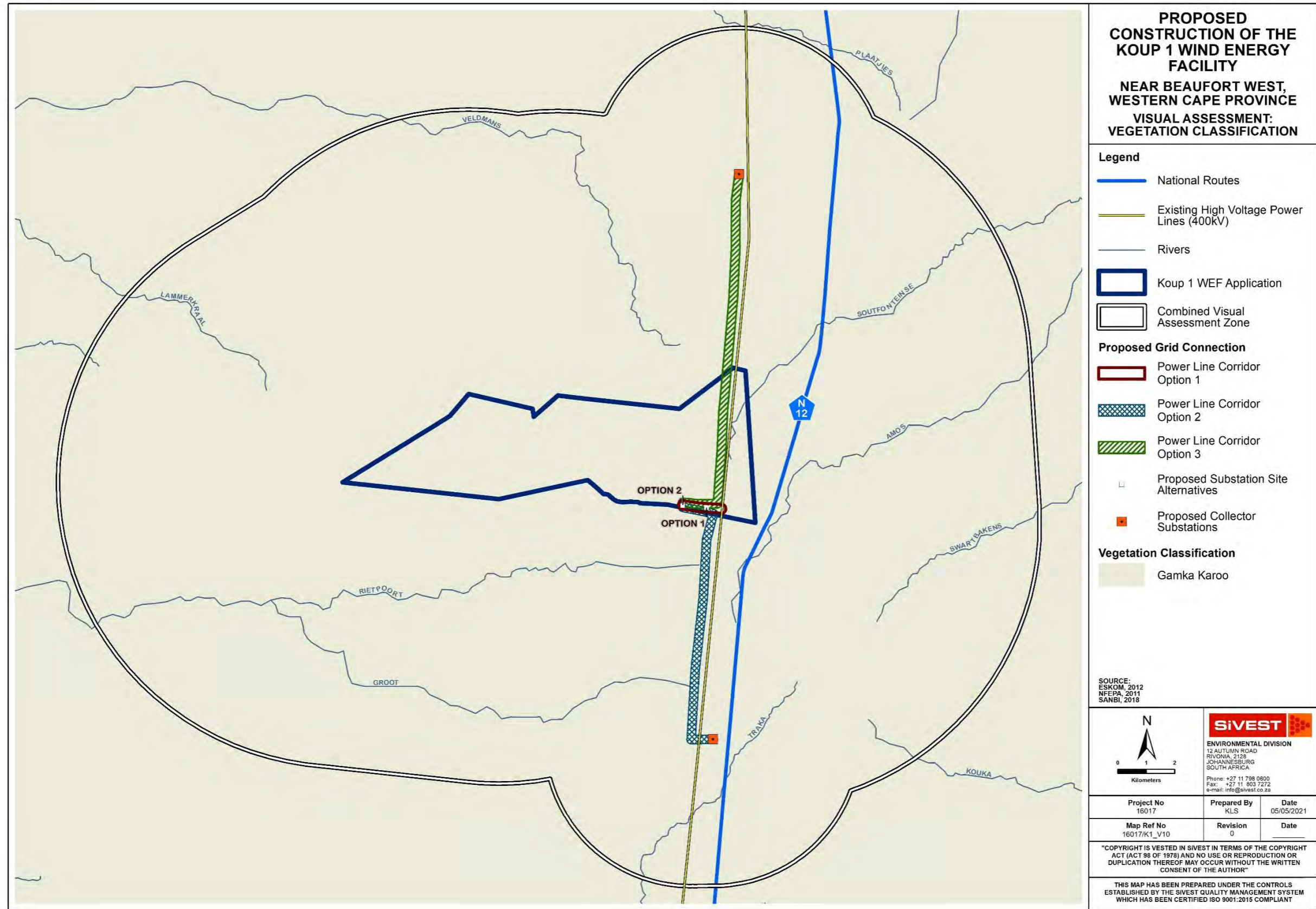
MAP 10: Vegetation Classification
