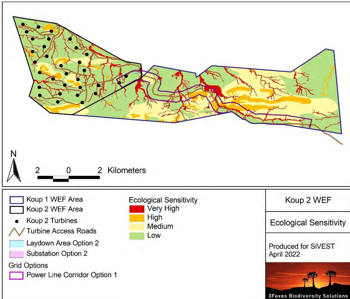
Figure 16. Sensitivity map for the Koups 2 site, showing the 32-turbine layout provided for the assessment as well as the grid connection alternatives.
