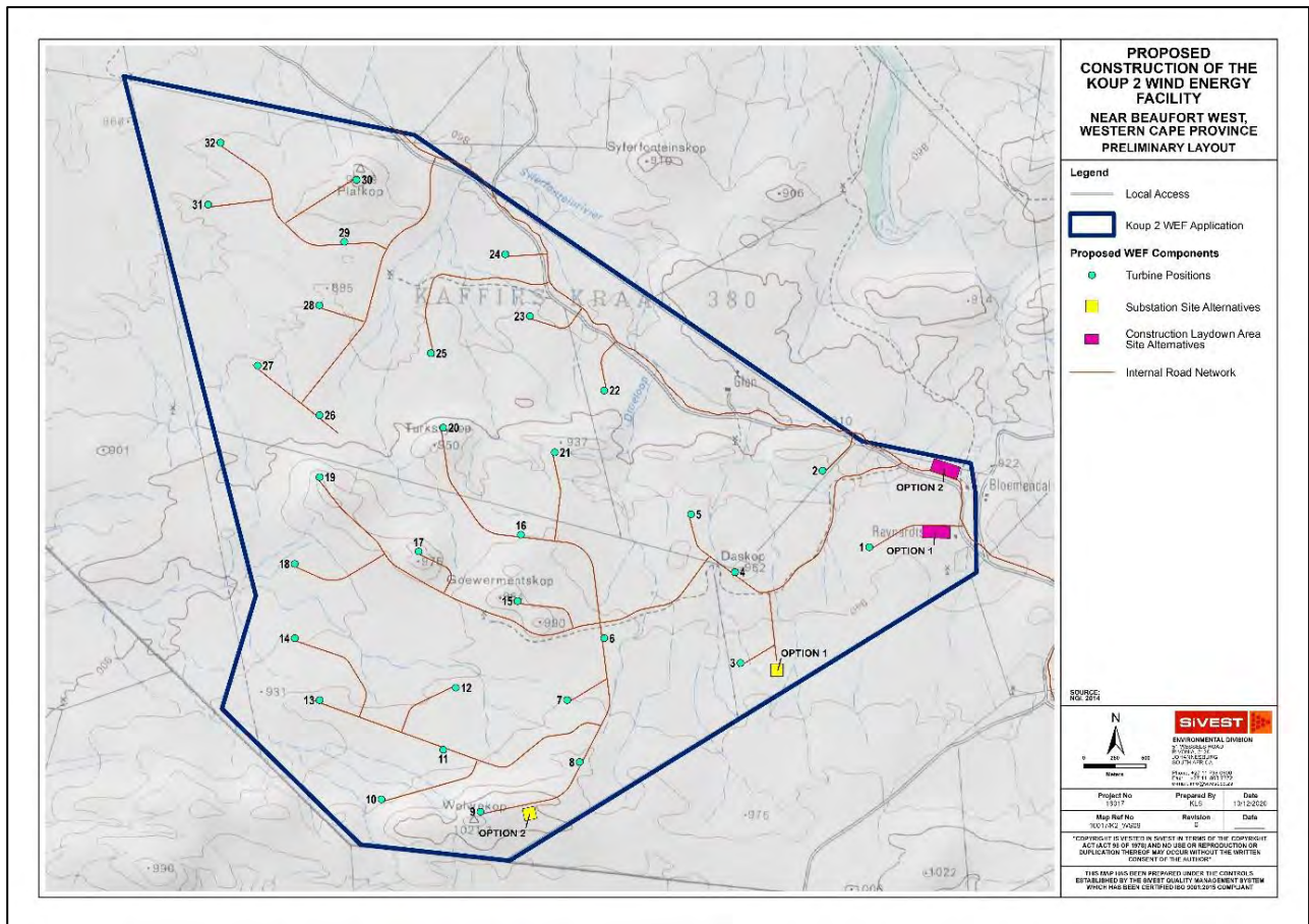
Figure 4: Alternatives proposed as part of the Koup 2 WEF. In the final assessment, Laydown Area Option 2 and Substation Option 2 have been selected as the preferred options for approval.
