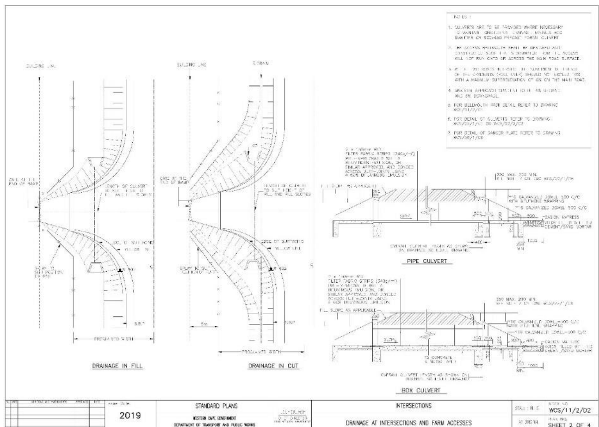
Figure 7.12 Typical Drainage at Intersections and Farm Access
