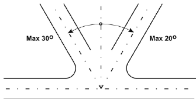
Figure 7.13 Angle of intersection deviation
