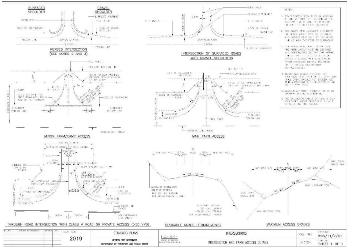
Figure 7.10 Typical Intersection and Farm Access Detail
