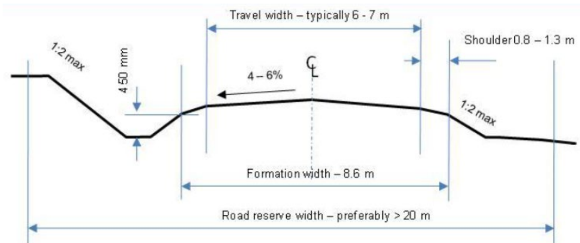
Figure 7.12 Typical Provincial Gravel Road Cross Section
