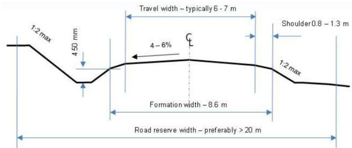
Figure 7.13 Typical Provincial Gravel Road Cross Section
