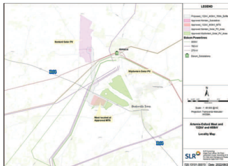
Figure 1: Radio Mast and 132kV and 400kV Infrastructure Locality
