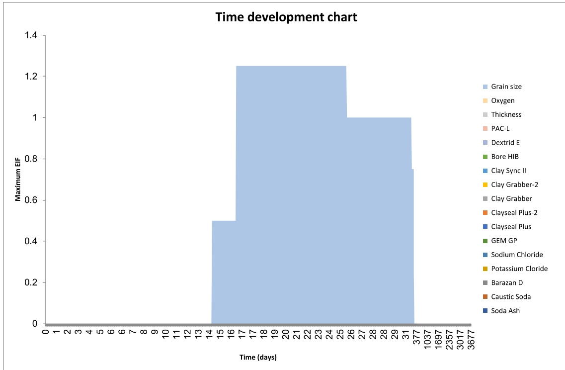
Figure 8.11 Time development of EIF for the sediment for discharges from the rig, location 4 – Summer.
