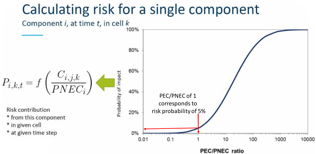
Figure 2.4 Relation between the PEC/PNEC ratio and the risk probability (in %) as presented by Karman et. Al. (1994) and further described in Karman and Reerink (1997). PEC/PNEC = 1 corresponds to a 5% risk probability (5% of the species are exposed above their chronic NOEC).
