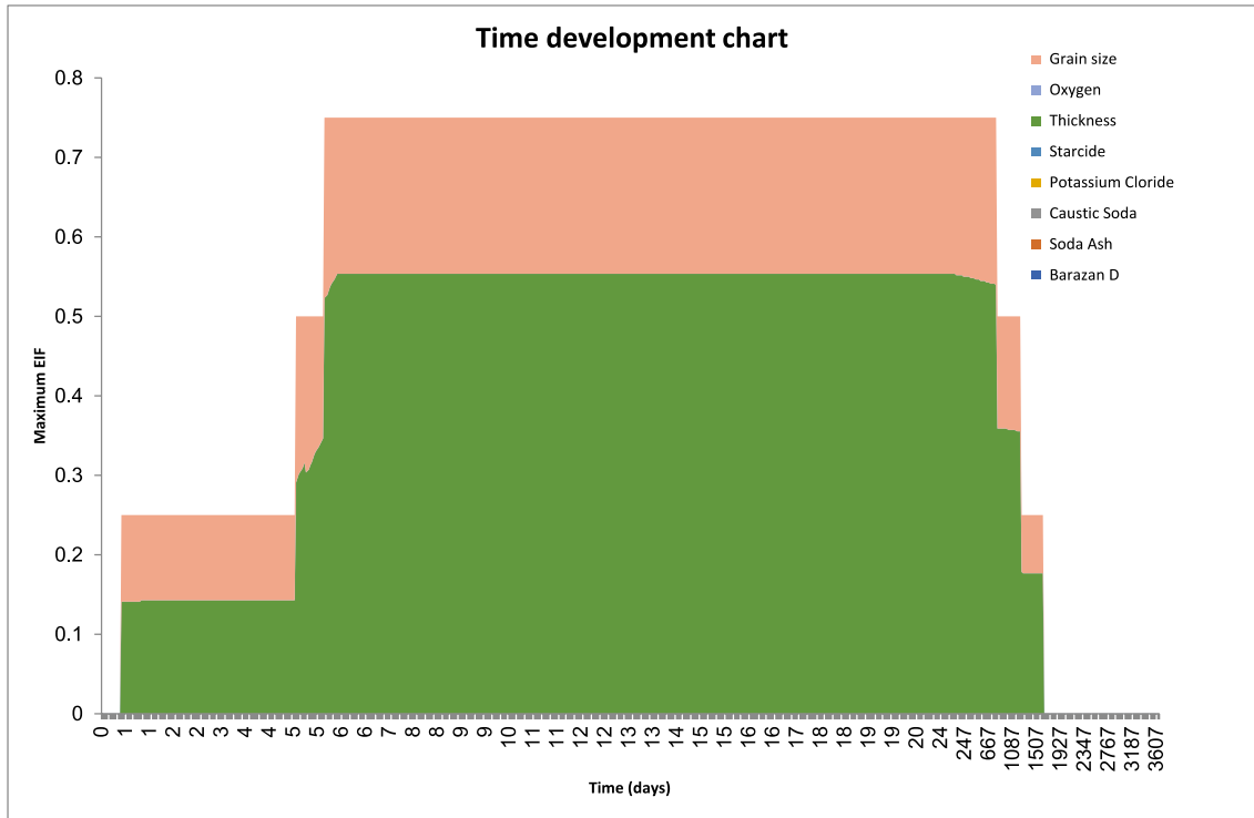
Figure 8.21 Time development of EIF for discharge from the top hole sections for the sediment for discharge location 4 – Autumn.
