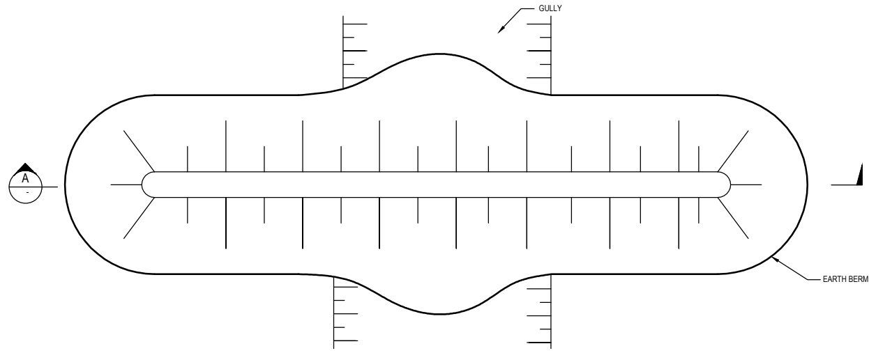
TYPICAL PLAN VIEW OF BERM
